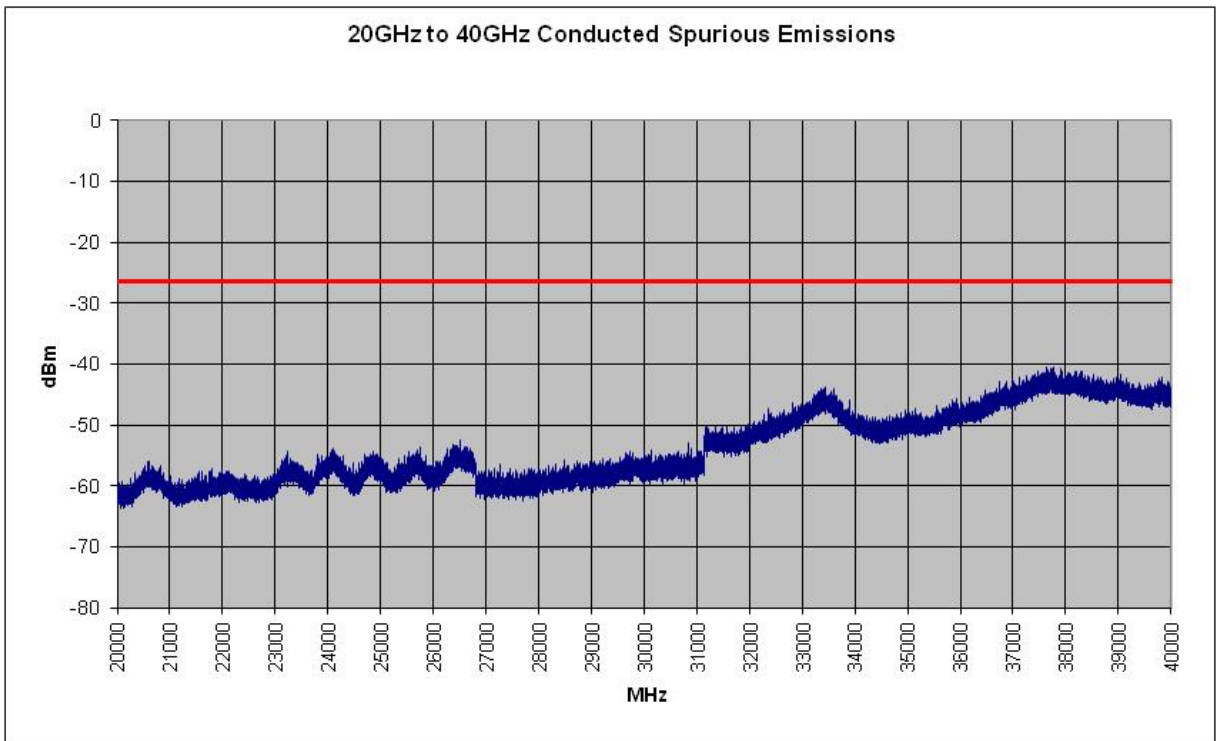
Plot 6-60. Conducted Spurious Plot (802.11a – Ch. 157)
