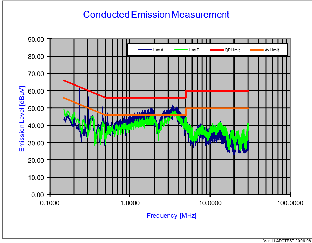
Plot 6-68. Line Conducted Plot with 802.11a
