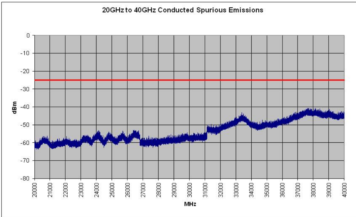
Plot 6-58. Conducted Spurious Plot (802.11a – Ch. 149)
