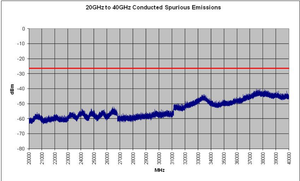
Plot 6-62. Conducted Spurious Plot (802.11a – Ch. 165)
