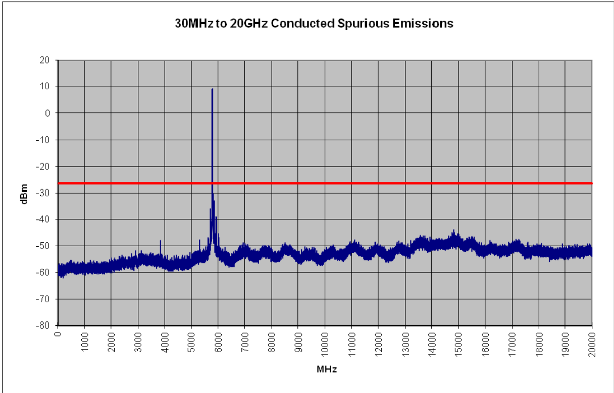
Plot 6-59. Conducted Spurious Plot (802.11a – Ch. 157)
