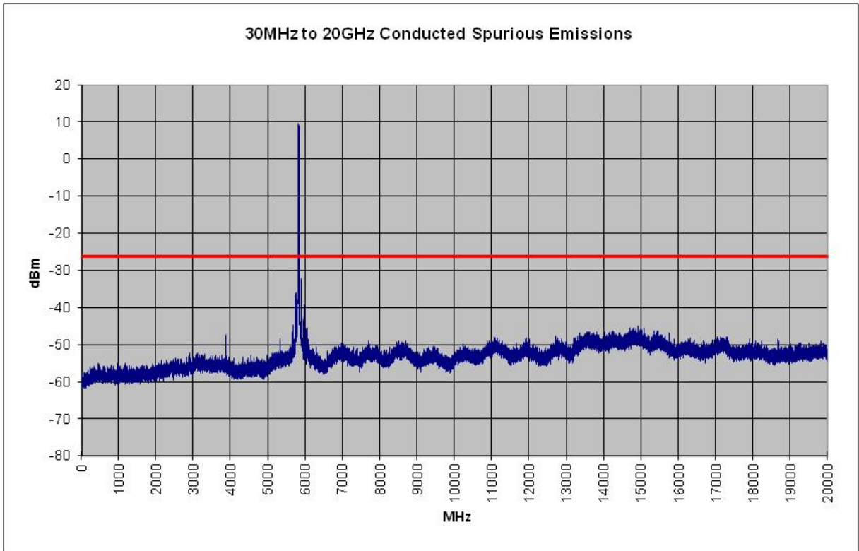
Plot 6-61. Conducted Spurious Plot (802.11a – Ch. 165)
