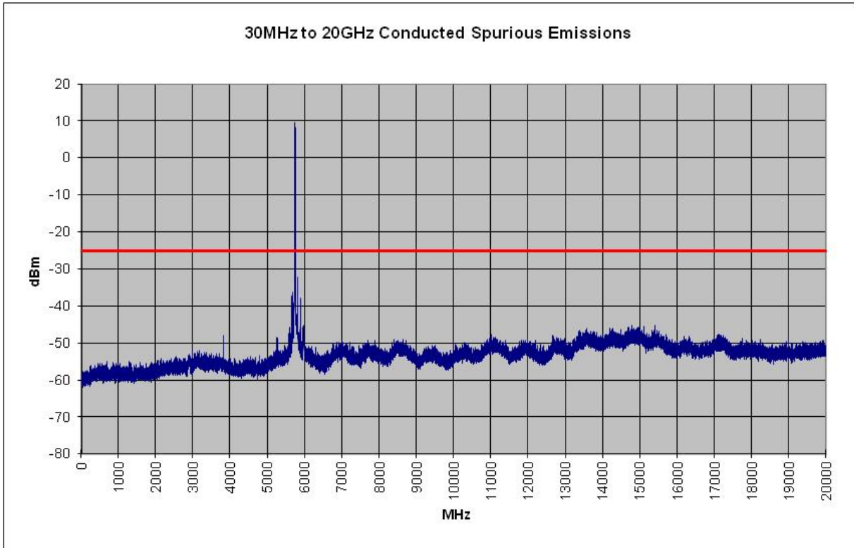
Plot 6-57. Conducted Spurious Plot (802.11a – Ch. 149)
