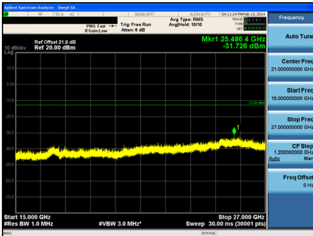
Conducted Spurious Plot_2 (Low ch_20 MHz_QPSK_RB 1_0)
