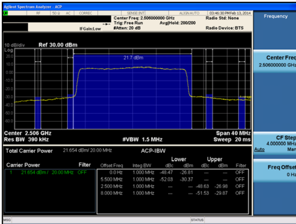
Channel Edge Plot (20MHz QPSK - RB Size 100 – Low Ch.)
