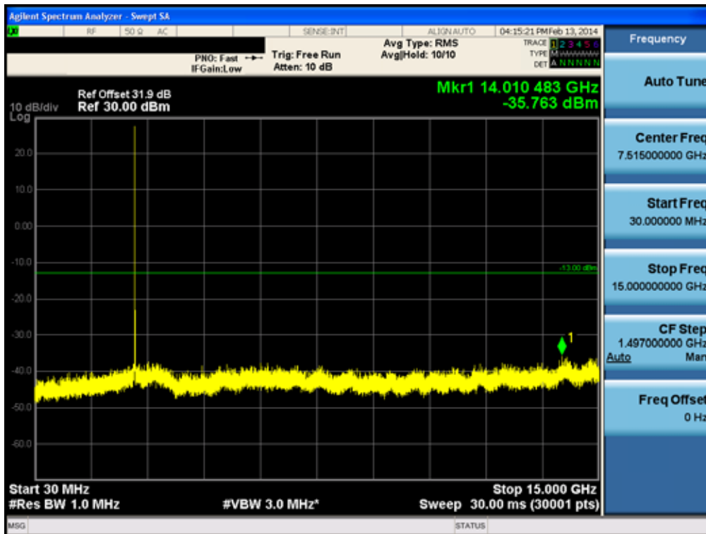
Conducted Spurious Plot_1 (High ch_15 MHz_QPSK_RB 1_0)
