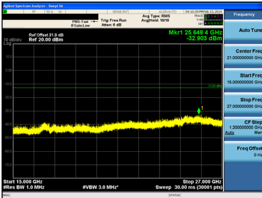
Conducted Spurious Plot_2 (High ch_15 MHz_QPSK_RB 1_0)
