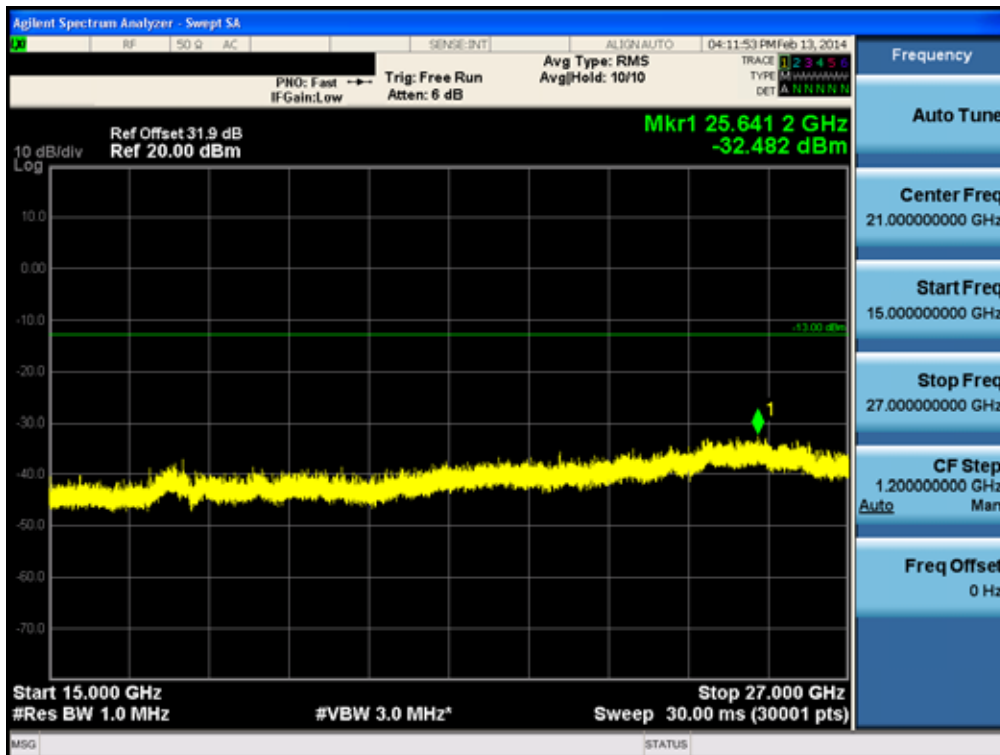
Conducted Spurious Plot_2 (Mid ch_20 MHz_QPSK_RB 1_0)
