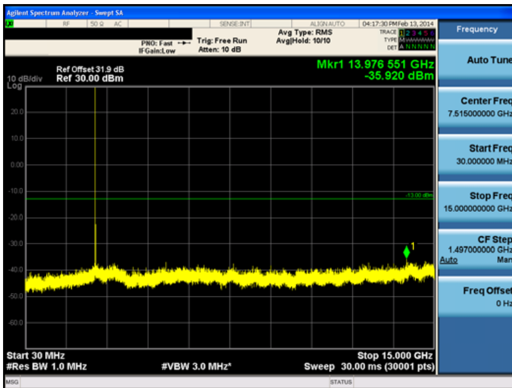
Conducted Spurious Plot_1 (Mid ch_10 MHz_QPSK_RB 1_0)
