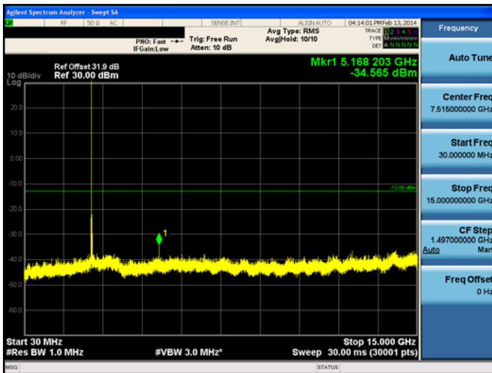
Conducted Spurious Plot_1 (Mid ch_20 MHz_QPSK_RB 1_0)
