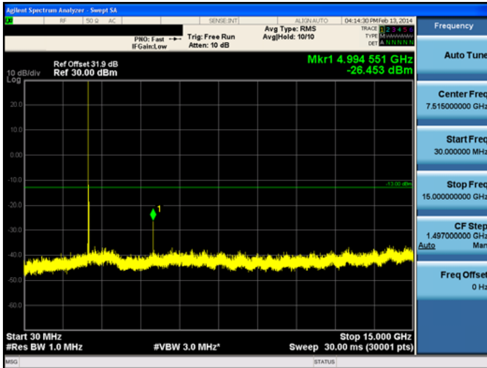
Conducted Spurious Plot_1 (Low ch_20 MHz_QPSK_RB 1_0)
