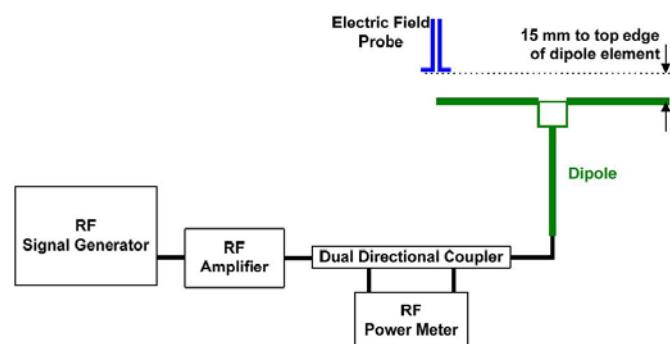
Setup diagram
