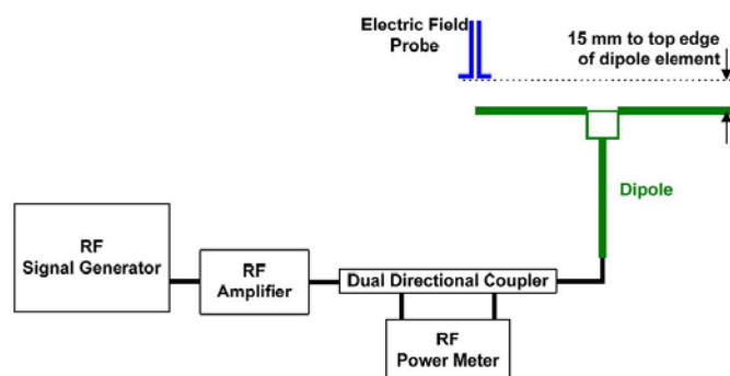
Setup diagram
