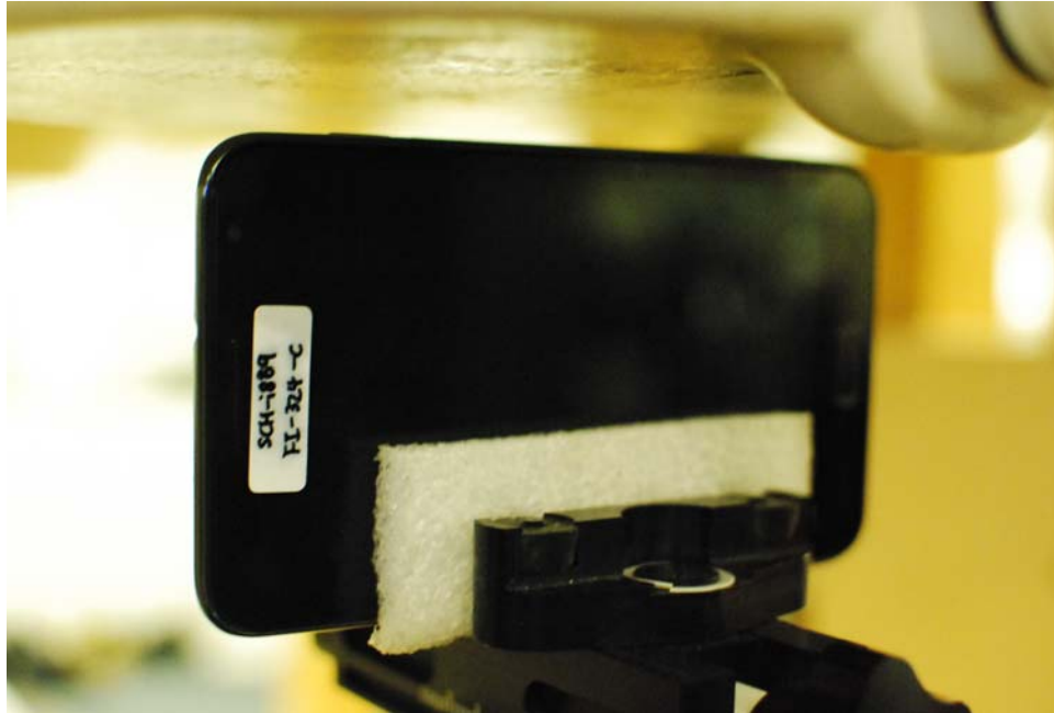
SAR Test Setup Photo 9
