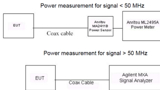
Figure 9-3 Power Measurement Setup
