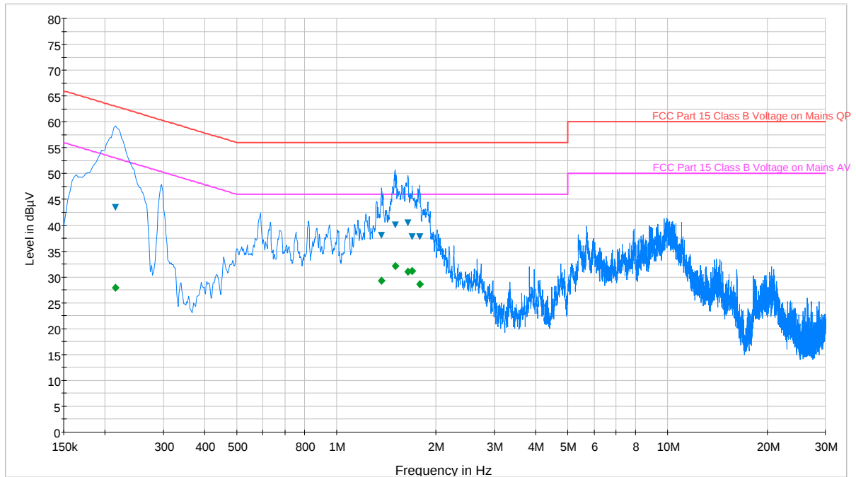
Plot 7-2. Line Conducted Plot (LN)
