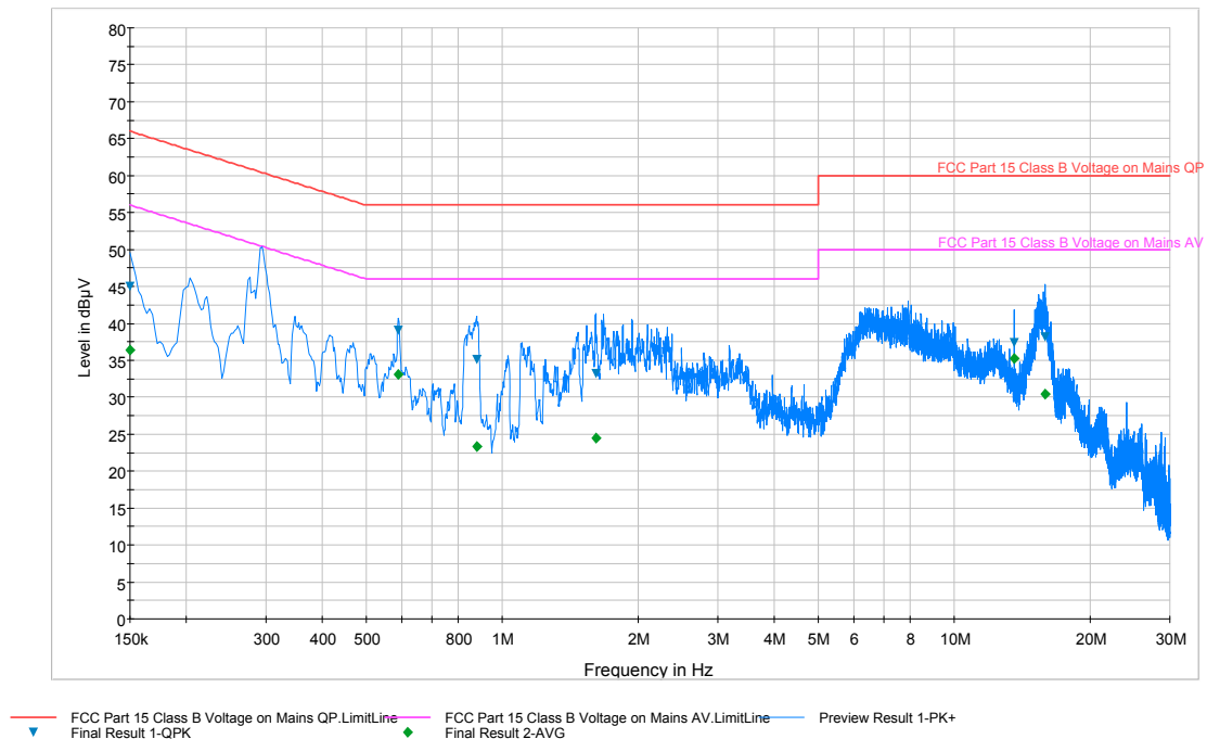
Plot 8-1. Line-Conducted Test Plot (L1)
