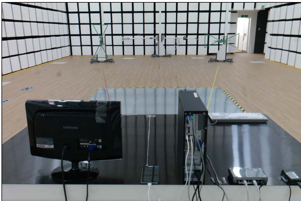
[ Radiated Disturbance for Below 1 GHz – Rear ]
