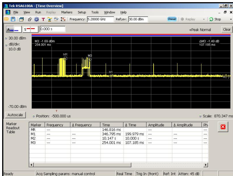
Figure 5-5. Move Time around M1
