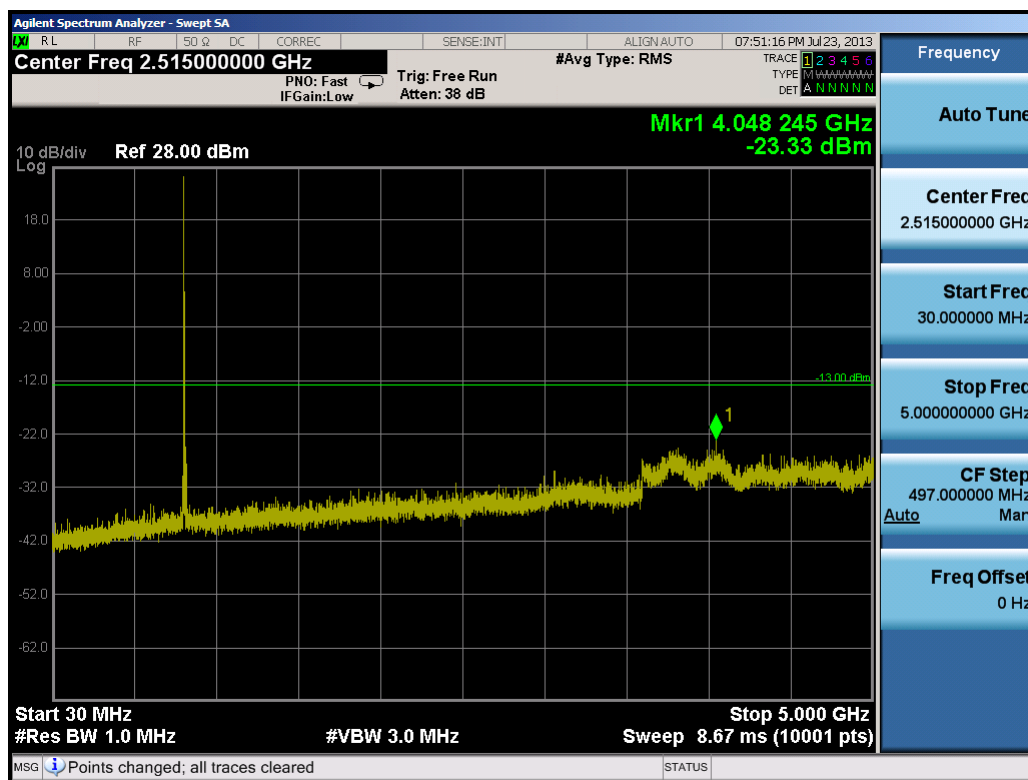
Plot 8-14. Conducted Spurious Plot (10.0MHz QPSK – RB Size 1, RB Offset 0– Low Channel)
