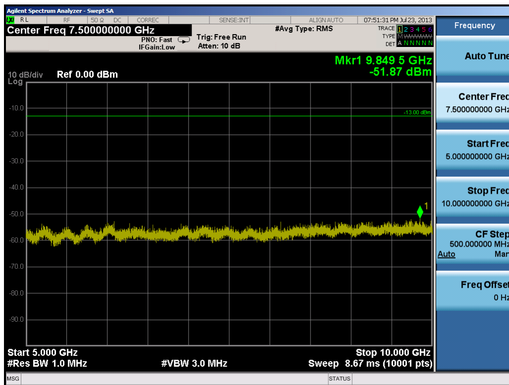
Plot 8-15. Conducted Spurious Plot (10.0MHz QPSK – RB Size 1, RB Offset 0 – Low Channel)
