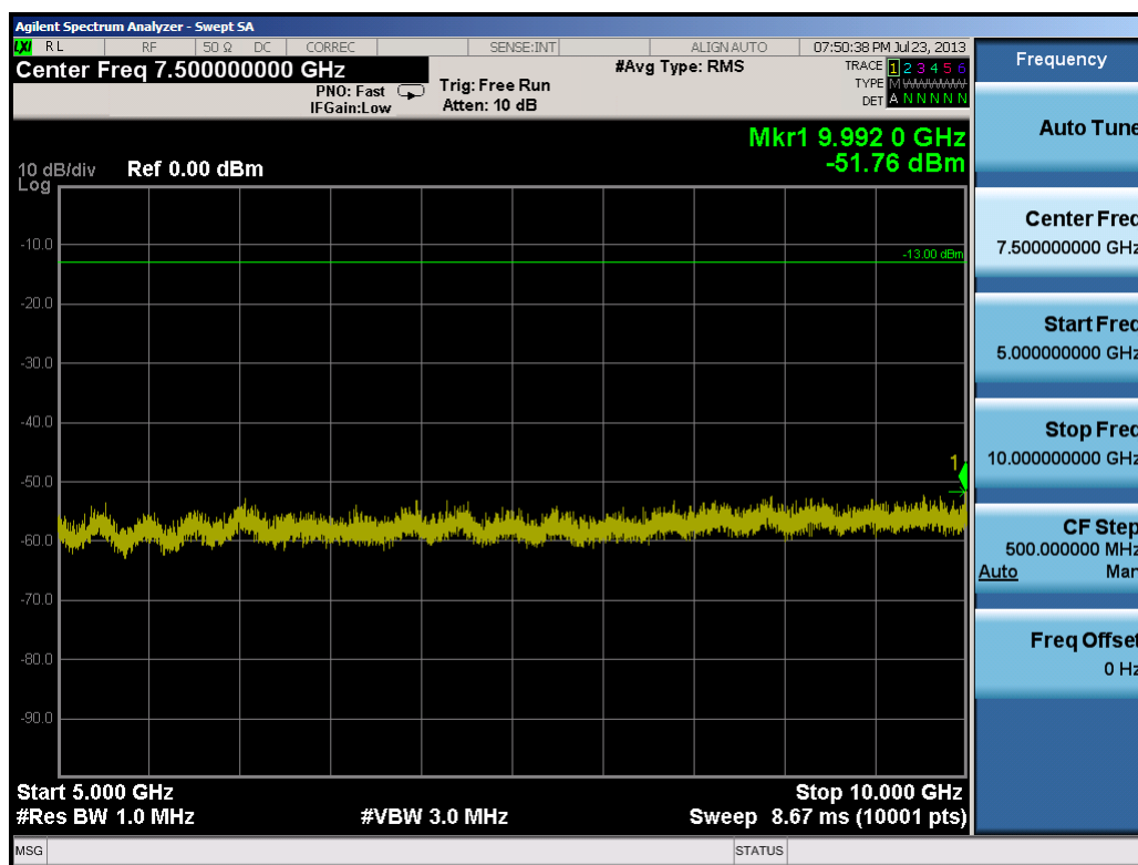
Plot 8-17. Conducted Spurious Plot (10.0MHz QPSK – RB Size 1, RB Offset 0 – Mid Channel)
