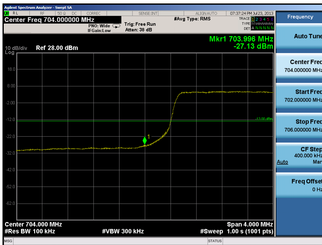
Plot 7-11. Lower Band Edge Plot (10.0MHz QPSK – RB Size 50)
