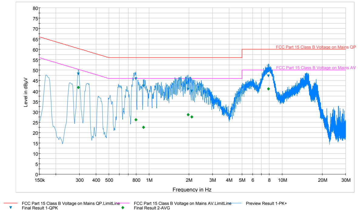
Plot 6-5. Line-Conducted Test Plot (L1)
