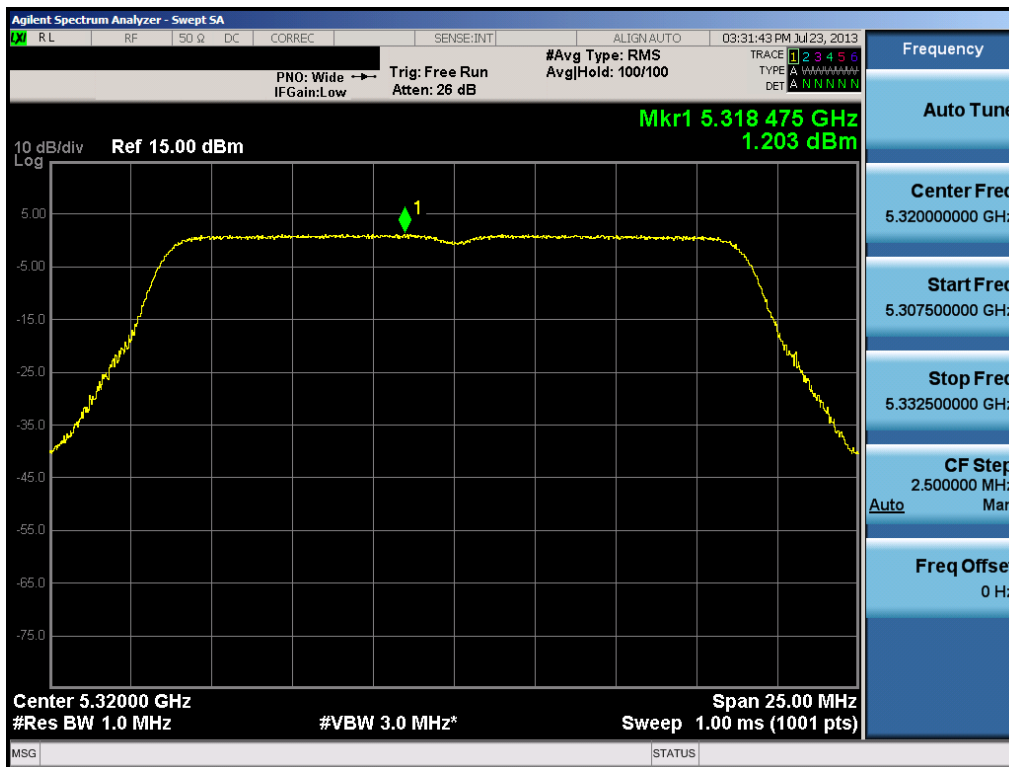
Plot 6-47. Peak Power Spectral Density Plot (20MHz BW 802.11n (UNII Band 2) – Ch. 64)
