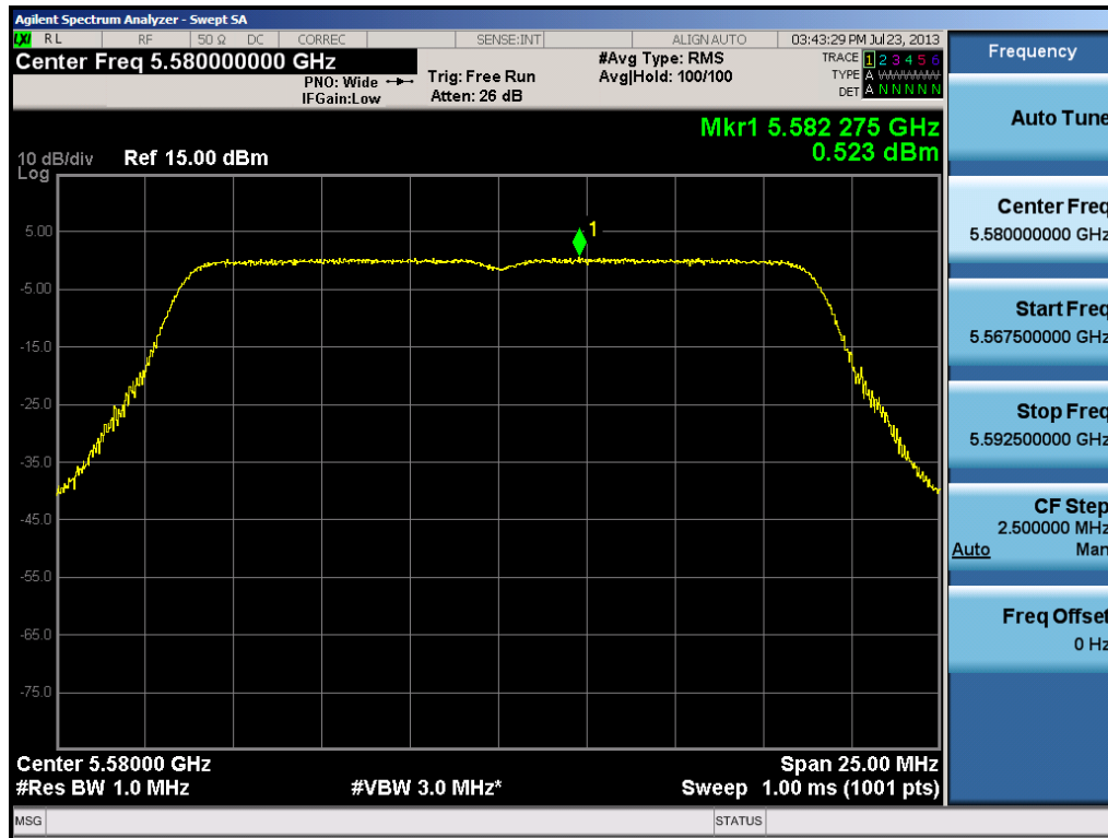
Plot 6-55. Peak Power Spectral Density Plot (20MHz BW 802.11n (UNII Band 3) – Ch. 116)
