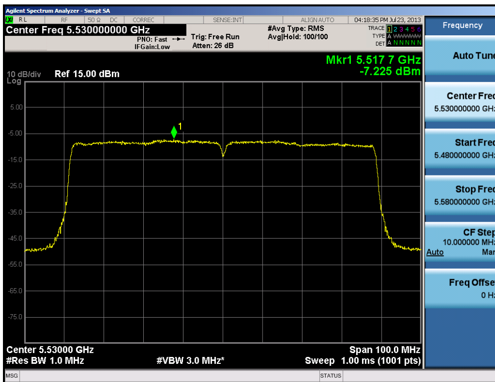
Plot 6-60. Peak Power Spectral Density Plot (80MHz BW 802.11a (UNII Band 3) – Ch. 106)
