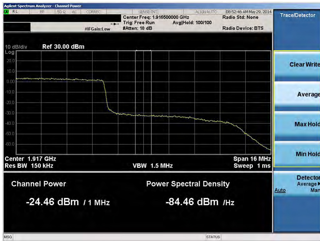
Plot 7-54. Upper Extended Band Edge Plot (20.0MHz QPSK – RB Size 100)
