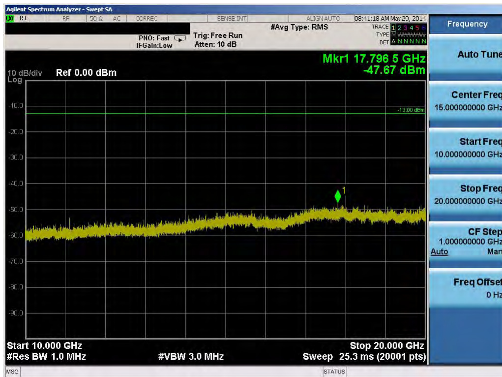
Plot 7-34. Conducted Spurious Plot (15.0MHz QPSK – RB Size 1, RB Offset 0 – Low Channel)
