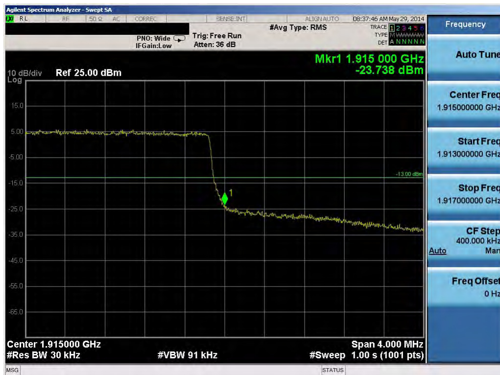
Plot 7-25. Upper Band Edge Plot (3.0MHz QPSK – RB Size 15)
