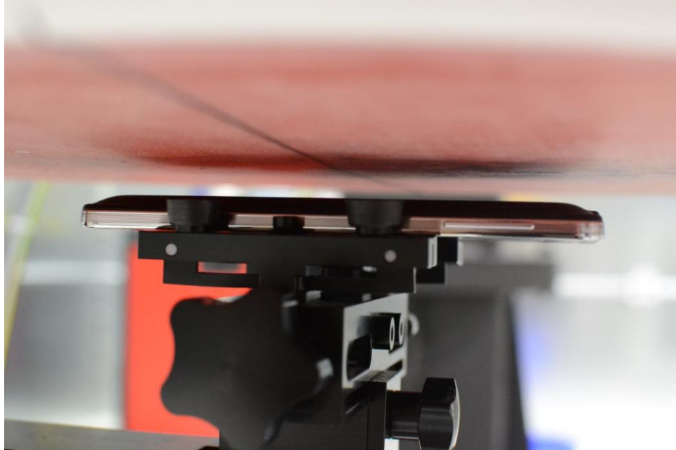
SAR Test Setup Photo 7 – Back Side at 1.0 cm with Wireless Charging Cover
