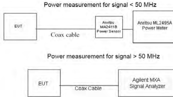
Figure 9-3 Power Measurement Setup
