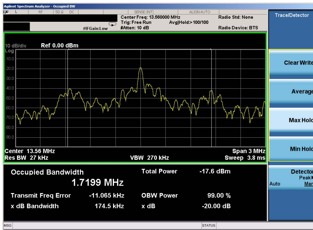
Figure 8-2. 20dB Bandwidth Plot
