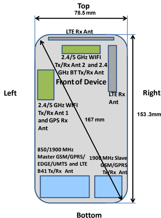
Figure 1-1 DUT Antenna Locations
