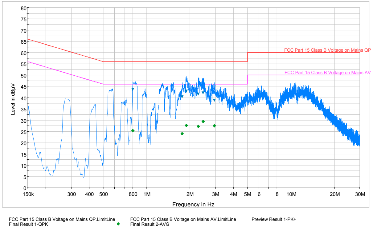
Plot 6-9. Line-Conducted Test Plot (N)
