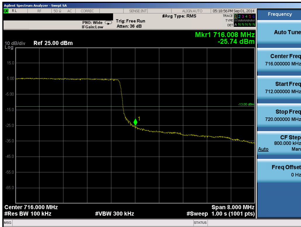
Plot 6-72. Upper Band Edge Plot (Band 12 – 10.0MHz QPSK – RB Size 50)
