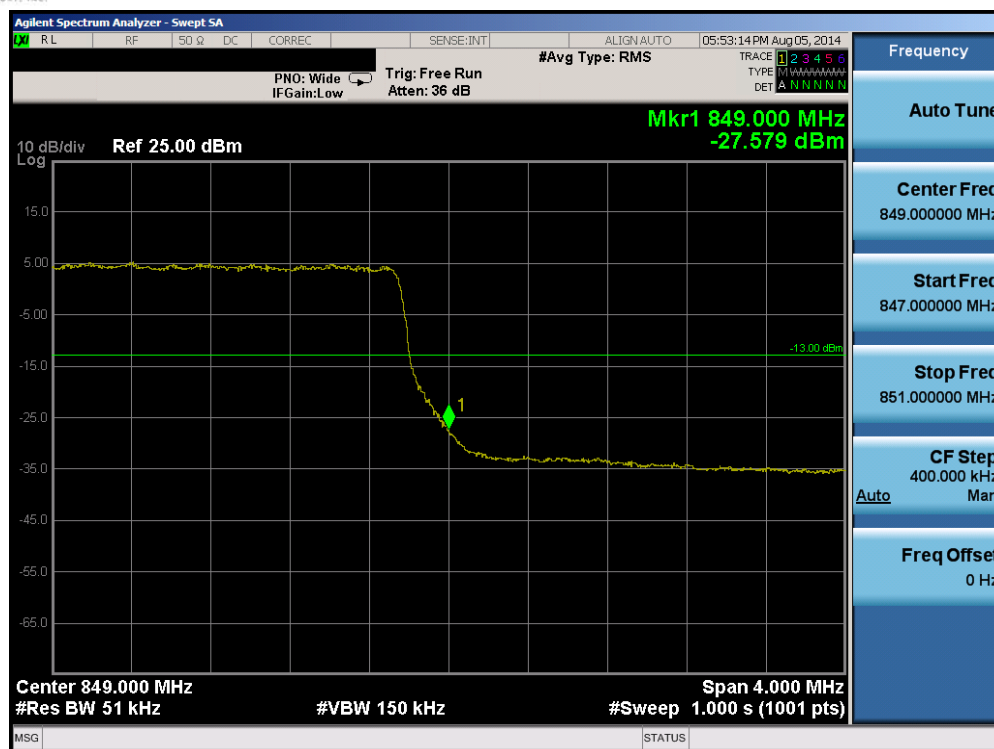
Plot 6-83. Upper Band Edge Plot (Band 5 – 5.0MHz QPSK – RB Size 25)
