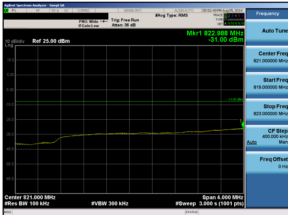
Plot 6-82. Lower Extended Band Edge Plot (Band 5 - 5.0MHz QPSK - RB Size 25)
