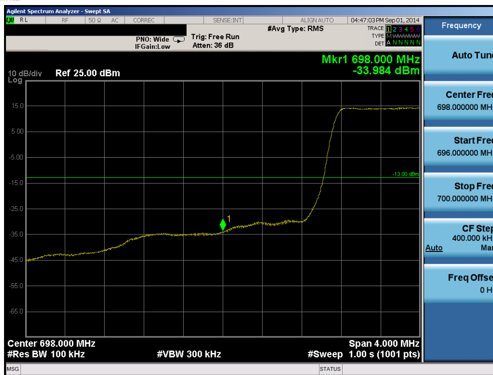
Plot 6-65. Lower Band Edge Plot (Band 12 – 1.4MHz QPSK – RB Size 6)
