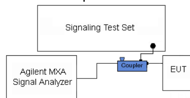
Figure 6-3. Test Instrument & Measurement Setup
