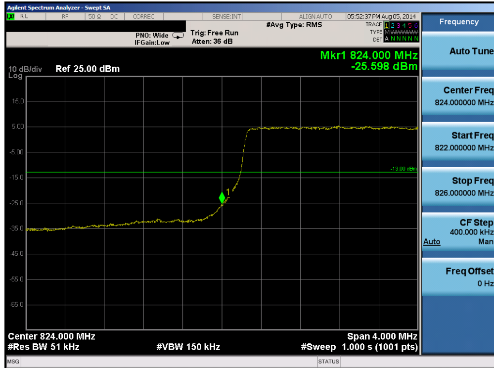
Plot 6-81. Lower Band Edge Plot (Band 5 - 5.0MHz QPSK - RB Size 25)
