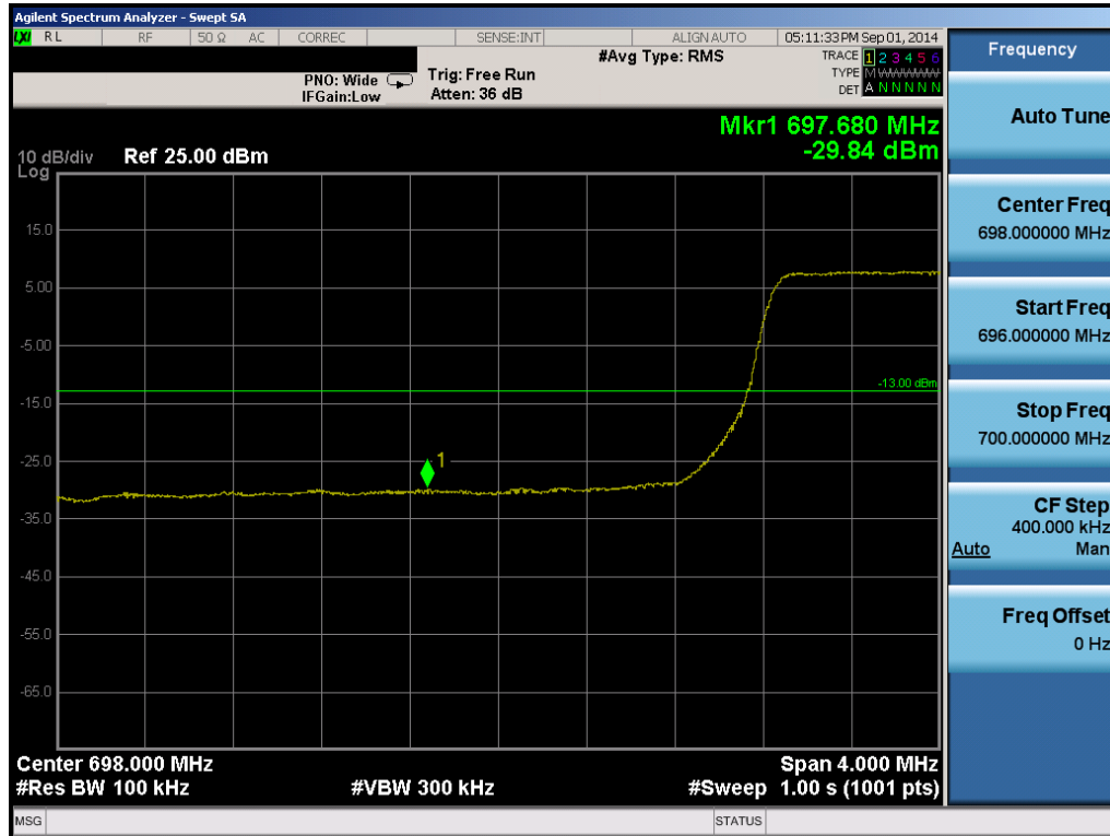
Plot 6-69. Lower Band Edge Plot (Band 12 – 5.0MHz QPSK – RB Size 25)
