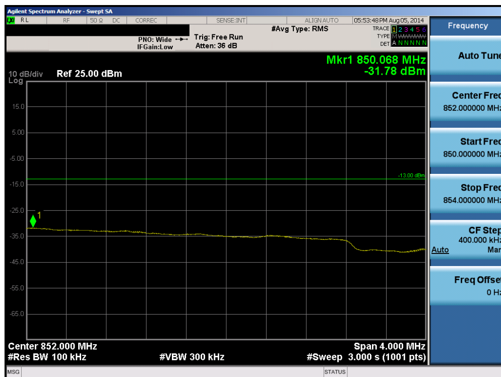
Plot 6-84. Upper Extended Band Edge Plot (Band 5 – 5.0MHz QPSK – RB Size 25)
