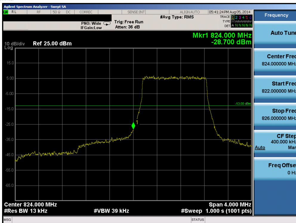
Plot 6-73. Lower Band Edge Plot (Band 5 – 1.4MHz QPSK – RB Size 6)
