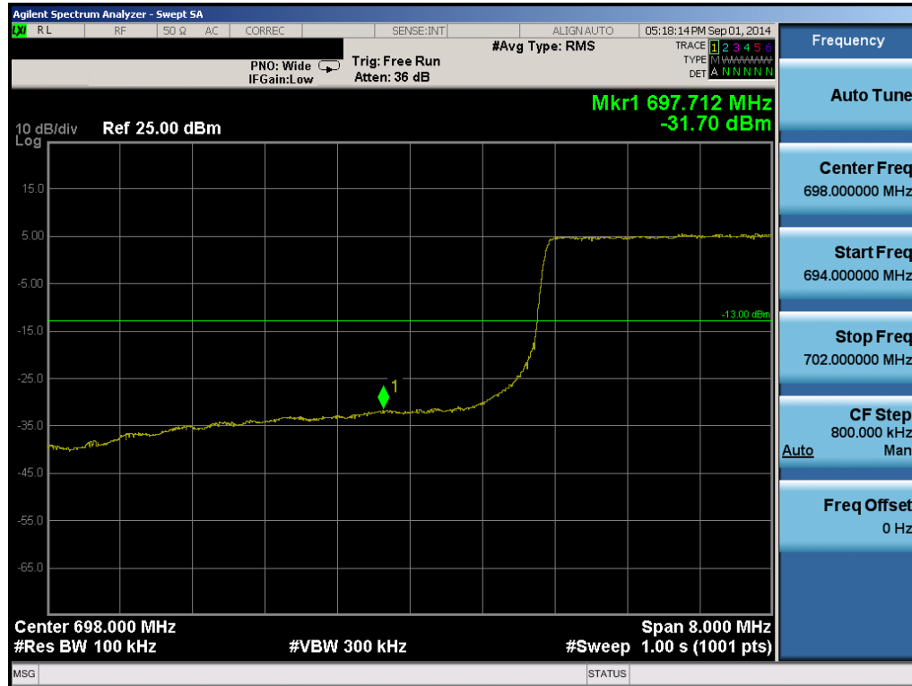
Plot 6-71. Lower Band Edge Plot (Band 12 – 10.0MHz QPSK – RB Size 50)
