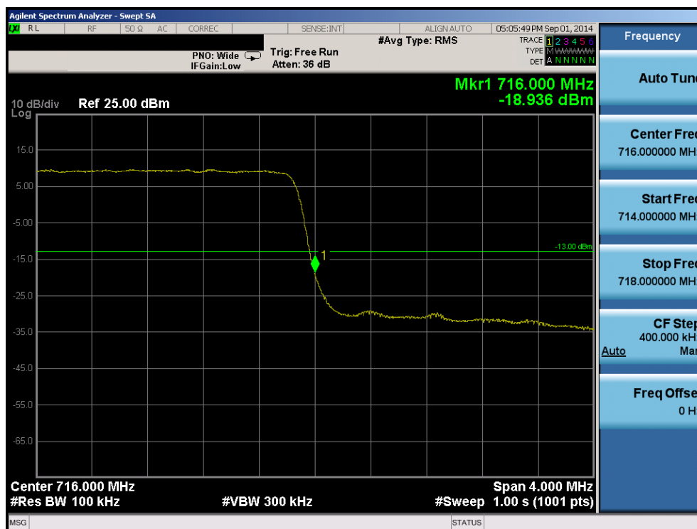
Plot 6-68. Upper Band Edge Plot (Band 12 – 3.0MHz QPSK – RB Size 15)
