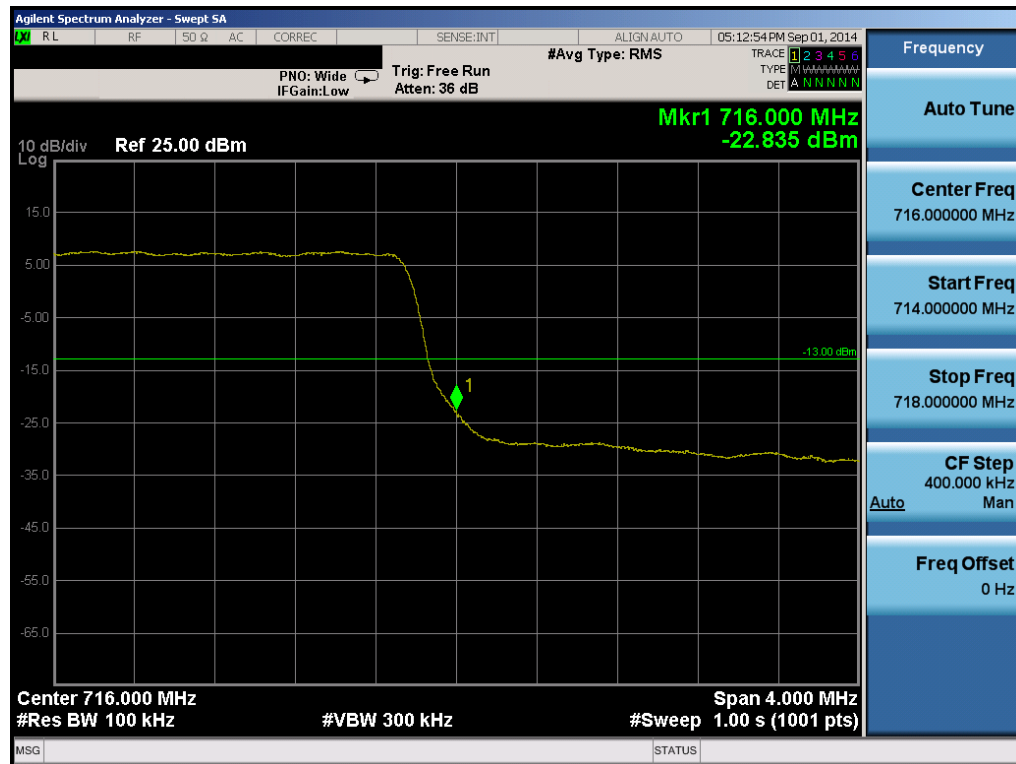
Plot 6-70. Upper Band Edge Plot (Band 12 – 5.0MHz QPSK – RB Size 25)
