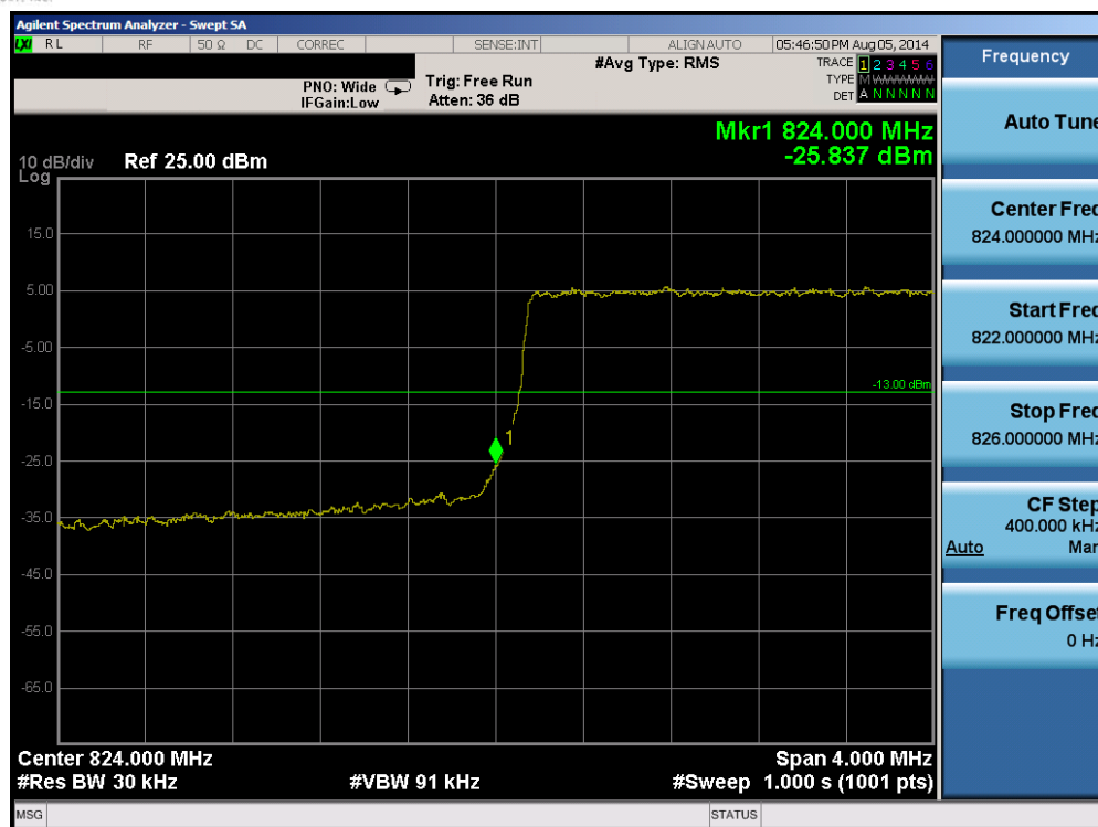
Plot 6-77. Lower Band Edge Plot (Band 5 – 3.0MHz QPSK – RB Size 15)
