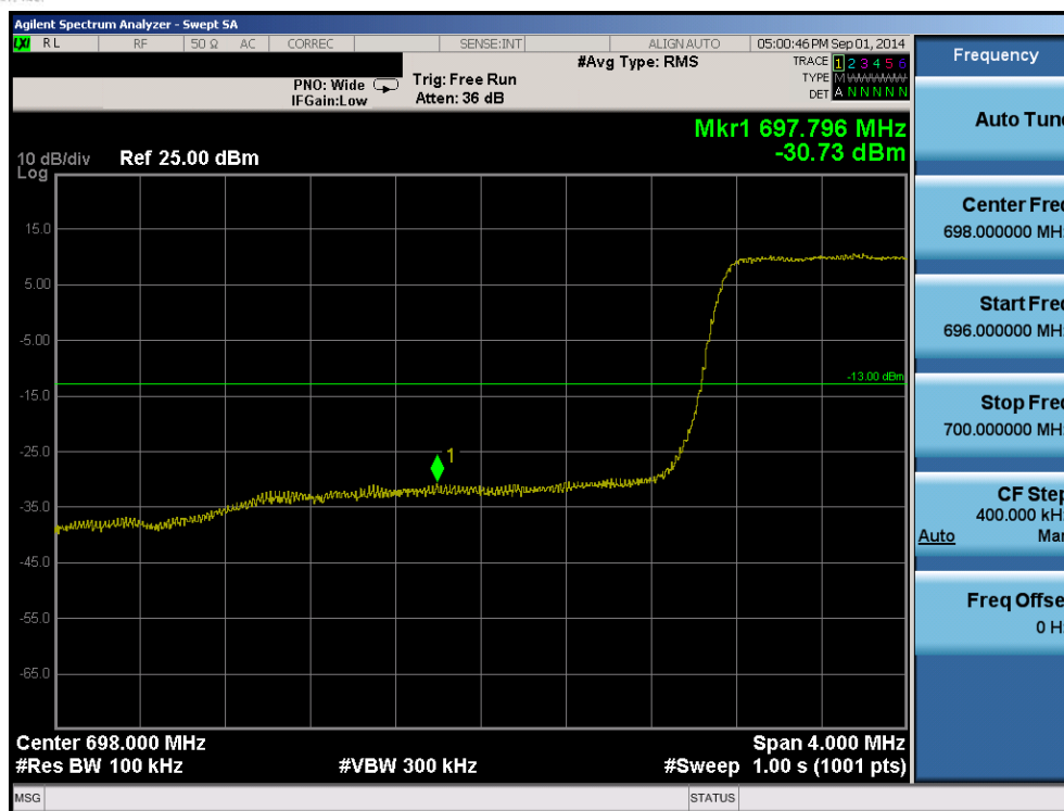
Plot 6-67. Lower Band Edge Plot (Band 12 – 3.0MHz QPSK – RB Size 15)
