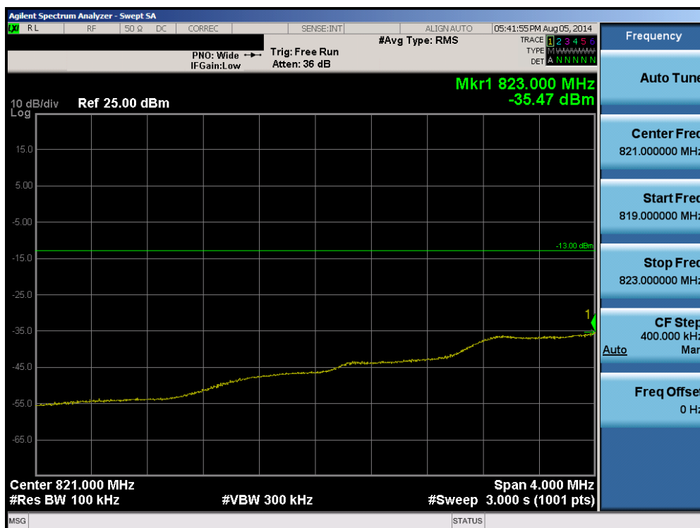
Plot 6-74. Lower Extended Band Edge Plot (Band 5 – 1.4MHz QPSK – RB Size 6)
