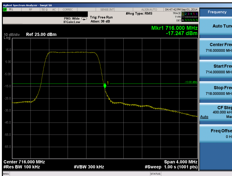
Plot 6-66. Upper Band Edge Plot (Band 12 – 1.4MHz QPSK – RB Size 6)
