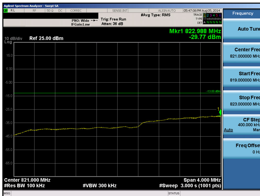
Plot 6-78. Lower Extended Band Edge Plot (Band 5 – 3.0MHz QPSK – RB Size 15)
