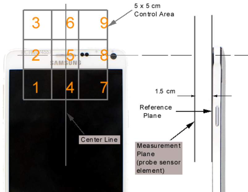
Figure 18-4 5x5 Scan grid above WD
