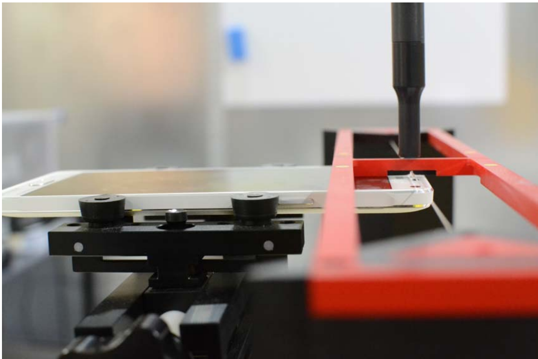
Figure 18-2 HAC Phantom Plane Alignment (with Standard Battery Cover)
