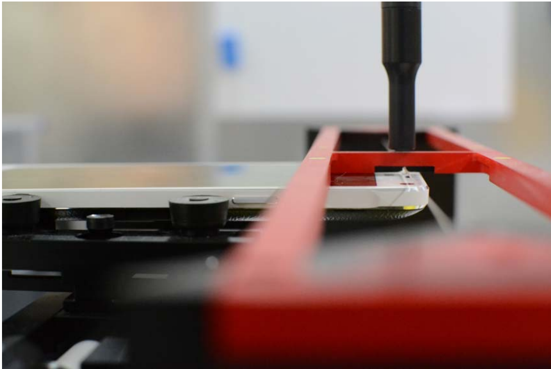
Figure 18-3 HAC Phantom Plane Alignment (with Wireless Charging Cover)
