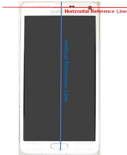
SAR Test Setup Photo 25 – DUT Reference Lines
