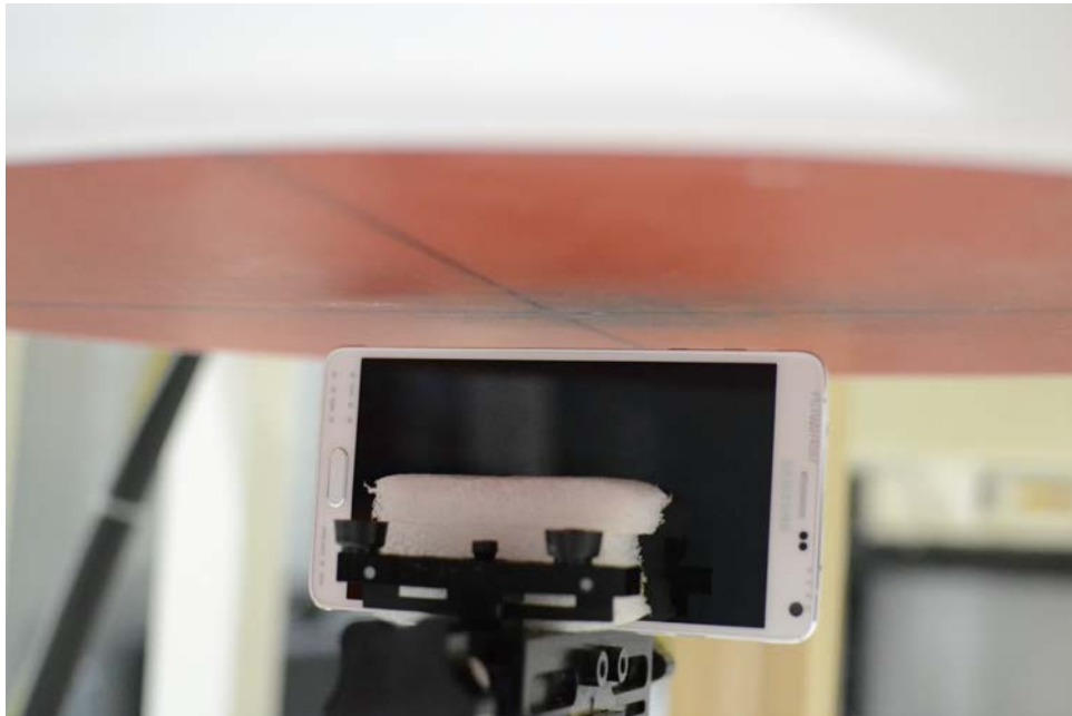
SAR Test Setup Photo 24 – Left Edge at 1.0 cm (Hotspot), Standard Cover
