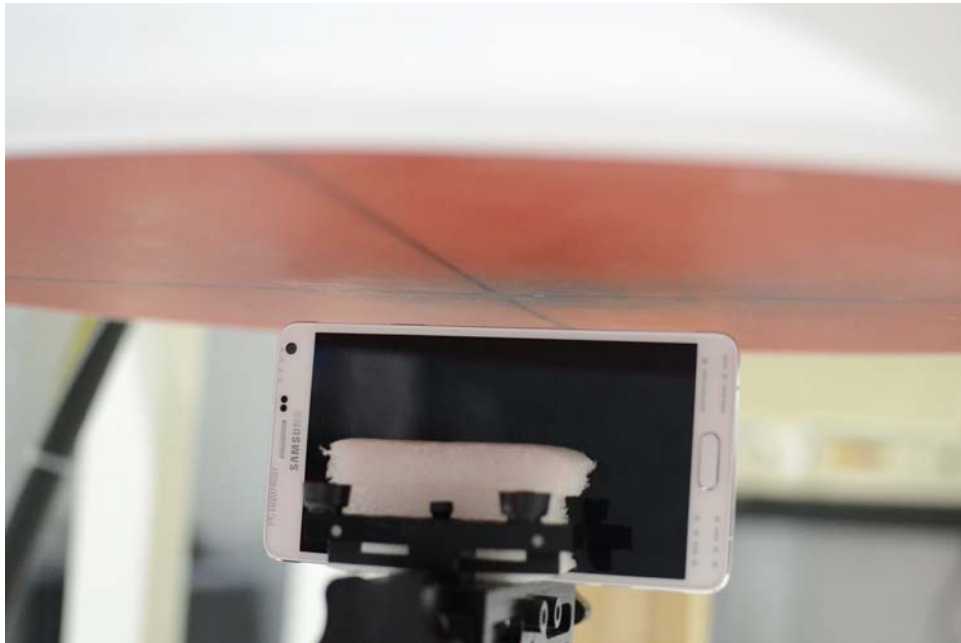
SAR Test Setup Photo 22 – Right Edge at 1.0 cm (Hotspot), Standard Cover
