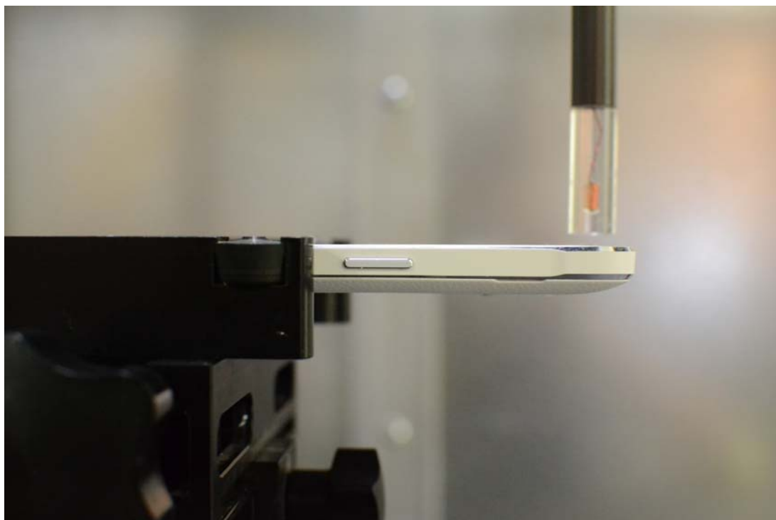
Figure 13-2 Test Setup for Wireless Device (with Standard Battery Cover)
