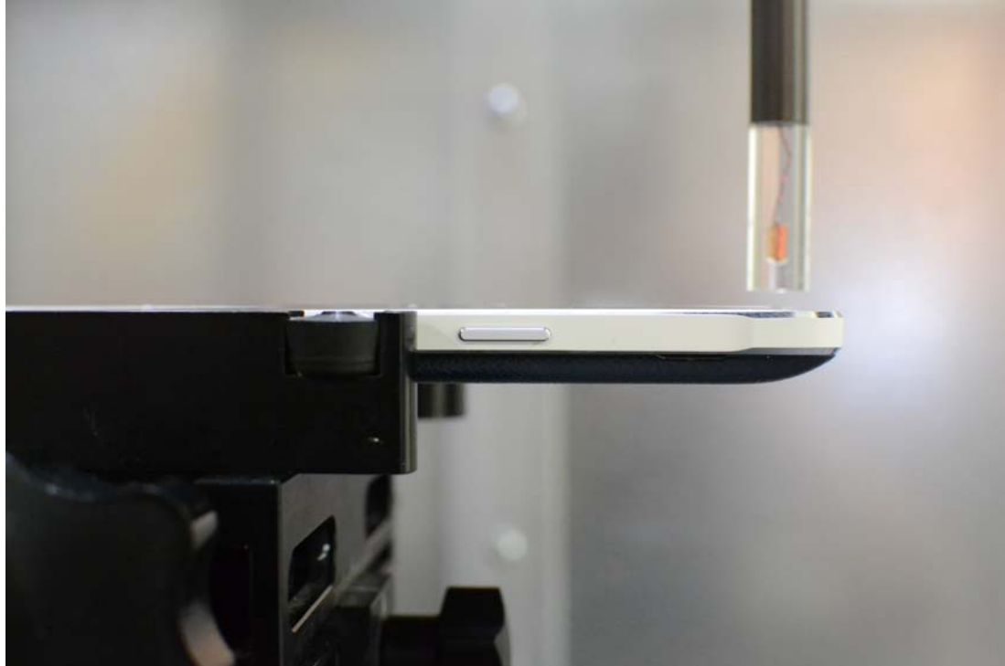
Figure 13-3 Test Setup for Wireless Device (with Wireless Charging Cover)
