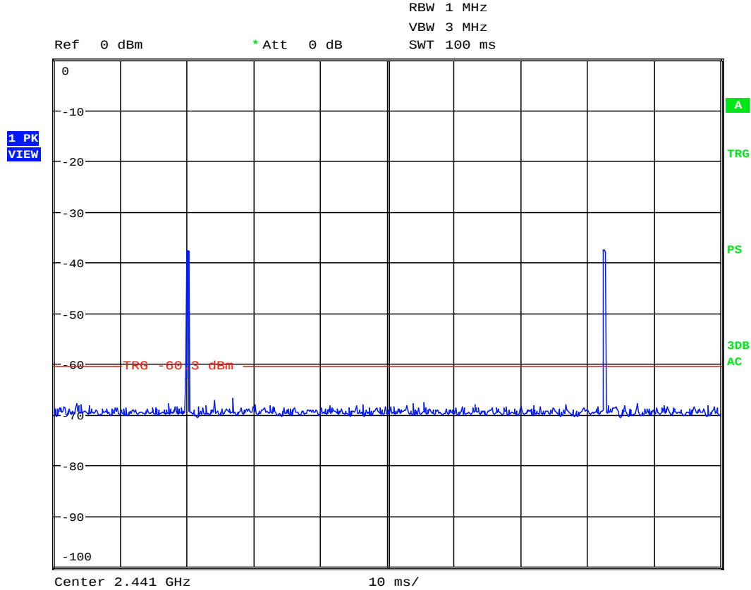
Plot 6-3. Worst Case 100ms Operation
