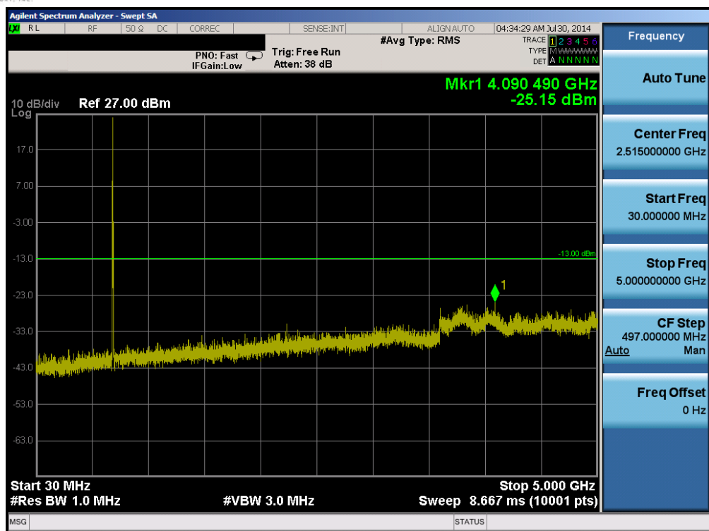
Plot 6-41. Conducted Spurious Plot (Band 17 – 10.0MHz QPSK – RB Size 1, RB Offset 0 – High Channel)
