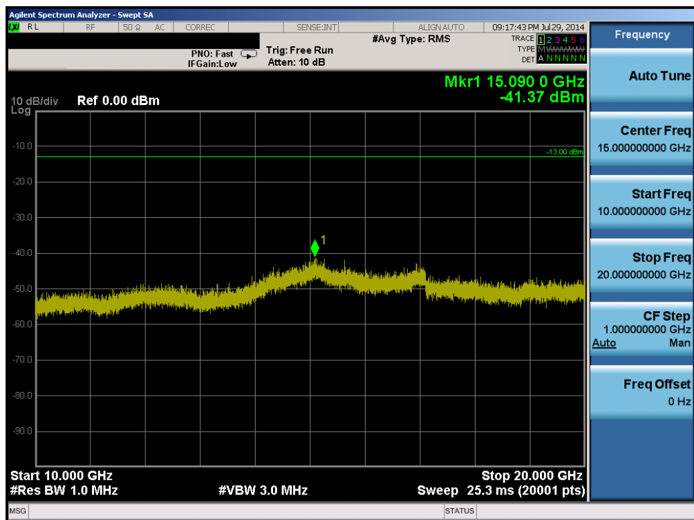
Plot 6-60. Conducted Spurious Plot (Band 2 – 20.0MHz QPSK – RB Size 1, RB Offset 0 – High Channel)
