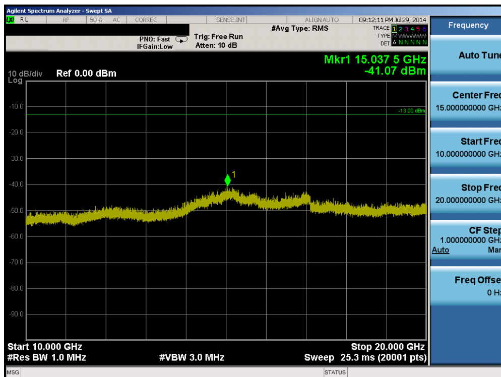
Plot 6-58. Conducted Spurious Plot (Band 2 – 20.0MHz QPSK – RB Size 1, RB Offset 0 – Mid Channel)
