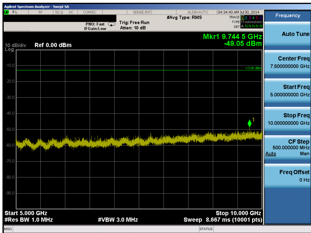
Plot 6-42. Conducted Spurious Plot (Band 17 – 10.0MHz QPSK – RB Size 1, RB Offset 0 – High Channel)
