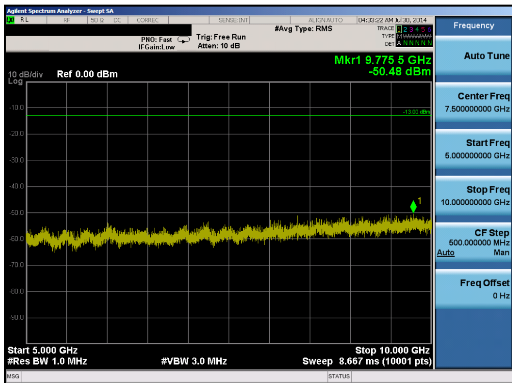
Plot 6-38. Conducted Spurious Plot (Band 17 – 10.0MHz QPSK – RB Size 1, RB Offset 0 – Low Channel)
