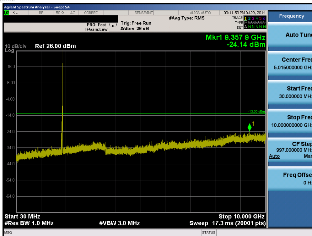
Plot 6-57. Conducted Spurious Plot (Band 2 – 20.0MHz QPSK – RB Size 1, RB Offset 0 – Mid Channel)
