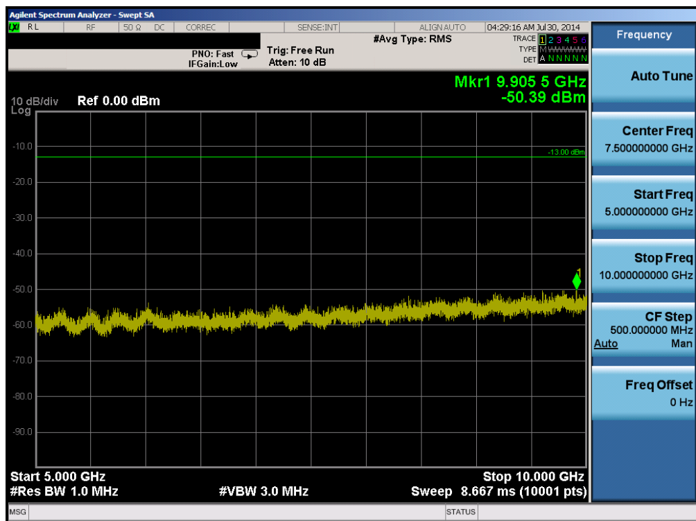
Plot 6-40. Conducted Spurious Plot (Band 17 – 10.0MHz QPSK – RB Size 1, RB Offset 0 – Mid Channel)
