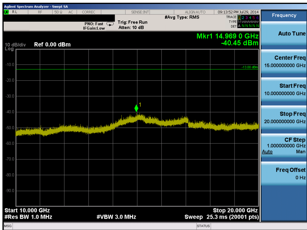
Plot 6-56. Conducted Spurious Plot (Band 2 – 20.0MHz QPSK – RB Size 1, RB Offset 0 – Low Channel)
