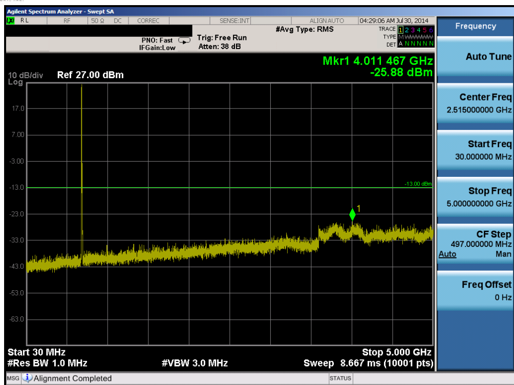
Plot 6-39. Conducted Spurious Plot (Band 17 – 10.0MHz QPSK – RB Size 1, RB Offset 0 – Mid Channel)
