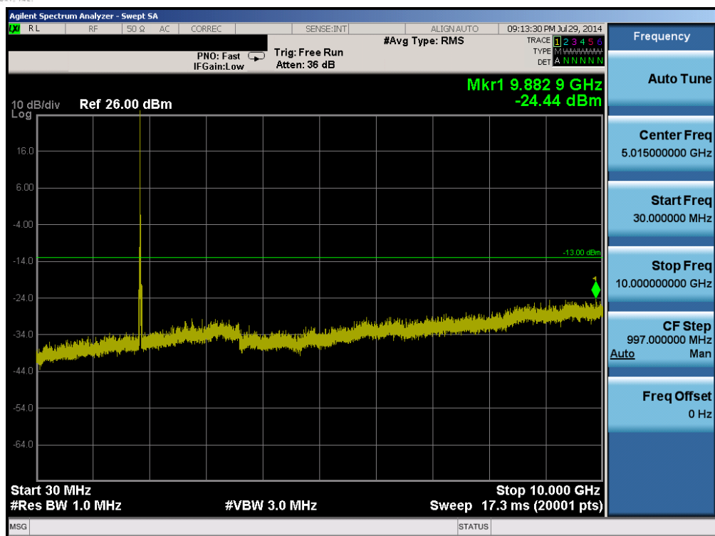
Plot 6-55. Conducted Spurious Plot (Band 2 – 20.0MHz QPSK – RB Size 1, RB Offset 0– Low Channel)
