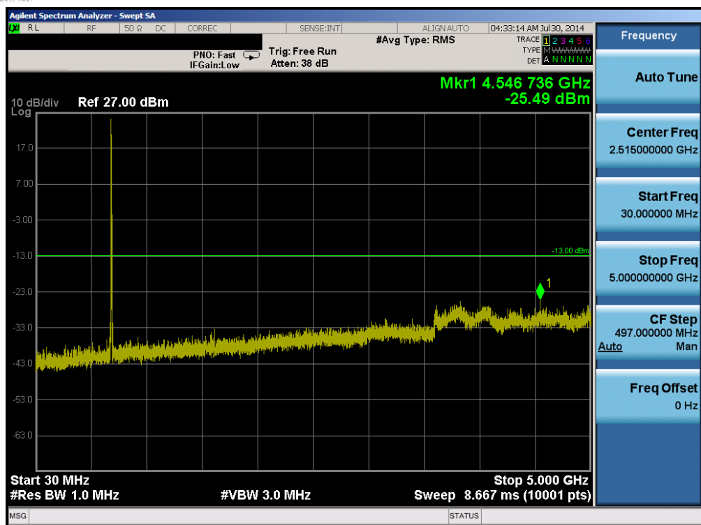
Plot 6-37. Conducted Spurious Plot (Band 17 – 10.0MHz QPSK – RB Size 1, RB Offset 0– Low Channel)
