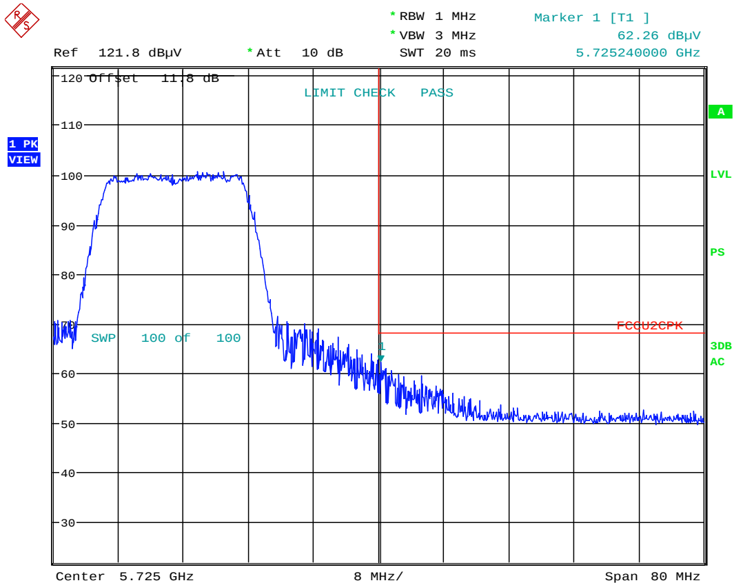
Plot 6-184. Radiated Upper Band Edge Plot (Peak – UNII Band 2C)
