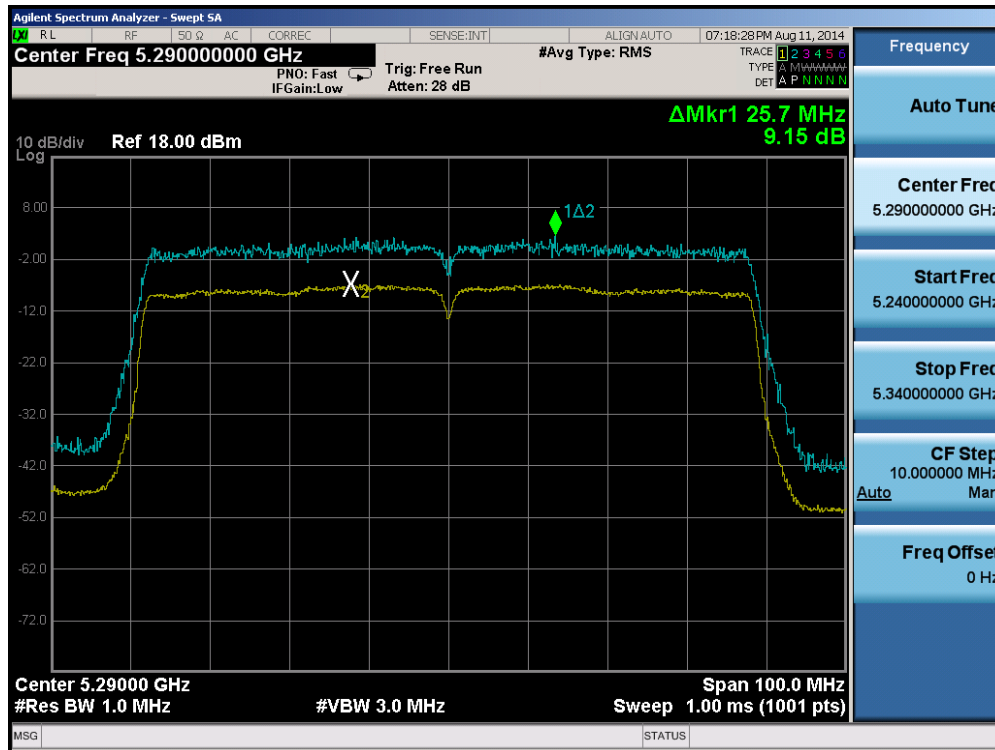
Plot 6-133. Peak Excursion Ratio Plot (80MHz BW 802.11ac (UNII Band 2A) – Ch. 58)
