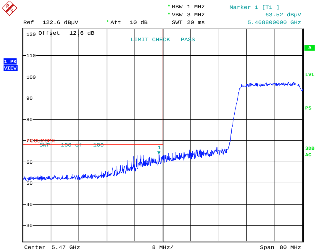
Plot 6-190. Radiated Restricted Lower Band Edge Plot (Peak – UNII Band 2C)
