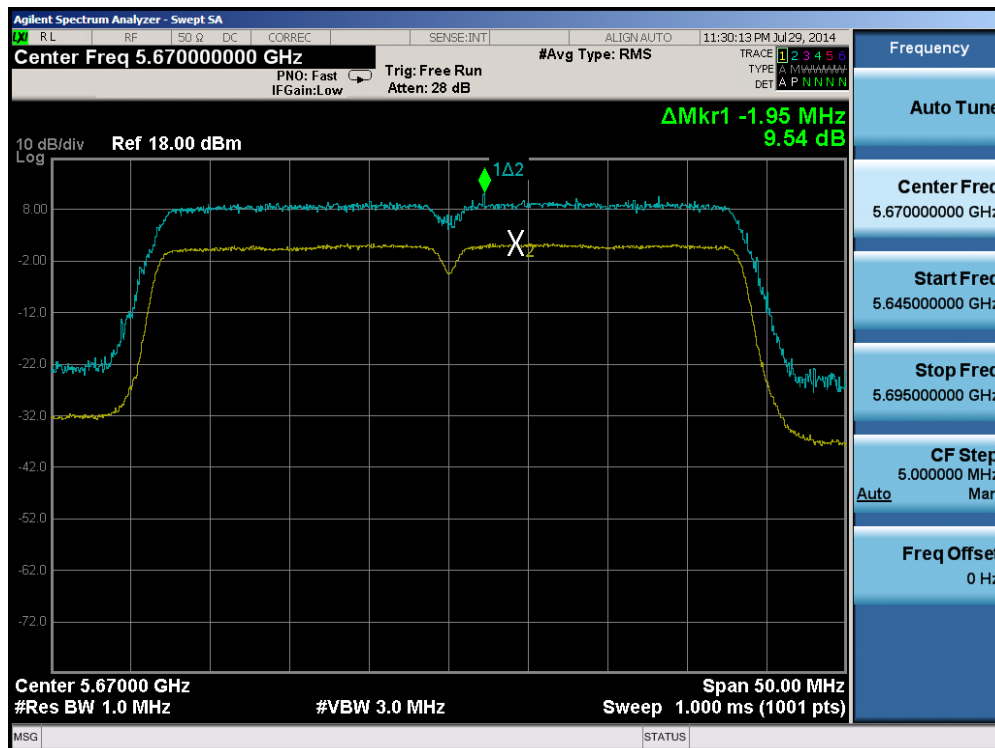
Plot 6-136. Peak Excursion Ratio Plot (40MHz BW 802.11n (UNII Band 2C) – Ch. 134)
