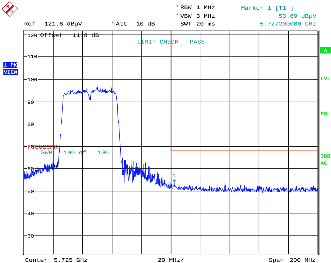
Plot 6-191. Radiated Upper Band Edge Plot (Peak – UNII Band 2C)
