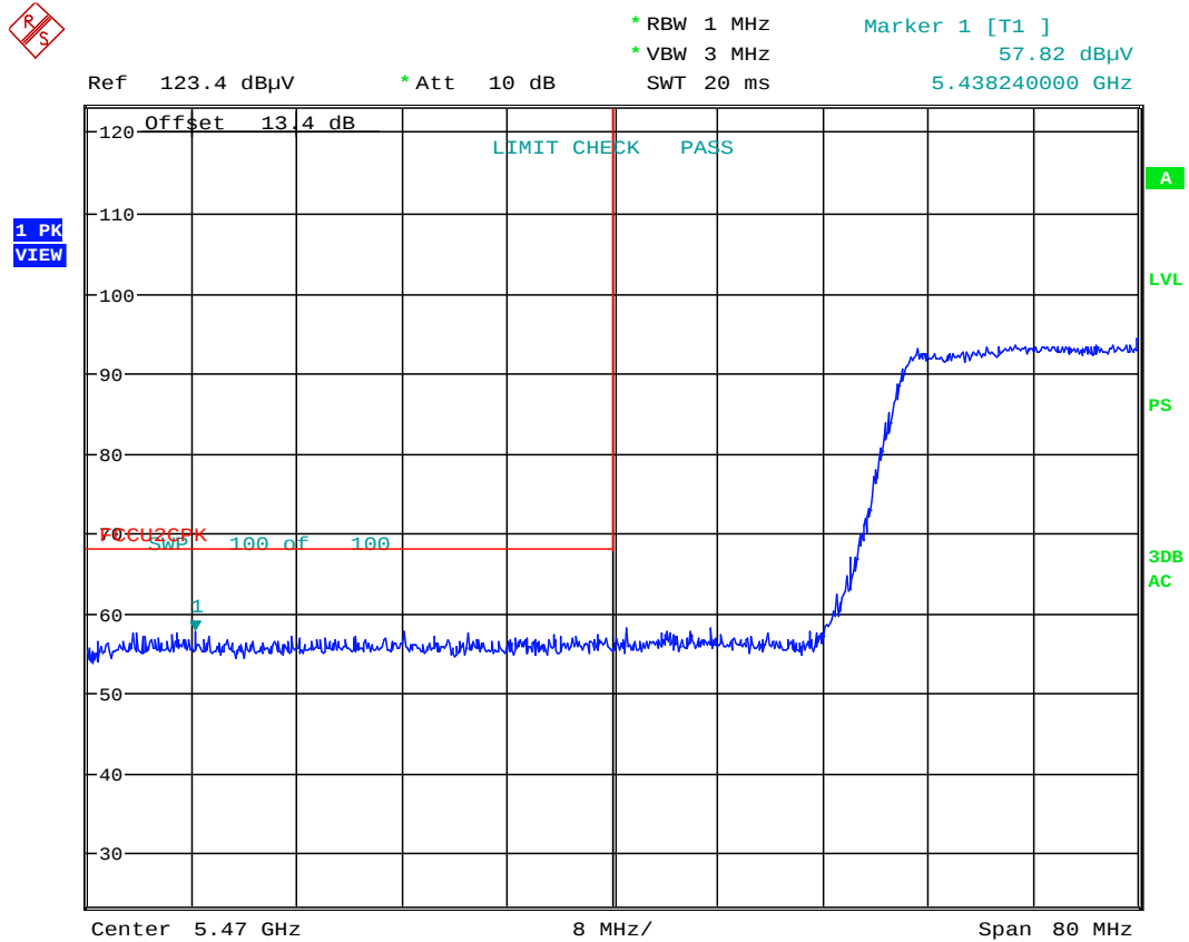
Plot 6-197. Radiated Restricted Lower Band Edge Plot (Peak – UNII Band 2C)
