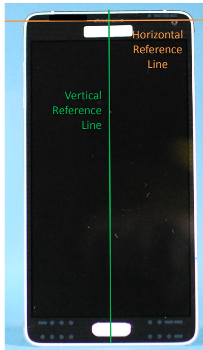
SAR Test Setup Photo 15: DUT Reference Lines
