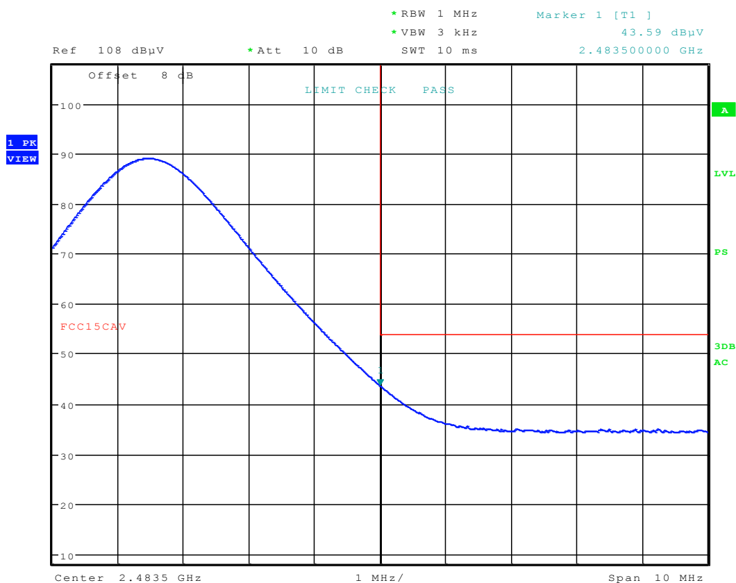
Plot 6-18. Radiated Restricted Upper Band Edge Measurement (Average)
