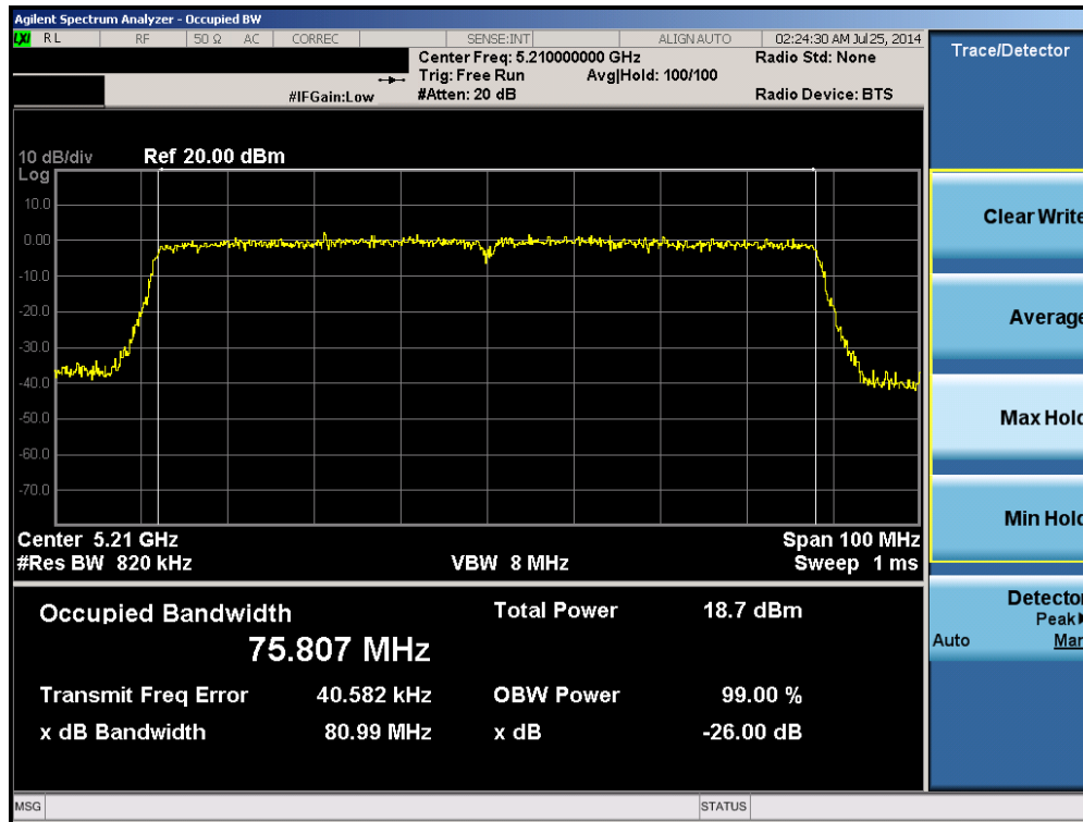
Plot 6-42. 26dB Bandwidth Plot (80MHz BW 802.11ac (UNII Band 1) – Ch. 42)
