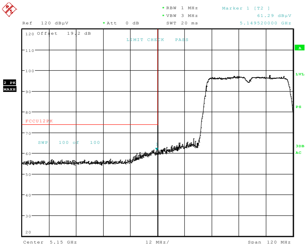
Plot 6-146. Radiated Restricted Lower Band Edge Plot (Peak – UNII Band 1)
