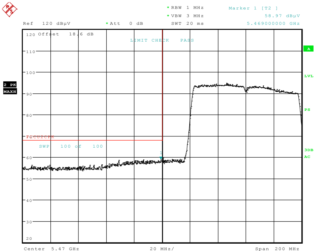
Plot 6-157. Radiated Restricted Lower Band Edge Plot (Peak – UNII Band 2C)
