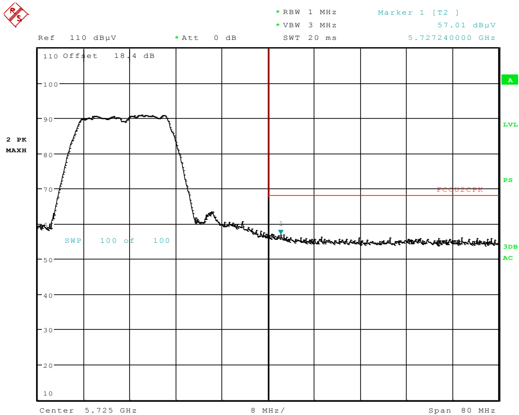
Plot 6-164. Radiated Upper Band Edge Plot (Peak – UNII Band 2C)
