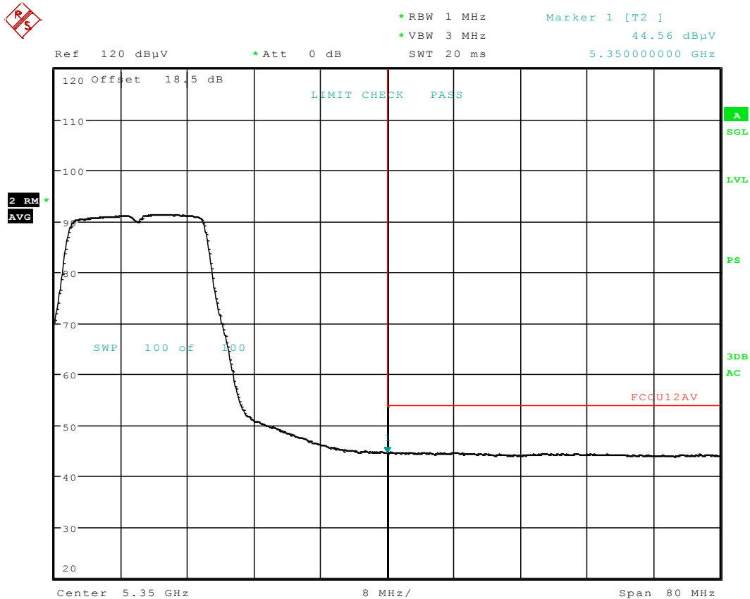
Plot 6-140. Radiated Restricted Upper Band Edge Plot (Average – UNII Band 2A)
