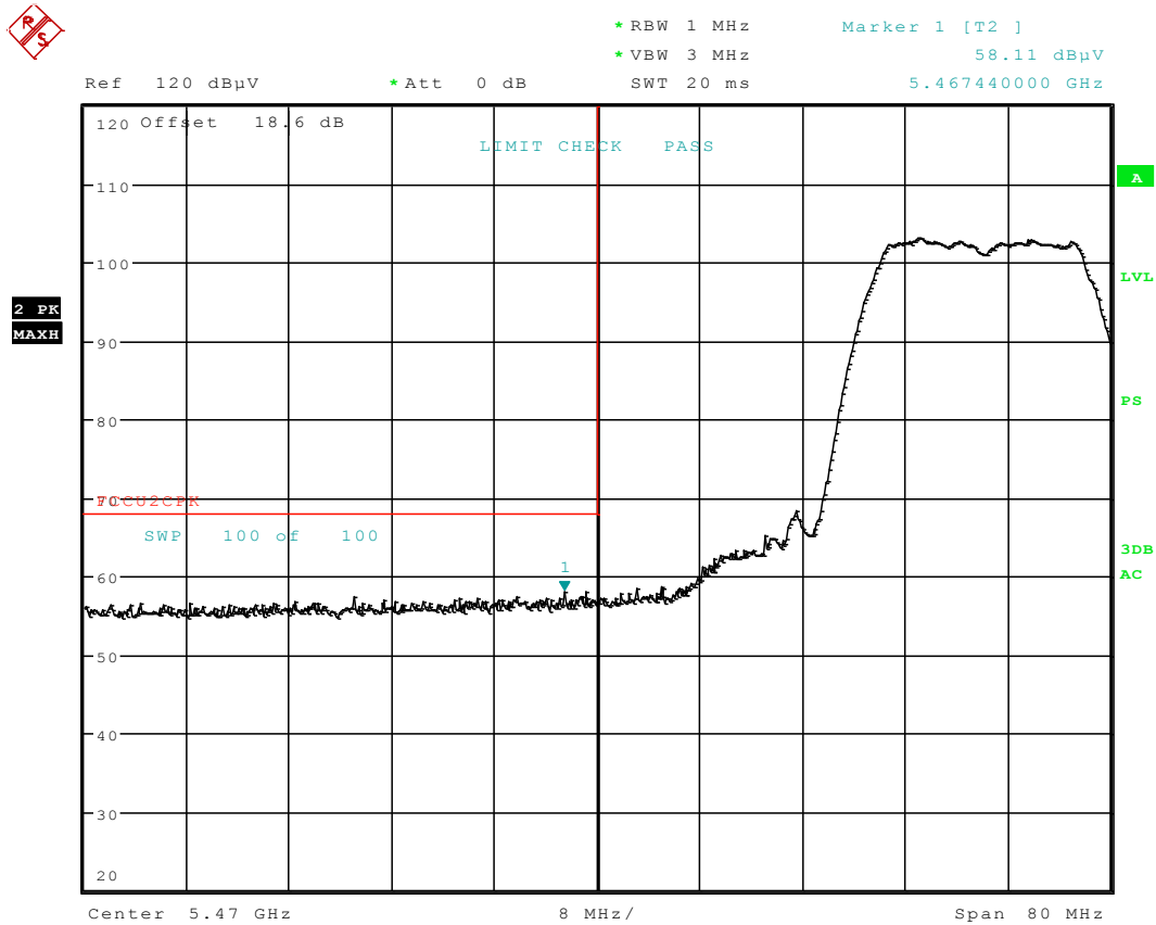
Plot 6-143. Radiated Restricted Lower Band Edge Plot (Peak – UNII Band 2C)
