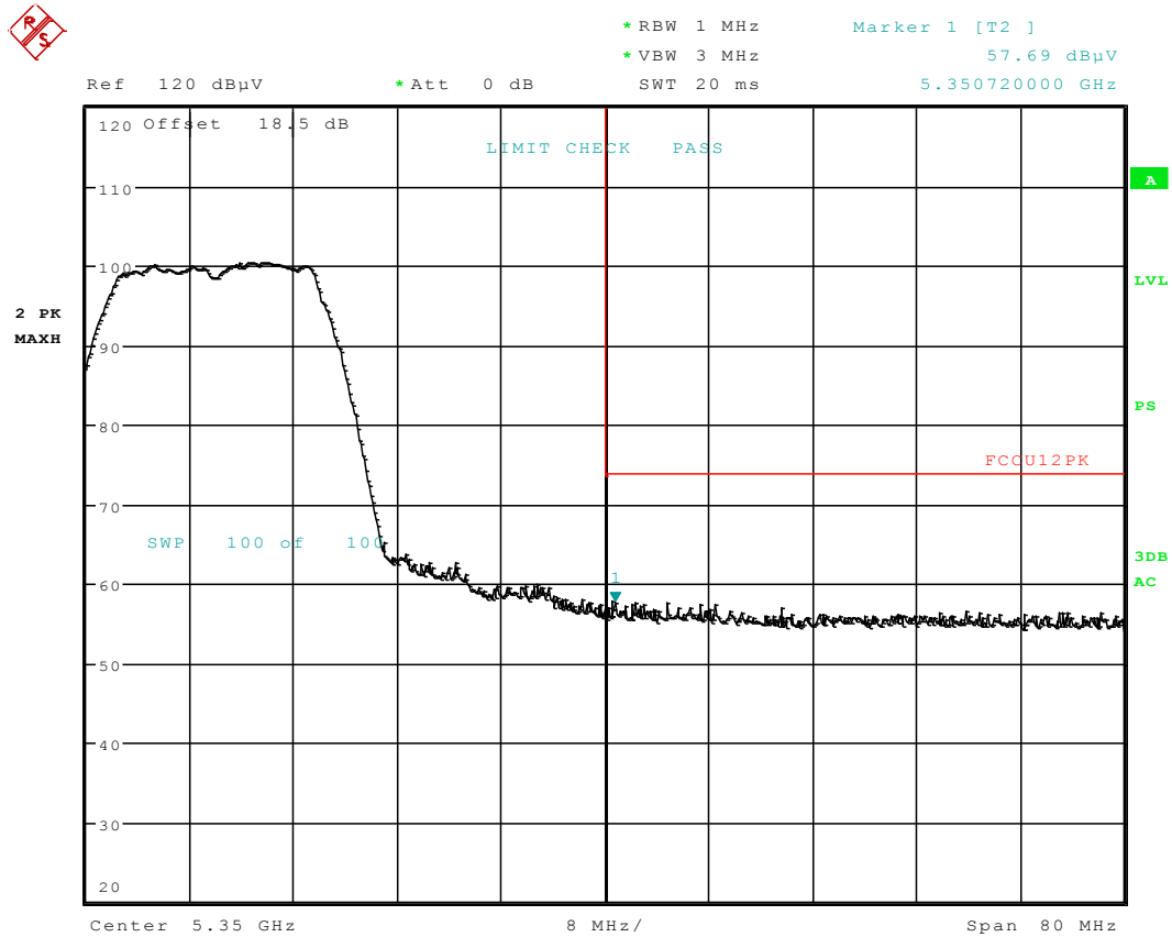
Plot 6-141. Radiated Restricted Upper Band Edge Plot (Peak – UNII Band 2A)
