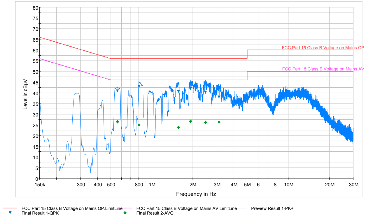
Plot 6-8. Line-Conducted Test Plot (L1)
