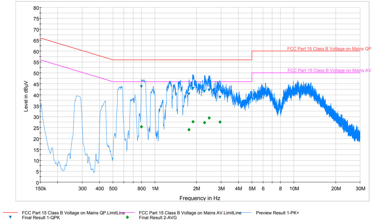
Plot 6-9. Line-Conducted Test Plot (N)
