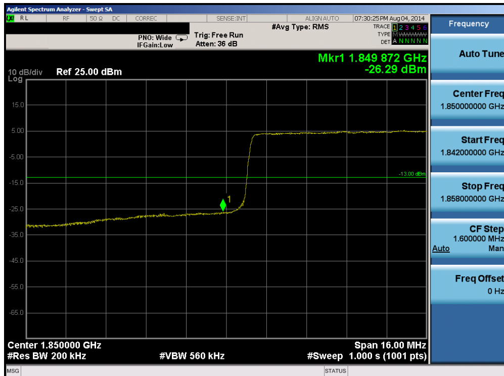
Plot 6-87. Lower Band Edge Plot (Band 25 - 20.0MHz QPSK - RB Size 100)
