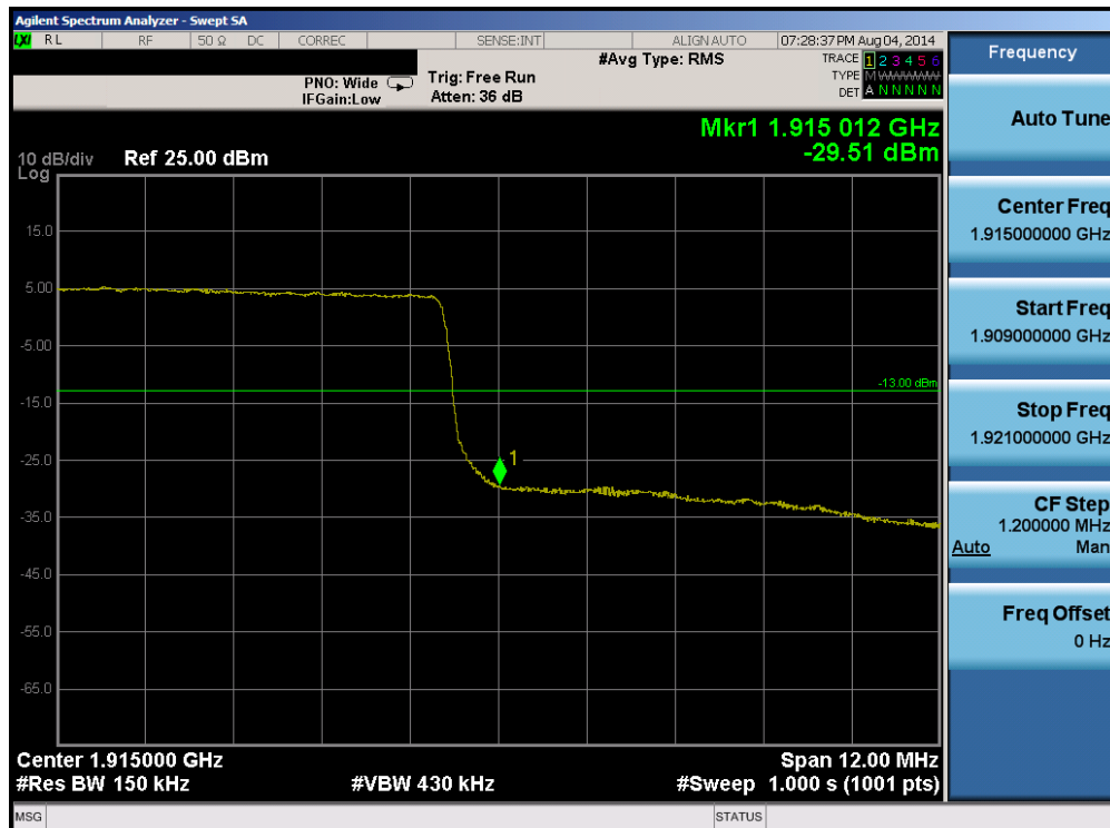
Plot 6-85. Upper Band Edge Plot (Band 25 – 15.0MHz QPSK – RB Size 75)
