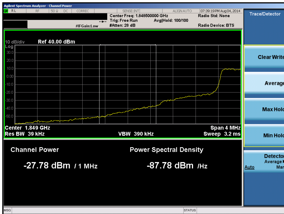
Plot 6-68. Lower Extended Band Edge Plot (Band 25 – 1.4MHz QPSK – RB Size 6)
