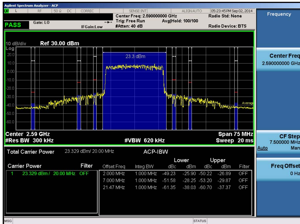
Plot 6-103. Mid ACP Plot (Band 41 – 20.0MHz QPSK – RB Size 100)
