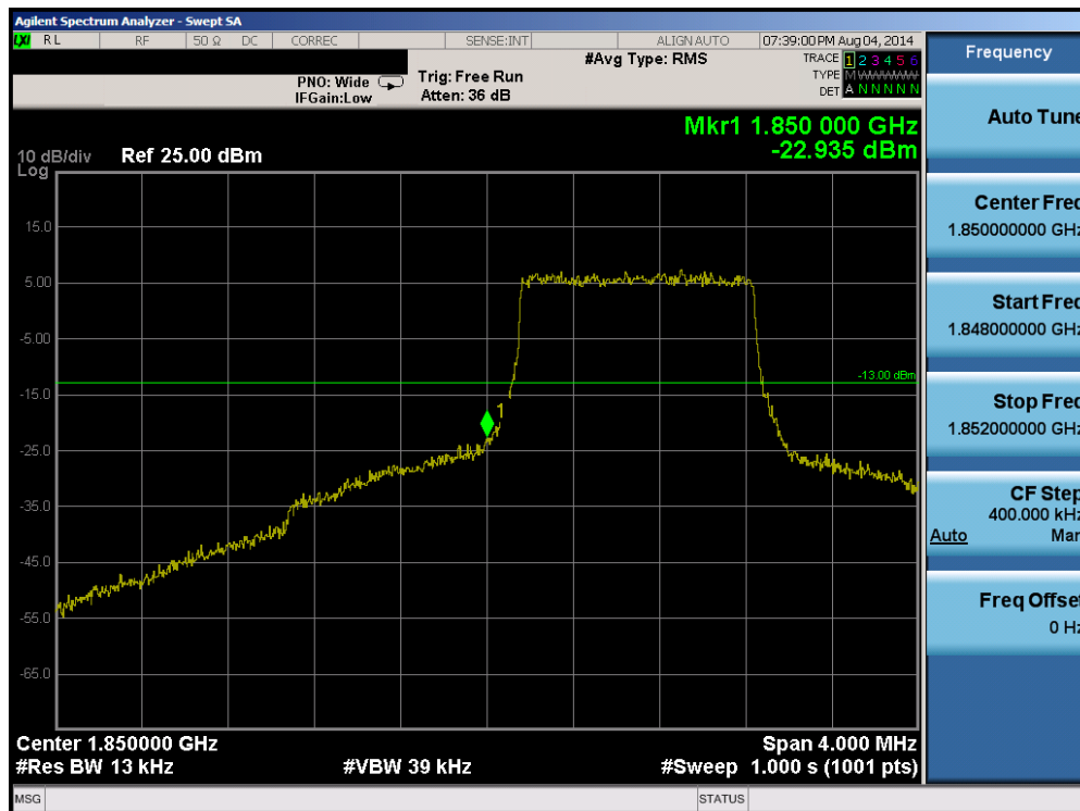
Plot 6-67. Lower Band Edge Plot (Band 25 – 1.4MHz QPSK – RB Size 6)
