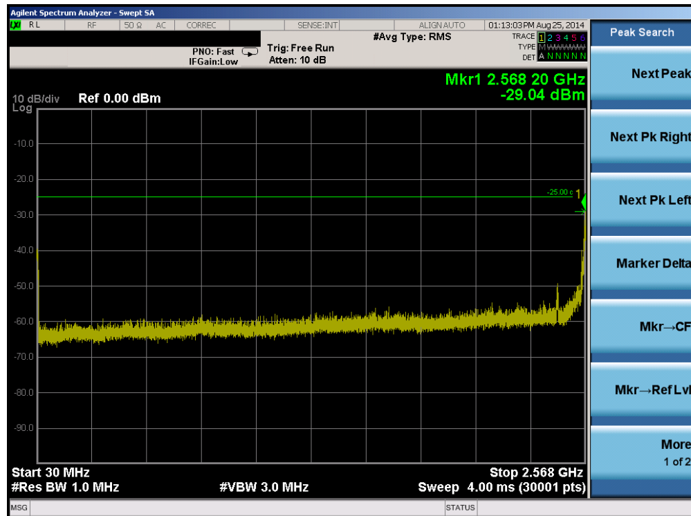
Plot 6-44. Conducted Spurious Plot (Band 41 – 15.0MHz QPSK – RB Size 75, RB Offset 0 – Mid Channel)
