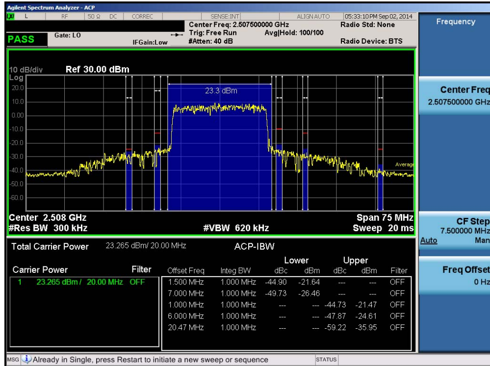
Plot 6-102. Lower ACP Plot (Band 41 – 20.0MHz QPSK – RB Size 100)
