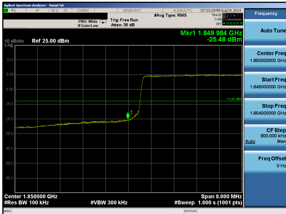
Plot 6-79. Lower Band Edge Plot (Band 25 – 10.0MHz QPSK – RB Size 50)
