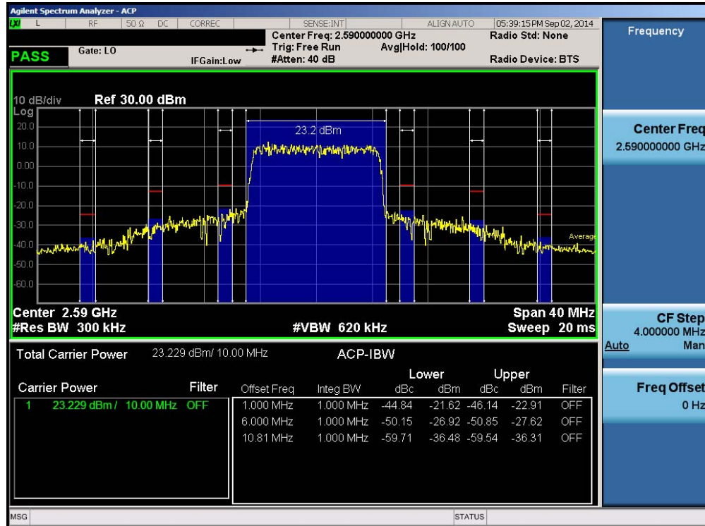
Plot 6-96. Mid ACP Plot (Band 41 – 10.0MHz QPSK – RB Size 50)
