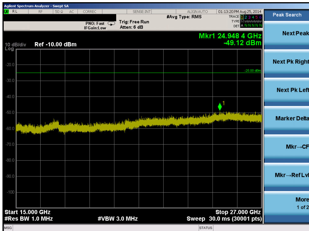
Plot 6-46. Conducted Spurious Plot (Band 41 – 15.0MHz QPSK – RB Size 75, RB Offset 0 – Mid Channel)
