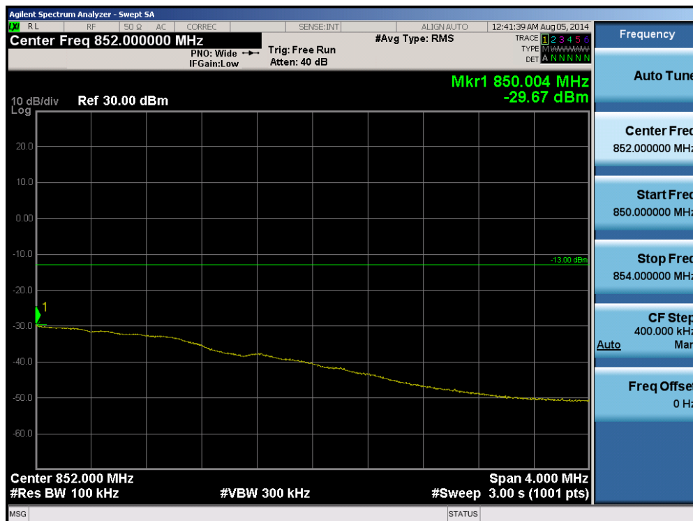
Plot 6-59. Upper Extended Band Edge Plot (Band 26 – Band 5 – 3.0MHz QPSK – RB Size 15)
