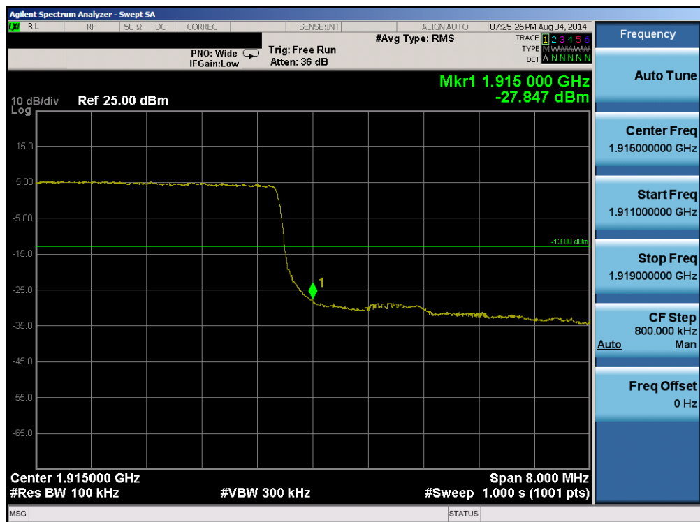
Plot 6-81. Upper Band Edge Plot (Band 25 - 10.0MHz QPSK - RB Size 50)
