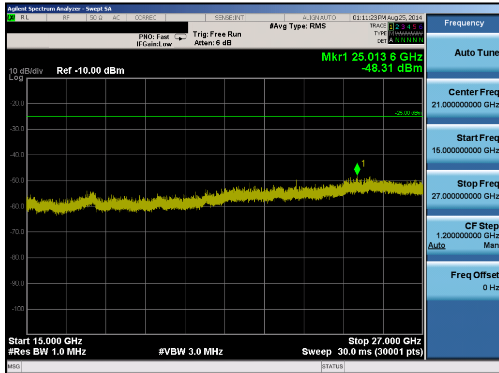
Plot 6-43. Conducted Spurious Plot (Band 41 – 15.0MHz QPSK – RB Size 75, RB Offset 0 – Low Channel)
