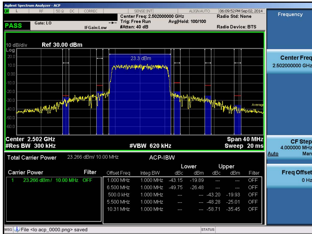
Plot 6-95. Lower ACP Plot (Band 41 – 10.0MHz QPSK – RB Size 50)
