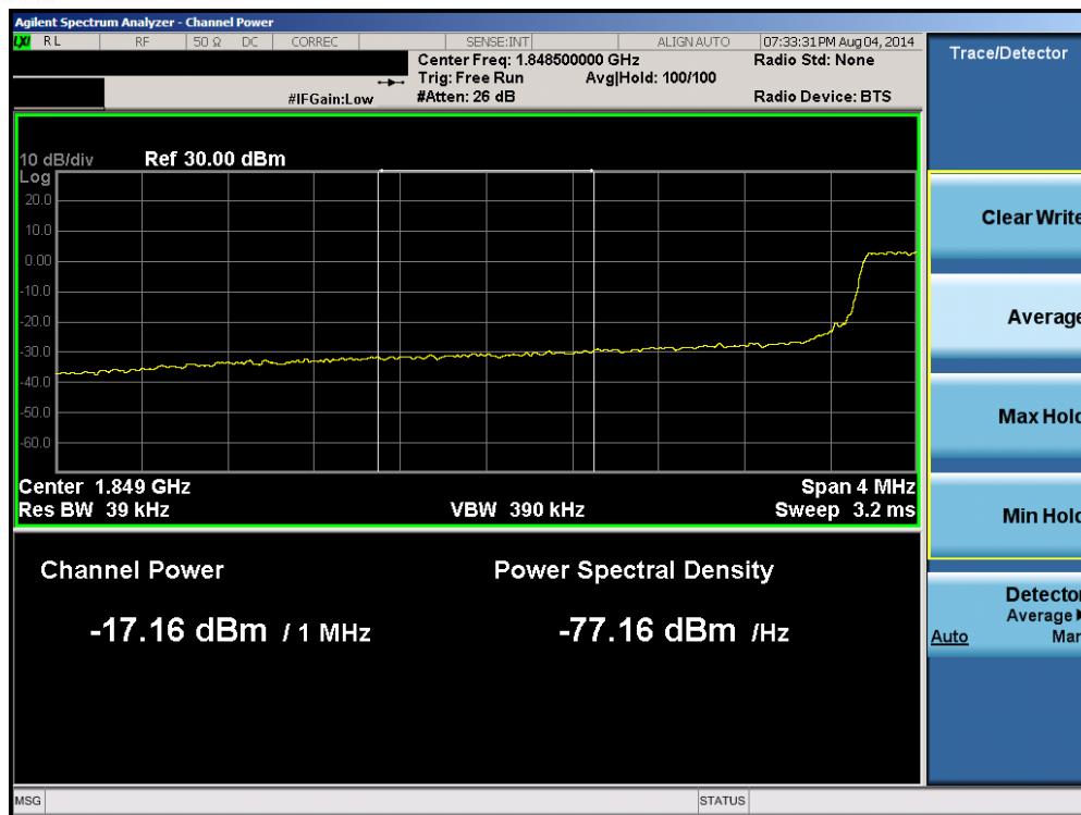
Plot 6-76. Lower Extended Band Edge Plot (Band 25 – 5.0MHz QPSK – RB Size 25)
