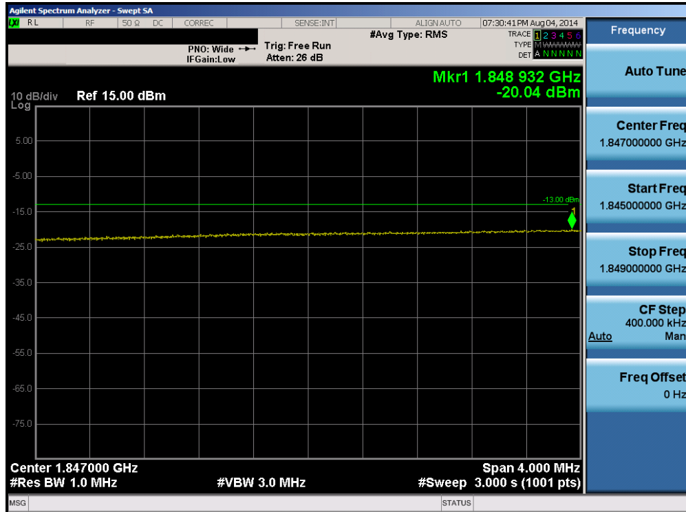
Plot 6-88. Lower Extended Band Edge Plot (Band 25 – 20.0MHz QPSK – RB Size 100)
