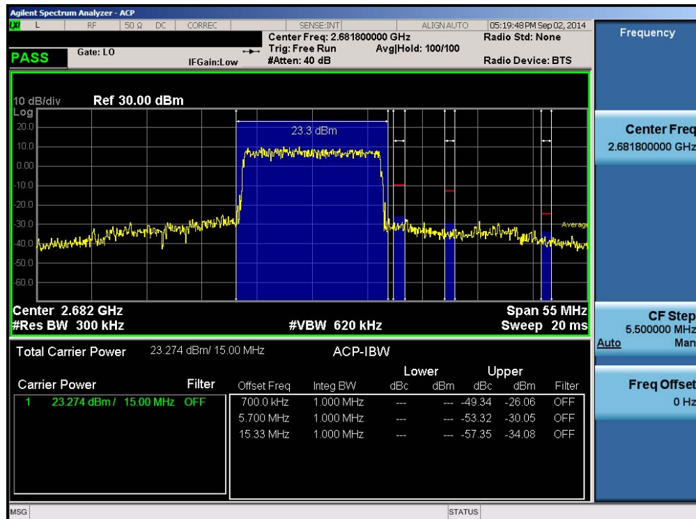
Plot 6-101. Upper-2 ACP Plot (Band 41 – 15.0MHz QPSK – RB Size 75)
