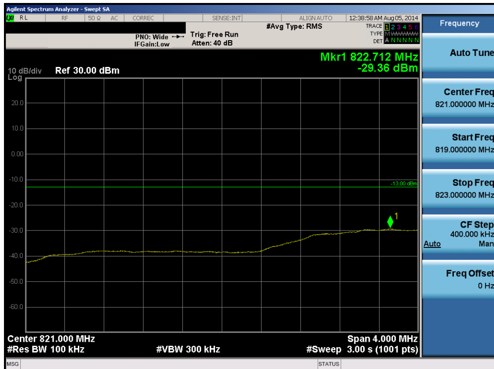
Plot 6-57. Lower Extended Band Edge Plot (Band 26 - 3.0MHz QPSK - RB Size 15)
