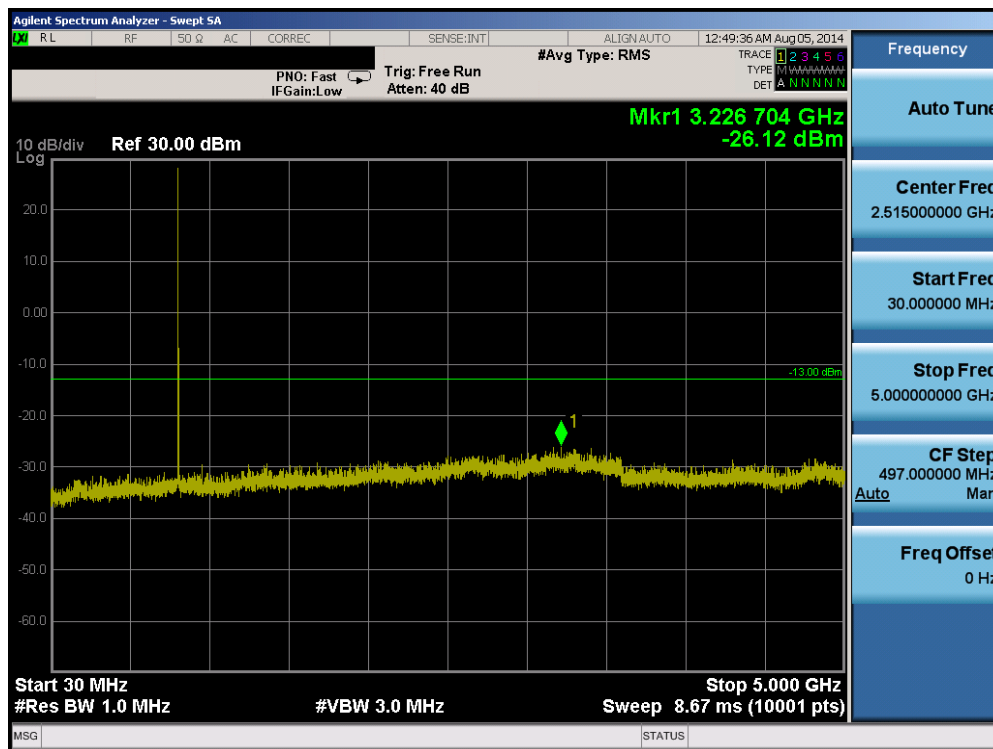
Plot 6-29. Conducted Spurious Plot (Band 26 – 5.0MHz QPSK – RB Size 1, RB Offset 0 – Low Channel)
