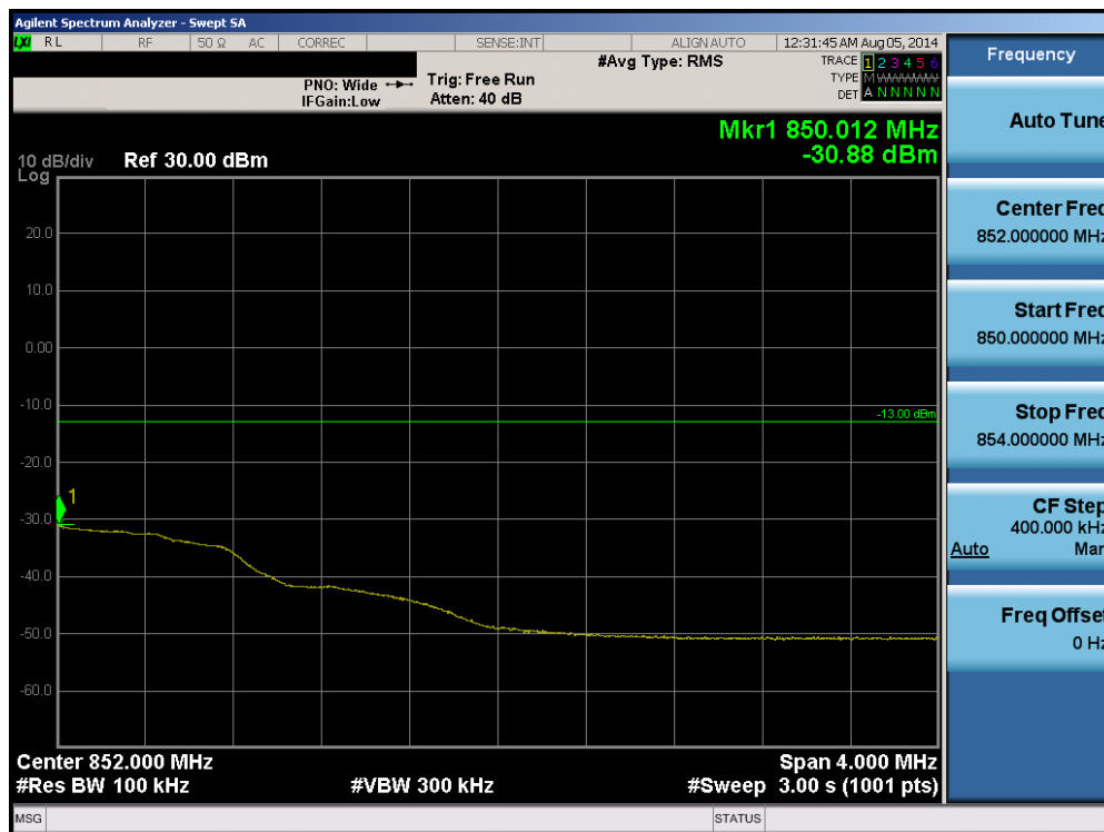
Plot 6-55. Upper Extended Band Edge Plot (Band 26 – 1.4MHz QPSK – RB Size 6)
