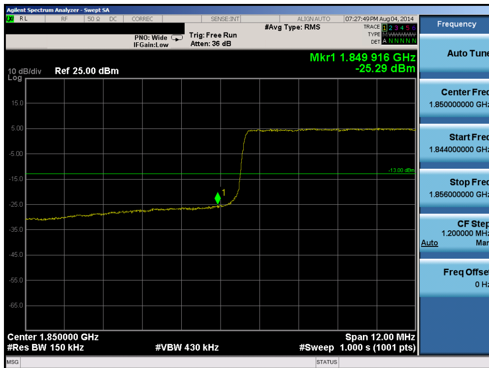
Plot 6-83. Lower Band Edge Plot (Band 25 - 15.0MHz QPSK - RB Size 75)
