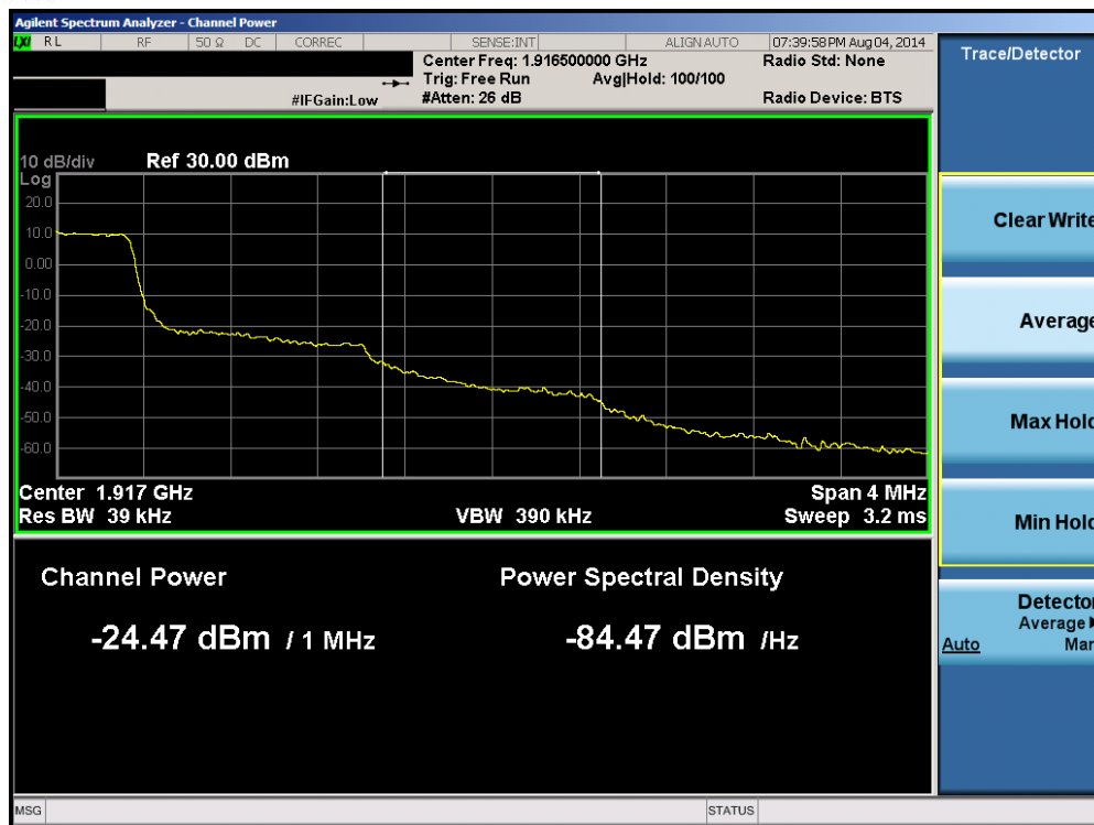
Plot 6-70. Upper Extended Band Edge Plot (Band 25 – 1.4MHz QPSK – RB Size 6)
