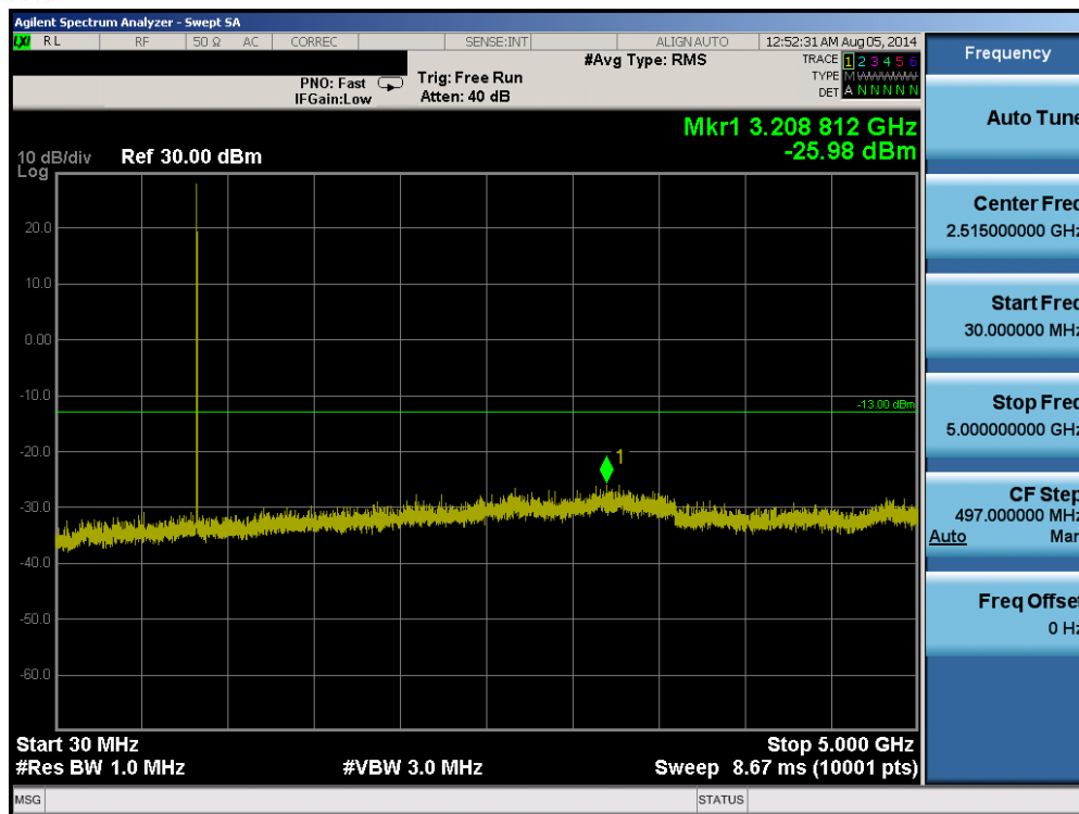
Plot 6-33. Conducted Spurious Plot (Band 26 – 5.0MHz QPSK – RB Size 1, RB Offset 0 – High Channel)
