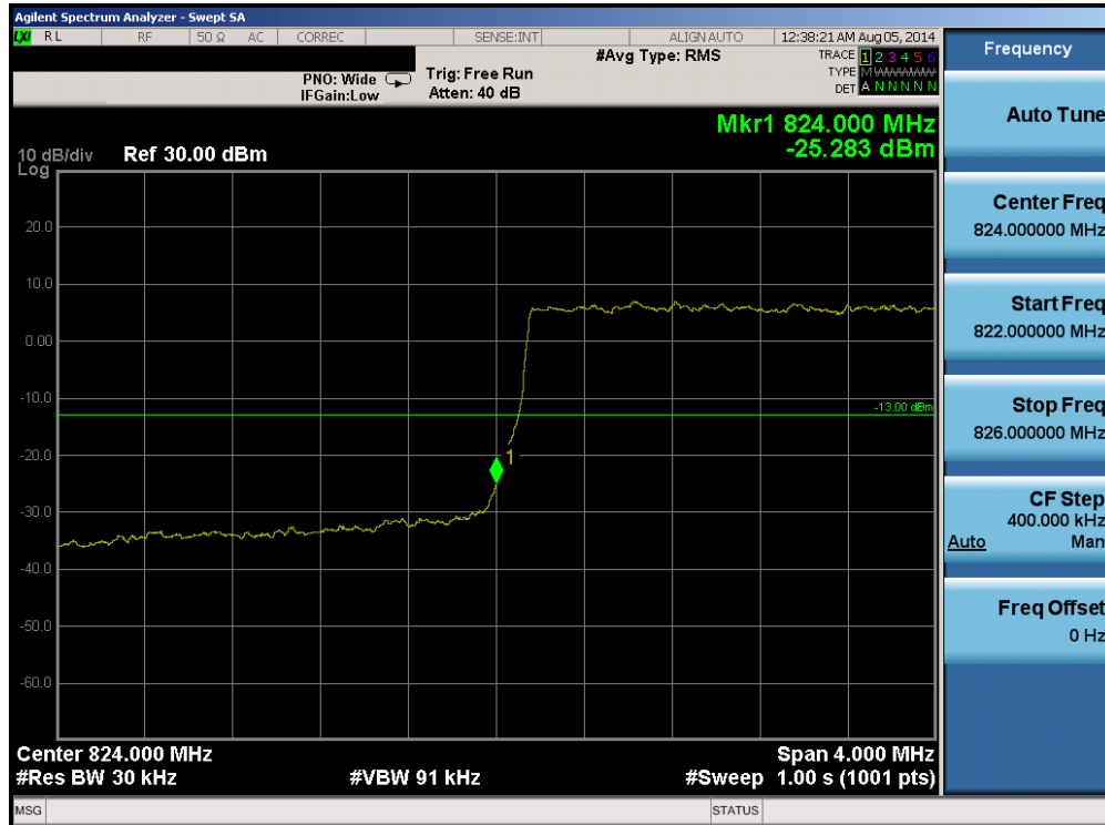
Plot 6-56. Lower Band Edge Plot (Band 26 - 3.0MHz QPSK - RB Size 15)
