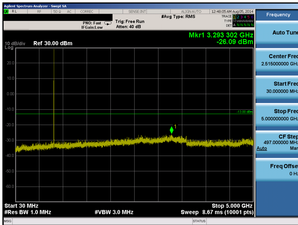
Plot 6-31. Conducted Spurious Plot (Band 26 – 5.0MHz QPSK – RB Size 1, RB Offset 0 – Mid Channel)
