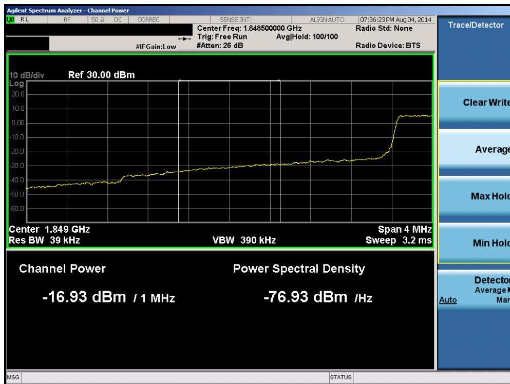
Plot 6-72. Lower Extended Band Edge Plot (Band 25 – 3.0MHz QPSK – RB Size 15)
