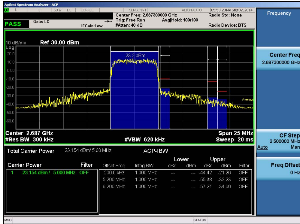
Plot 6-94. Upper-2 ACP Plot (Band 41 – 5.0MHz QPSK – RB Size 25)
