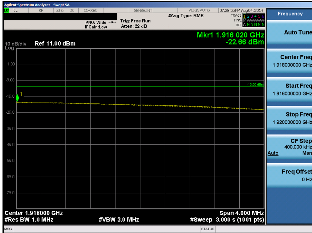
Plot 6-86. Upper Extended Band Edge Plot (Band 25 - 15.0MHz QPSK - RB Size 75)
