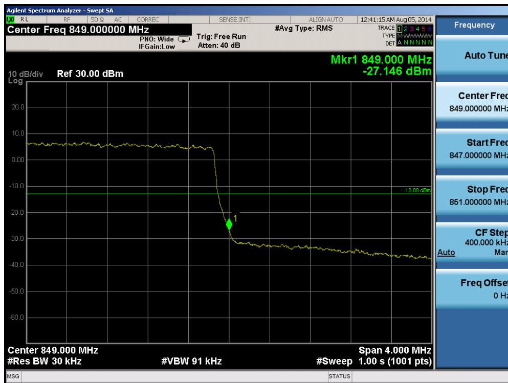
Plot 6-58. Upper Band Edge Plot (Band 26 – 3.0MHz QPSK – RB Size 15)
