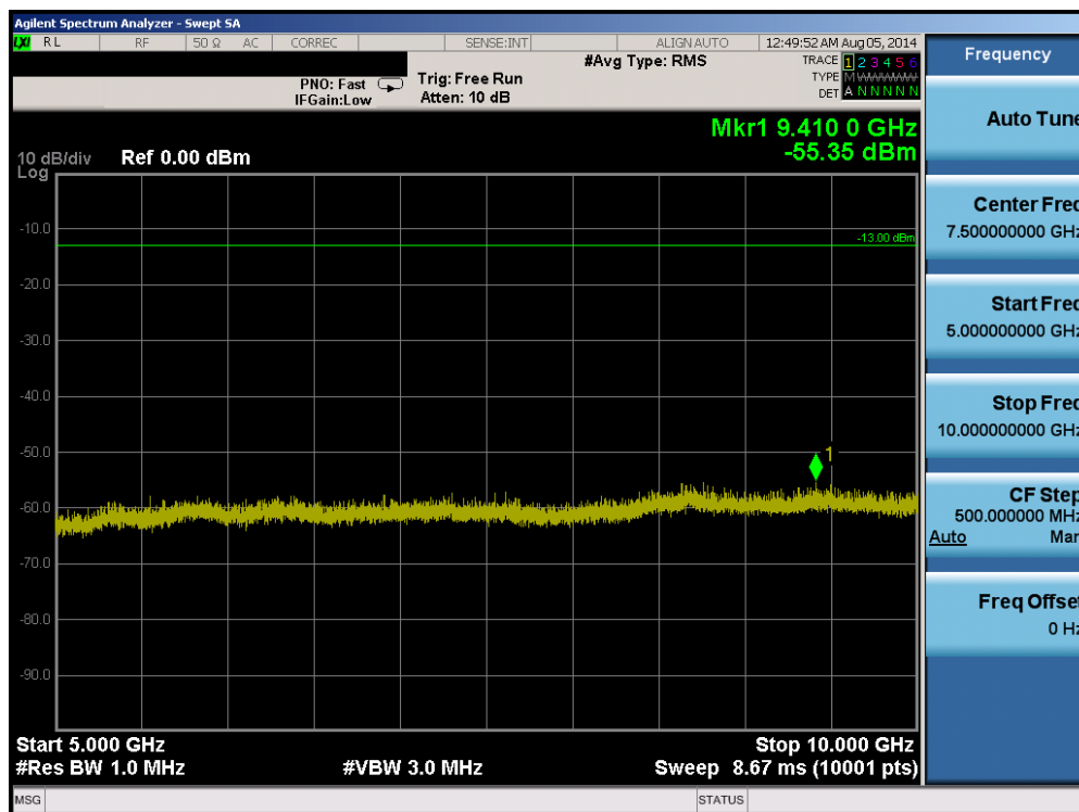
Plot 6-30. Conducted Spurious Plot (Band 26 – 5.0MHz QPSK – RB Size 1, RB Offset 0 – Low Channel)
