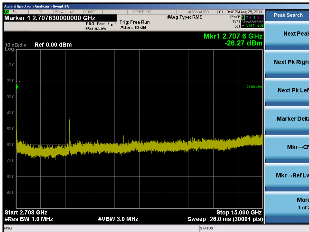
Plot 6-48. Conducted Spurious Plot (Band 41 – 15.0MHz QPSK – RB Size 75, RB Offset 0 – High Channel)
