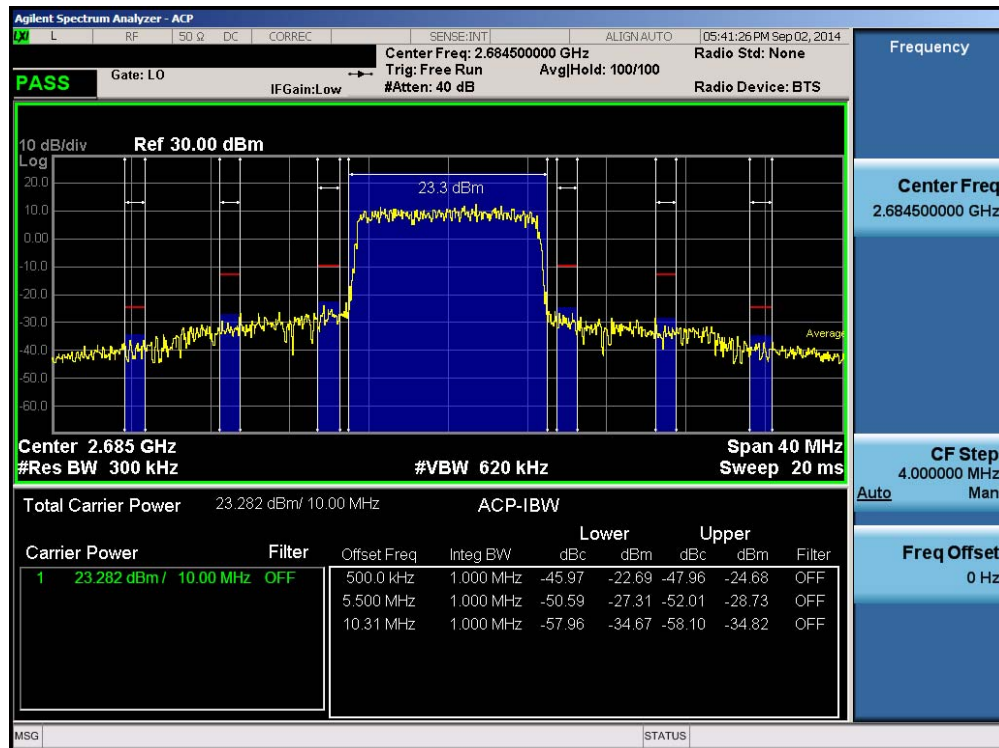
Plot 6-97. Upper ACP Plot (Band 41 – 10.0MHz QPSK – RB Size 50)
