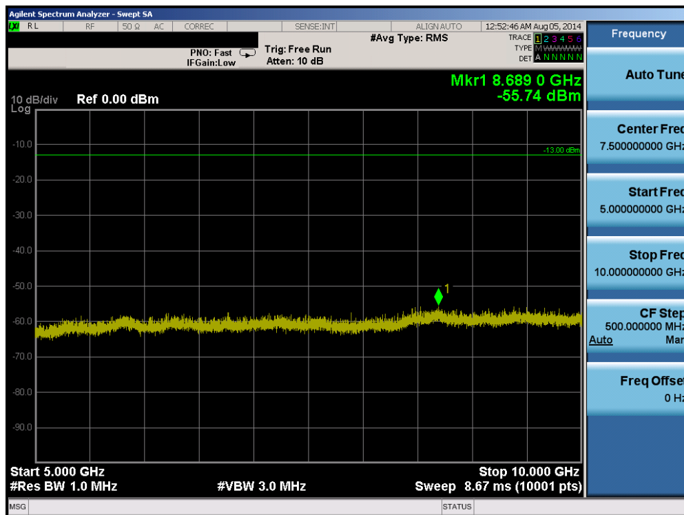
Plot 6-34. Conducted Spurious Plot (Band 26 – 5.0MHz QPSK – RB Size 1, RB Offset 0 – High Channel)
