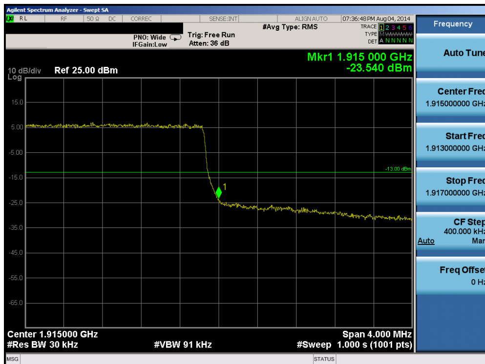
Plot 6-73. Upper Band Edge Plot (Band 25 – 3.0MHz QPSK – RB Size 15)
