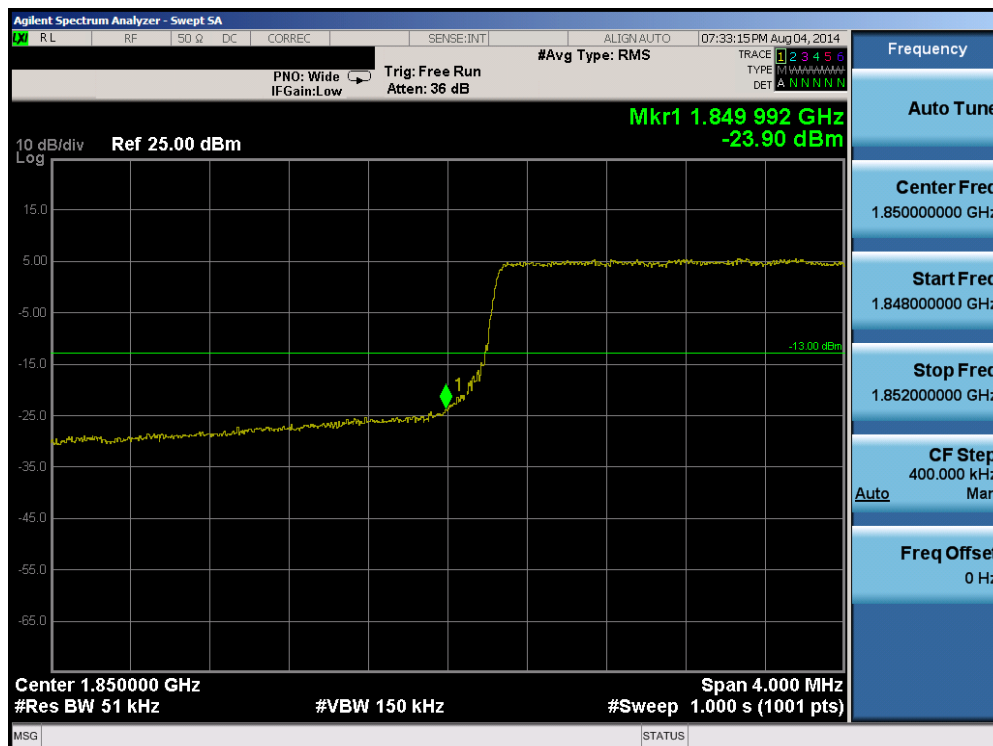
Plot 6-75. Lower Band Edge Plot (Band 25 – 5.0MHz QPSK – RB Size 25)
