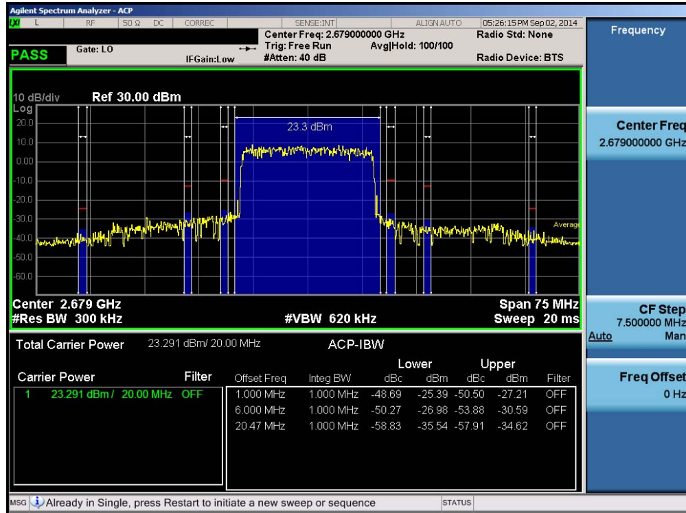
Plot 6-104. Upper ACP Plot (Band 41 – 20.0MHz QPSK – RB Size 100)
