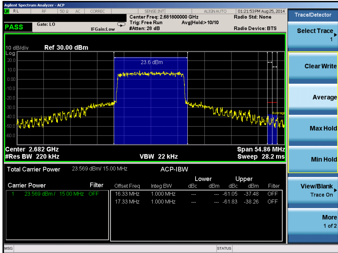
Plot 6-51. Conducted Spurious Plot (Band 41 – 15.0MHz QPSK – RB Size 75, RB Offset 0 – High Channel)
