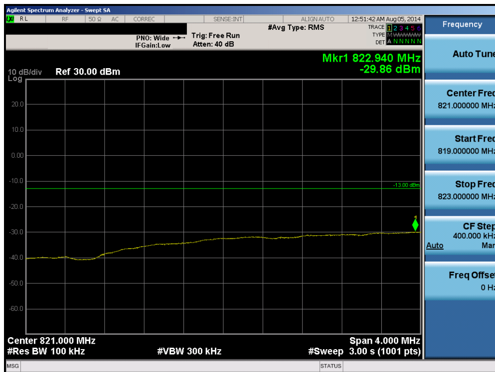
Plot 6-61. Lower Extended Band Edge Plot (Band 26 – 5.0MHz QPSK – RB Size 25)
