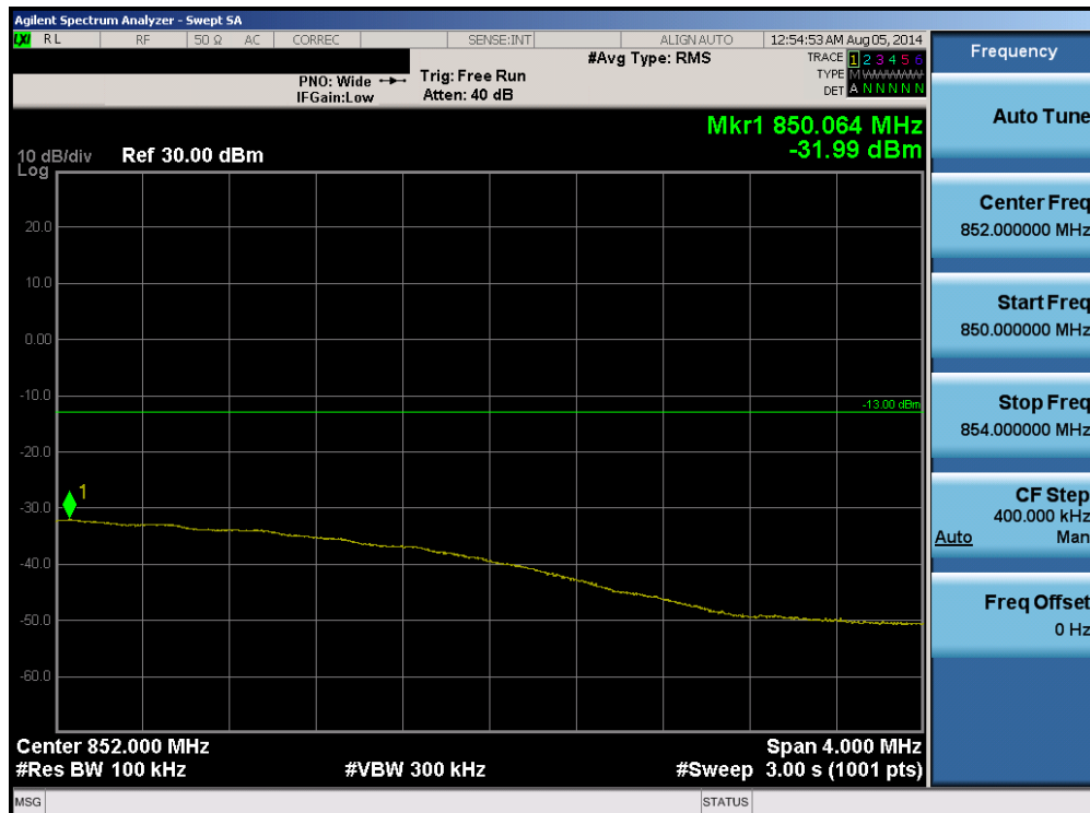
Plot 6-63. Upper Extended Band Edge Plot (Band 26 – 5.0MHz QPSK – RB Size 25)
