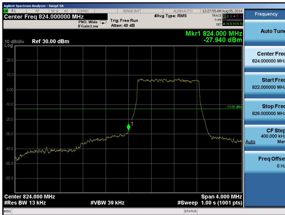
Plot 6-52. Lower Band Edge Plot (Band 26 – 1.4MHz QPSK – RB Size 6)
