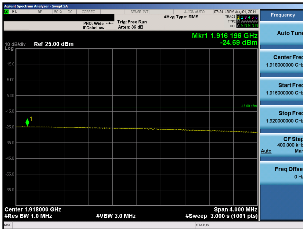
Plot 6-90. Upper Extended Band Edge Plot (Band 25 – 20.0MHz QPSK – RB Size 100)
