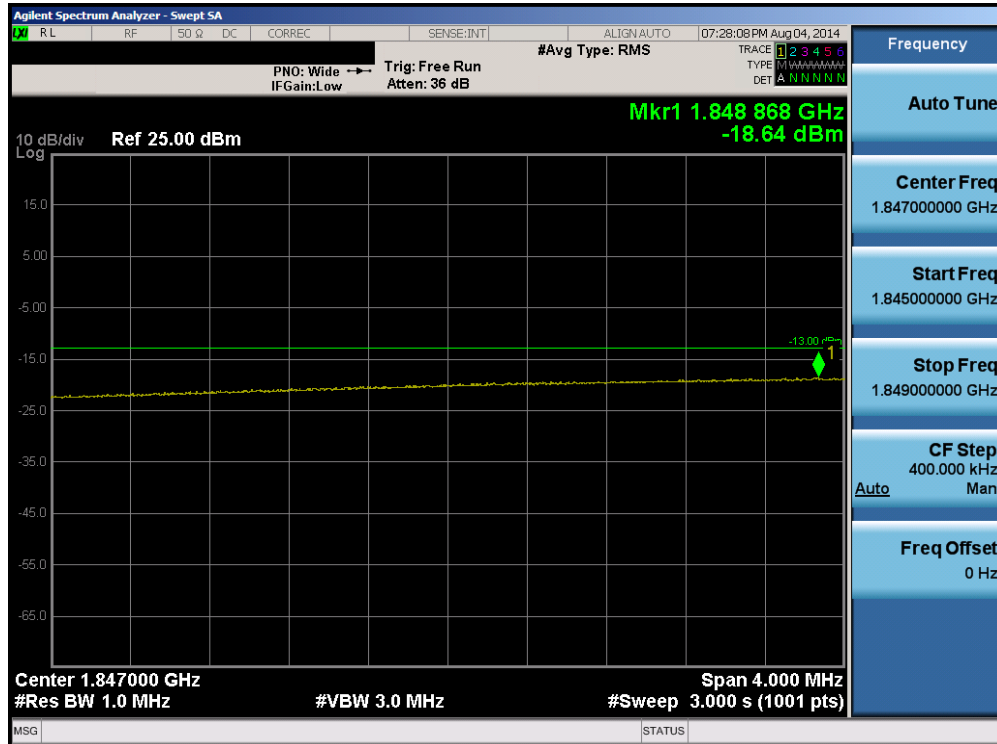
Plot 6-84. Lower Extended Band Edge Plot (Band 25 – 15.0MHz QPSK – RB Size 75)
