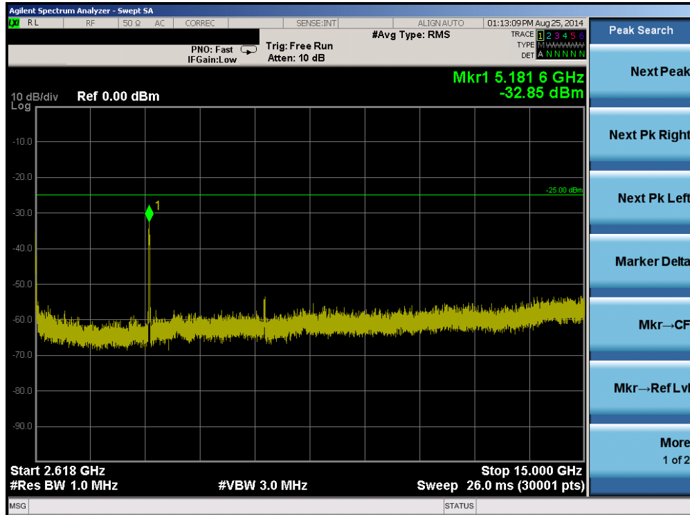
Plot 6-45. Conducted Spurious Plot (Band 41 – 15.0MHz QPSK – RB Size 75, RB Offset 0 – Mid Channel)
