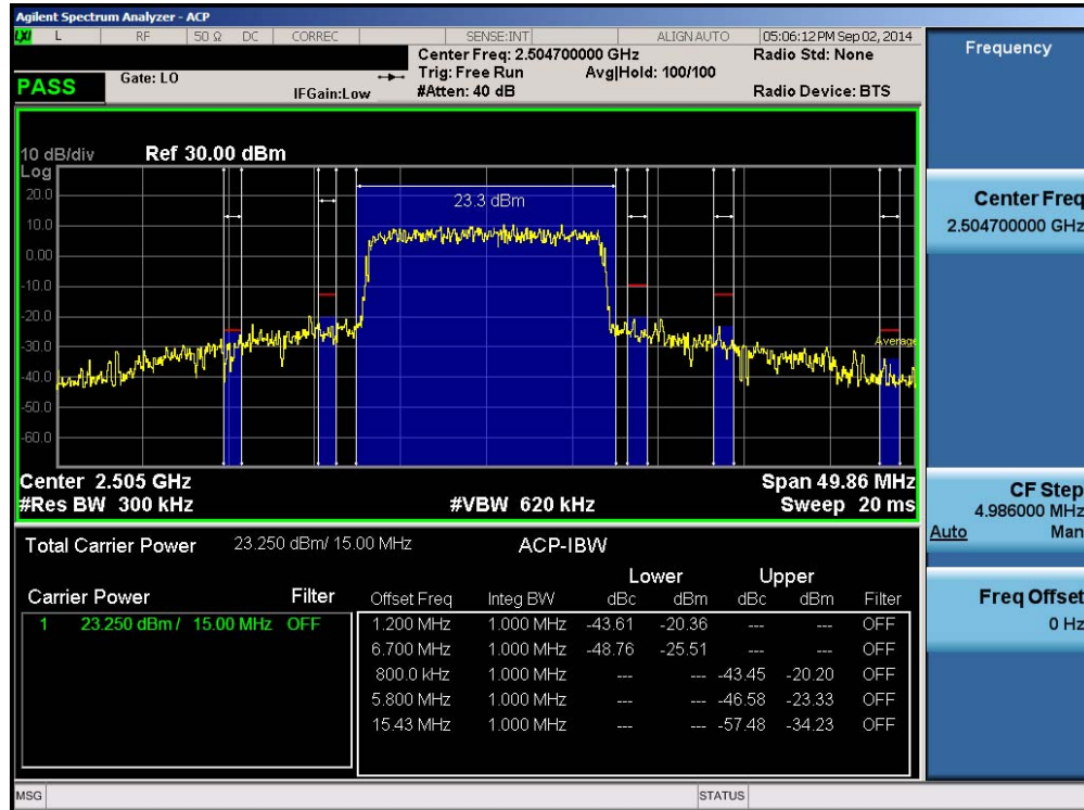
Plot 6-98. Lower ACP Plot (Band 41 – 15.0MHz QPSK – RB Size 75)
