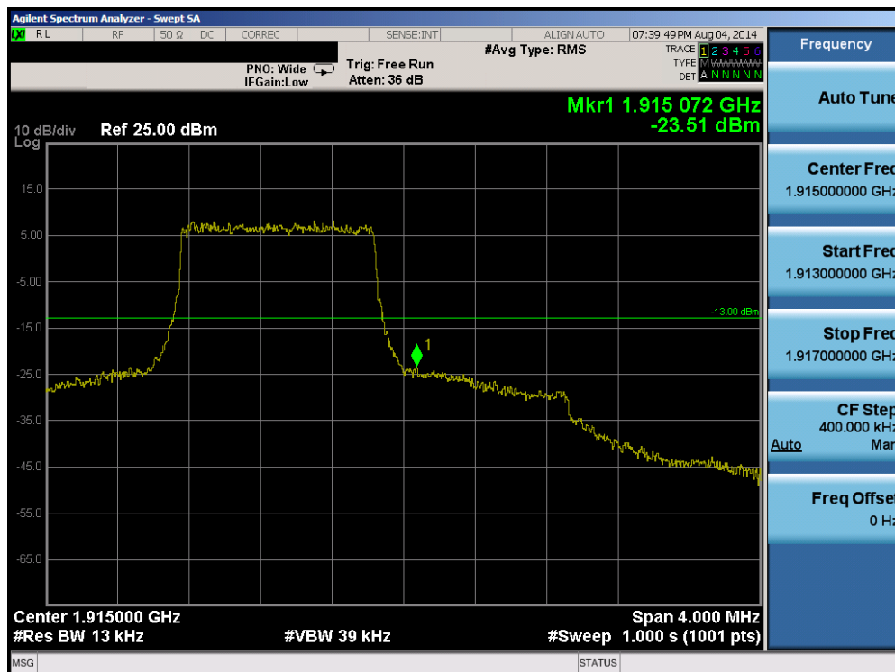
Plot 6-69. Upper Band Edge Plot (Band 25 – 1.4MHz QPSK – RB Size 6)
