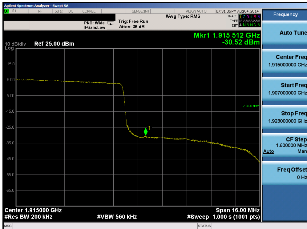
Plot 6-89. Upper Band Edge Plot (Band 25 – 20.0MHz QPSK – RB Size 100)
