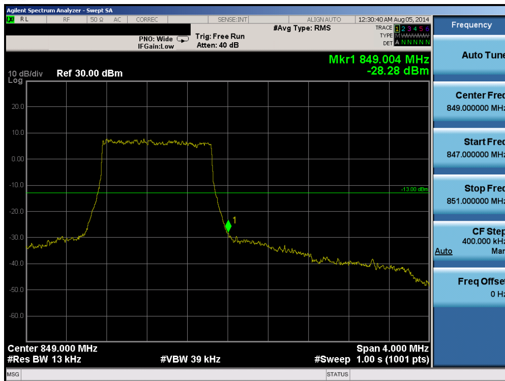
Plot 6-54. Upper Band Edge Plot (Band 26 – 1.4MHz QPSK – RB Size 6)
