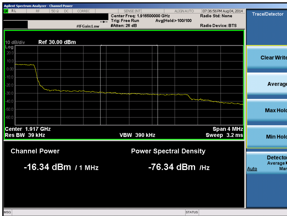
Plot 6-74. Upper Extended Band Edge Plot (Band 25 – 3.0MHz QPSK – RB Size 15)
