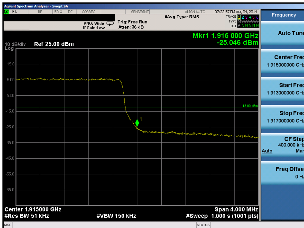
Plot 6-77. Upper Band Edge Plot (Band 25 – 5.0MHz QPSK – RB Size 25)
