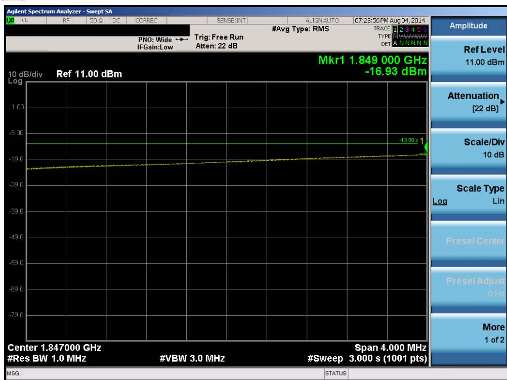
Plot 6-80. Lower Extended Band Edge Plot (Band 25 - 10.0MHz QPSK - RB Size 50)
