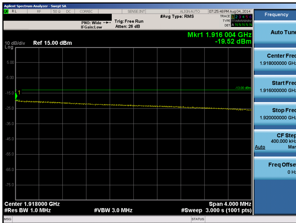
Plot 6-82. Upper Extended Band Edge Plot (Band 25 - 10.0MHz QPSK - RB Size 50)
