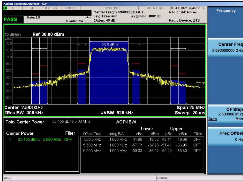
Plot 6-92. Mid ACP Plot (Band 41 – 5.0MHz QPSK – RB Size 25)
