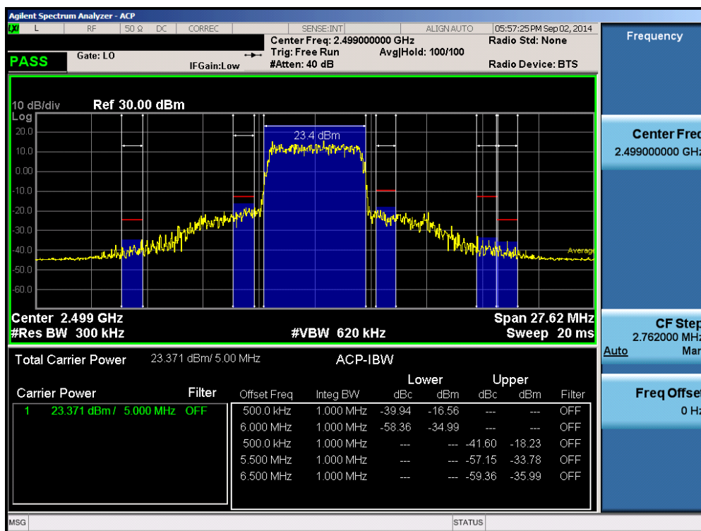
Plot 6-91. Lower ACP Plot (Band 41 – 5.0MHz QPSK – RB Size 25)
