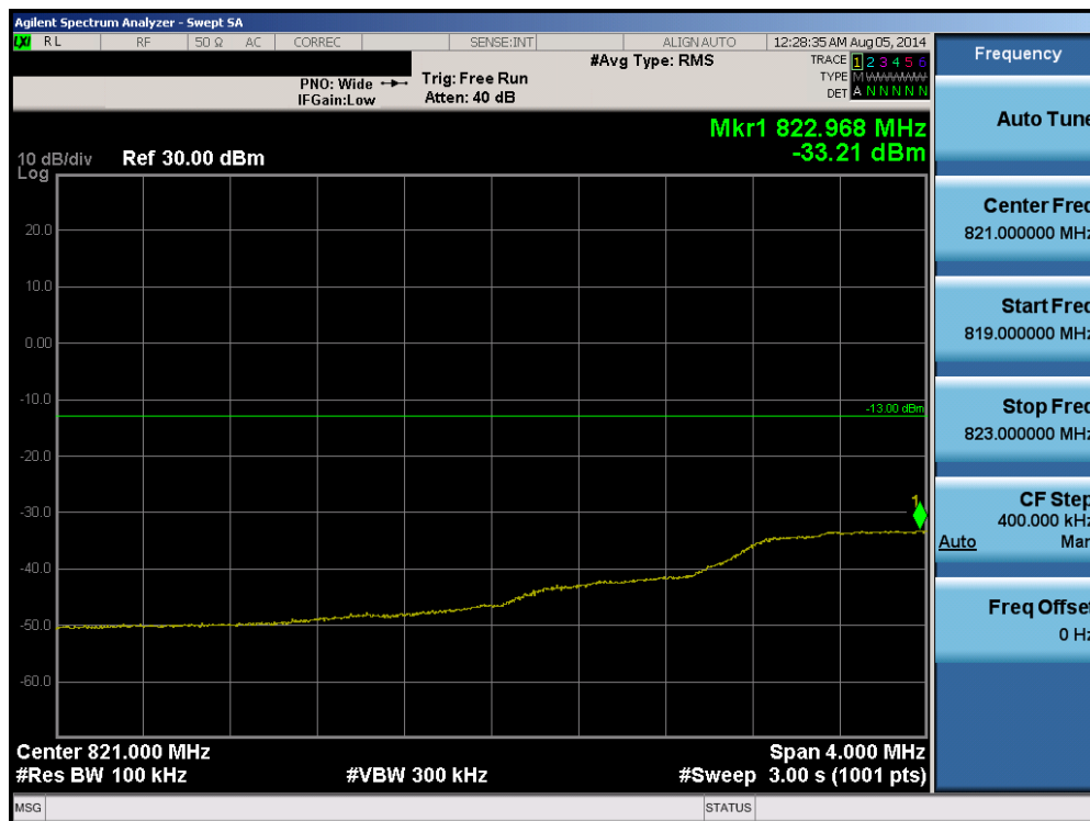
Plot 6-53. Lower Extended Band Edge Plot (Band 26 – 1.4MHz QPSK – RB Size 6)
