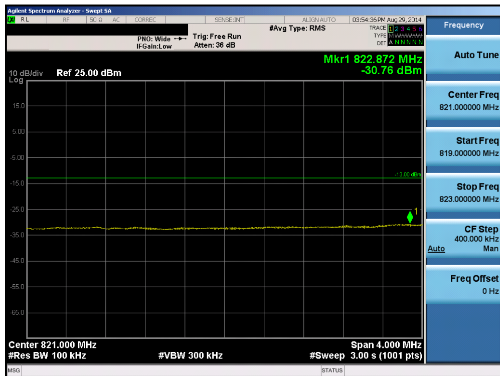
Plot 6-65. Lower Extended Band Edge Plot (Band 26 – 10.0MHz QPSK – RB Size 50)
