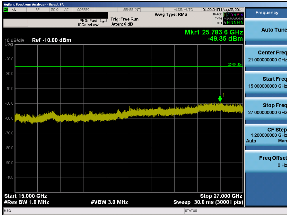
Plot 6-49. Conducted Spurious Plot (Band 41 – 15.0MHz QPSK – RB Size 75, RB Offset 0 – High Channel)
