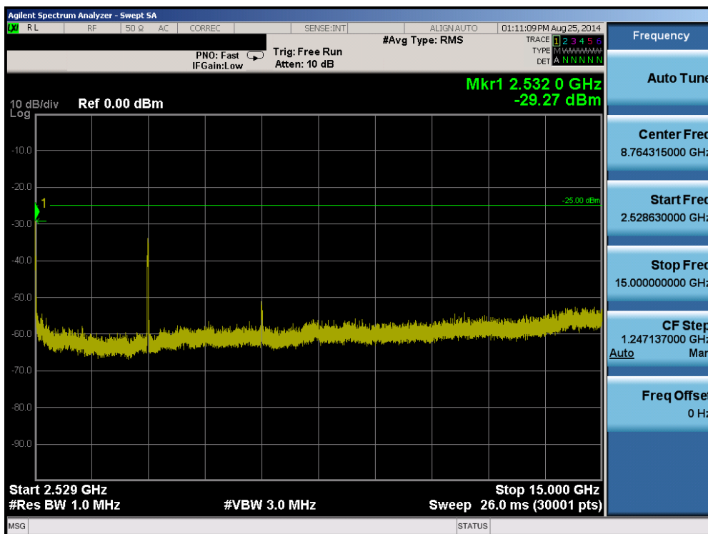
Plot 6-42. Conducted Spurious Plot (Band 41 – 15.0MHz QPSK – RB Size 75, RB Offset 0 – Low Channel)
