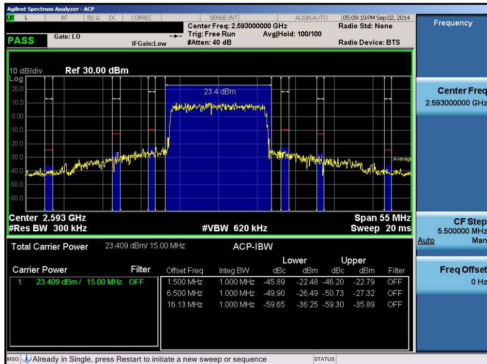
Plot 6-99. Mid ACP Plot (Band 41 – 15.0MHz QPSK – RB Size 75)
