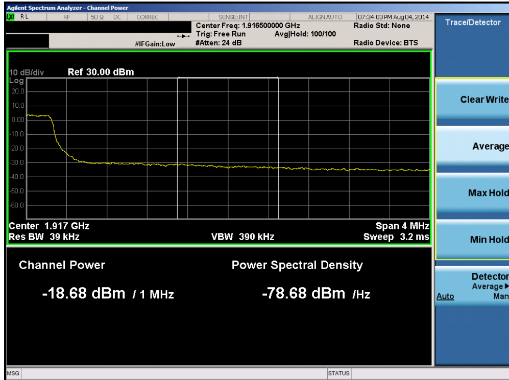
Plot 6-78. Upper Extended Band Edge Plot (Band 25 – 5.0MHz QPSK – RB Size 25)
