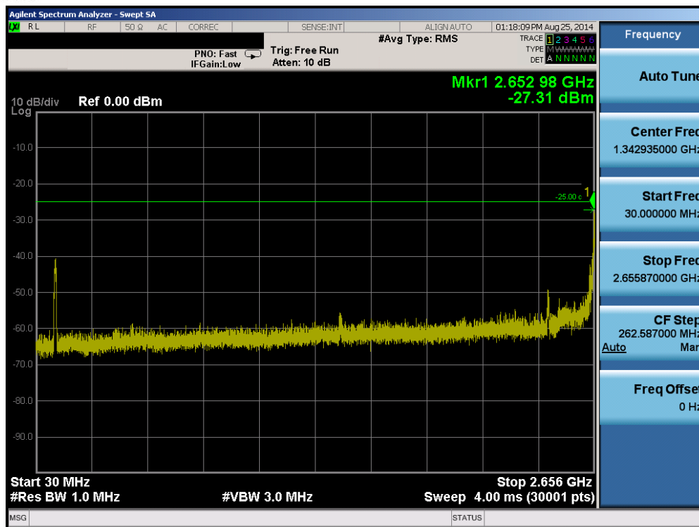
Plot 6-47. Conducted Spurious Plot (Band 41 – 15.0MHz QPSK – RB Size 75, RB Offset 0 – High Channel)
