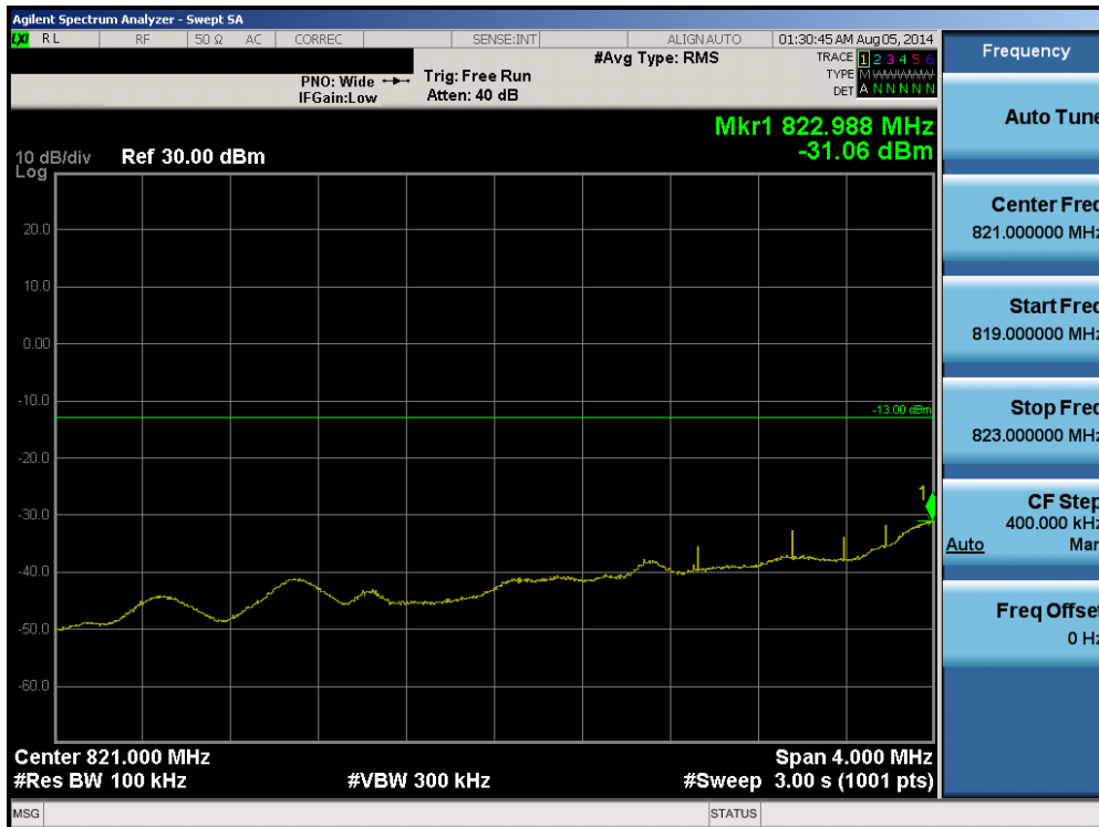
Plot 6-53. 4MHz Span Plot (Cellular CDMA Mode – Ch. 1013)
