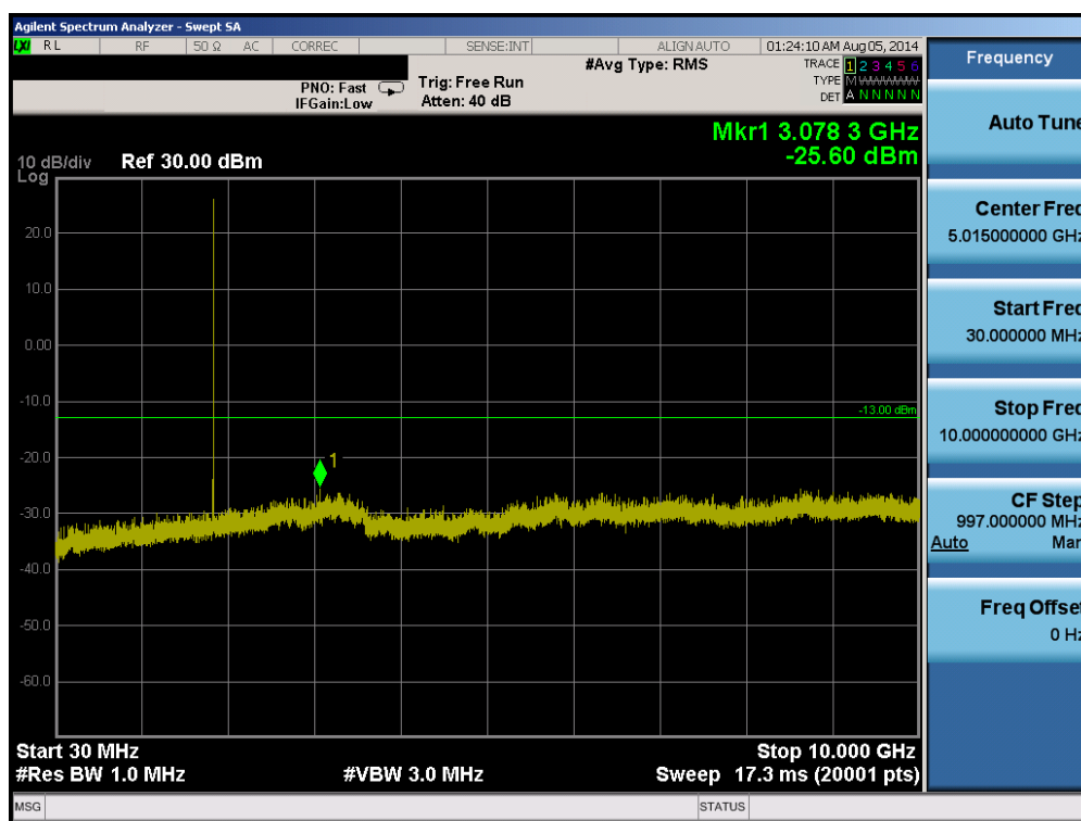
Plot 6-30. Conducted Spurious Plot (PCS CDMA Mode – Ch. 25)
