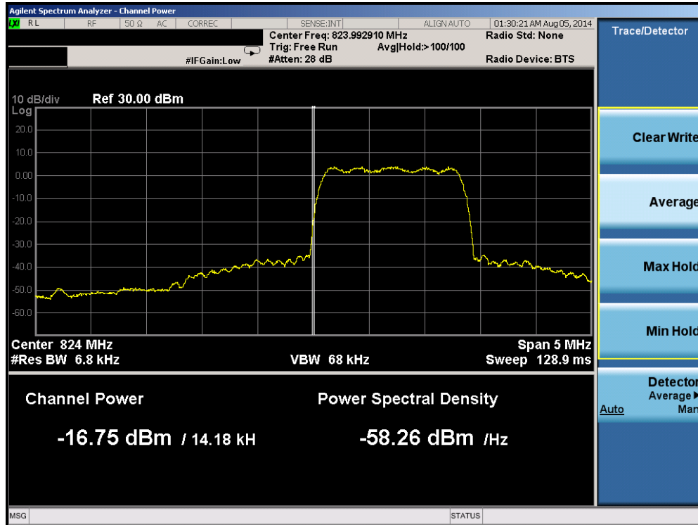
Plot 6-52. Band Edge Plot (Cellular CDMA Mode – Ch. 1013)
