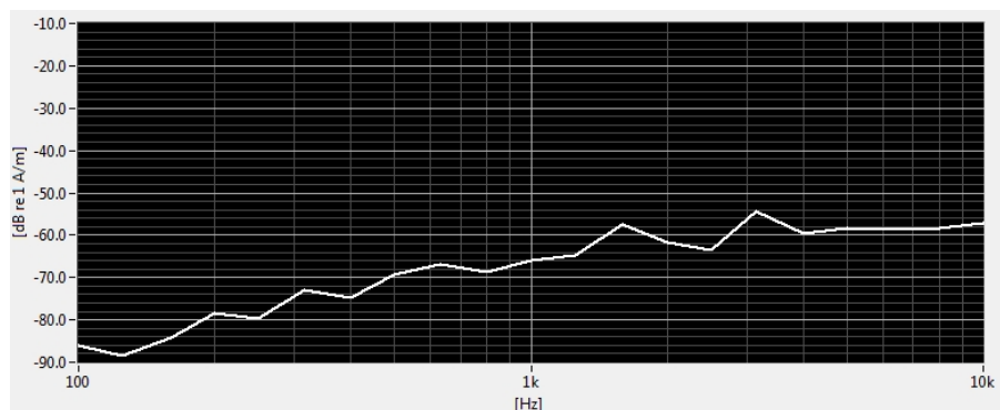
Figure 7-4 Worst-case ABM2 Plot for WD, UMTS
