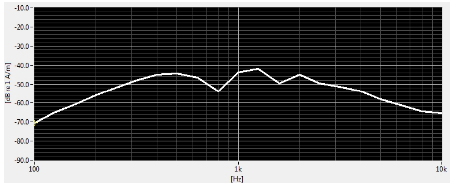
Figure 7-2 Worst-case ABM2 Plot for WD, CDMA
