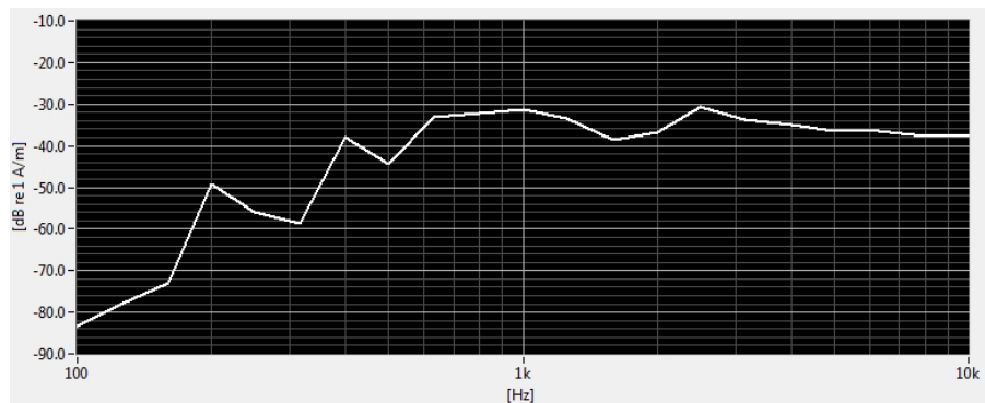
Figure 7-3 Worst-case ABM2 Plot for WD, GSM
