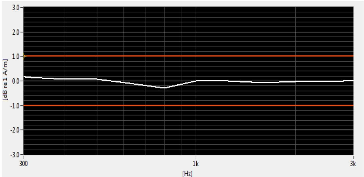
Figure 7-5 Helmholtz Coil Validation for Frequency Response
