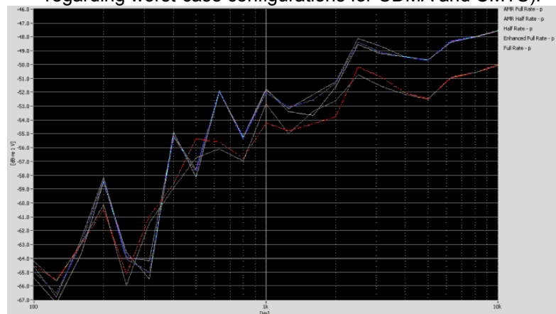
Figure 5-12 Vocoder Analysis for ABM Noise
