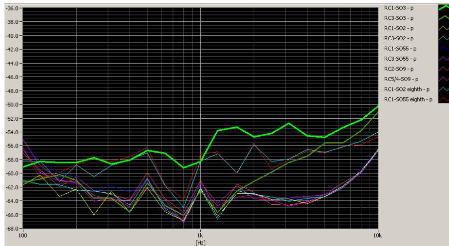
Figure 6-1 CDMA Audio Band Magnetic Noise
