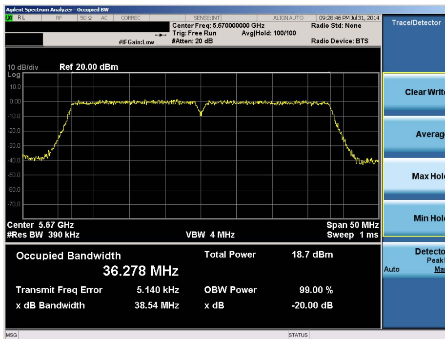
Plot 6-33. 20dB Bandwidth Plot (40MHz BW 802.11n (UNII Band 2C) – Ch. 134)
