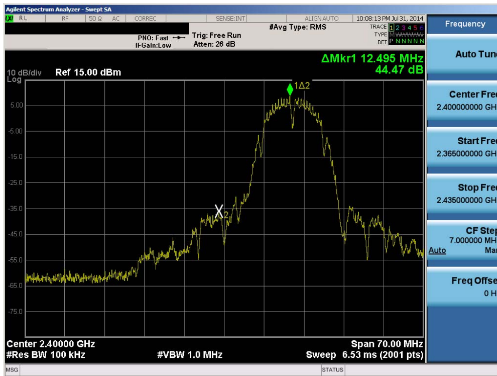
Plot 6-86. Band Edge Plot (802.11b – Ch. 1)
