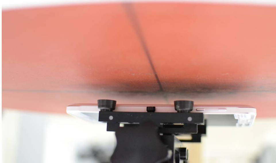
SAR Test Setup Photo 7: Back Side at 15mm, Standard Back Cover
