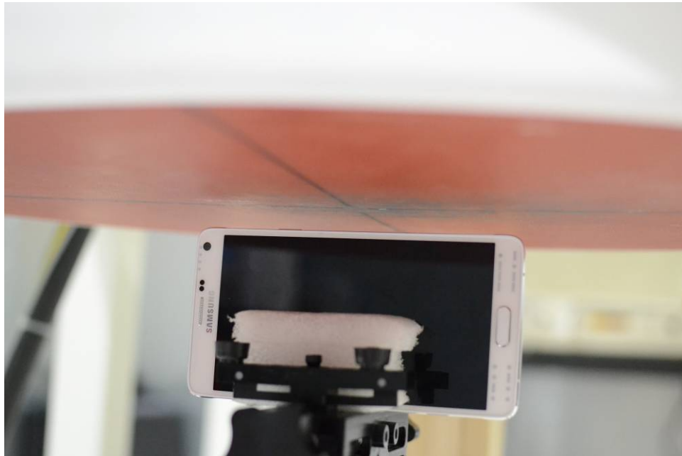
SAR Test Setup Photo 22: Right Edge at 10mm, Standard Back Cover
