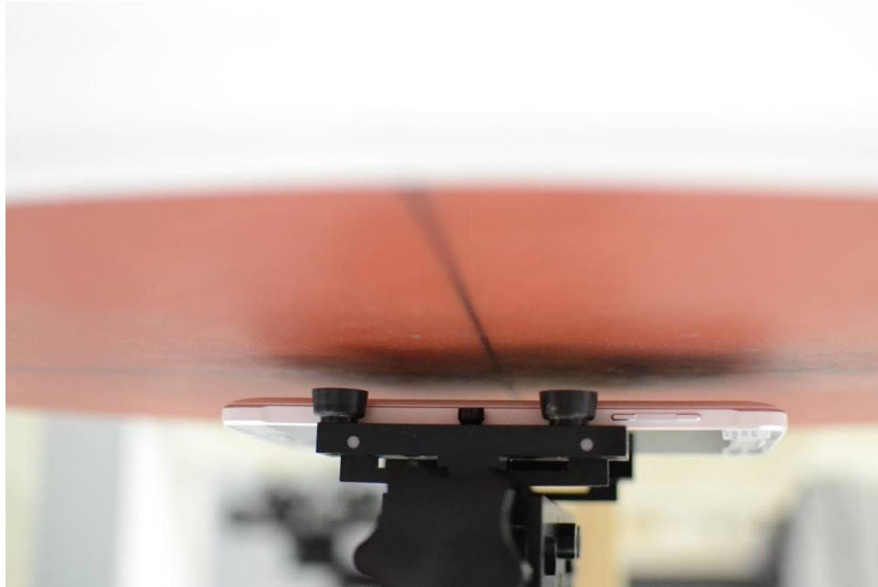
SAR Test Setup Photo 9: Back Side at 10mm, Standard Back Cover
