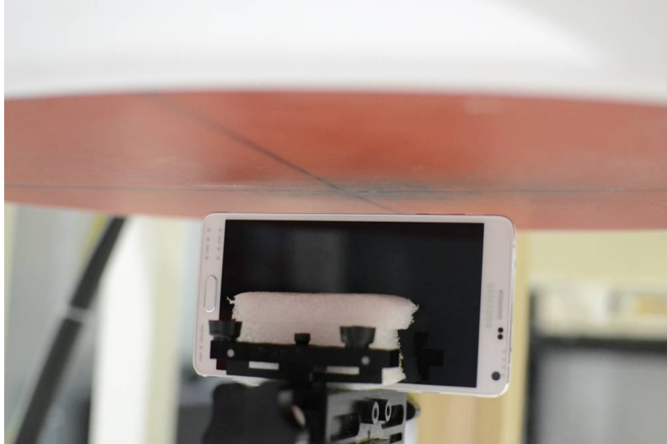
SAR Test Setup Photo 23: Left Edge at 10mm, Standard Back Cover
