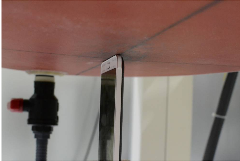
SAR Test Setup Photo 21 – Bottom Edge at 0.0 cm, Wireless Charging Cover
