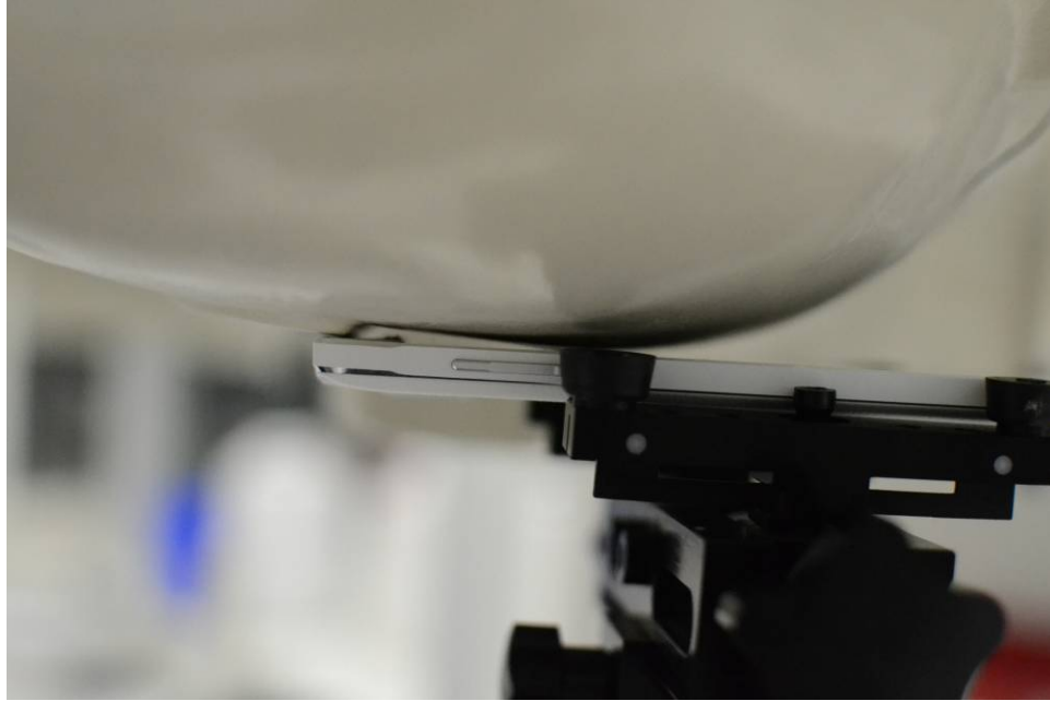
SAR Test Setup Photo 1: Right Cheek, Standard Back Cover
