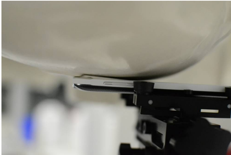
SAR Test Setup Photo 2: Right Cheek, Wireless Charging Cover
