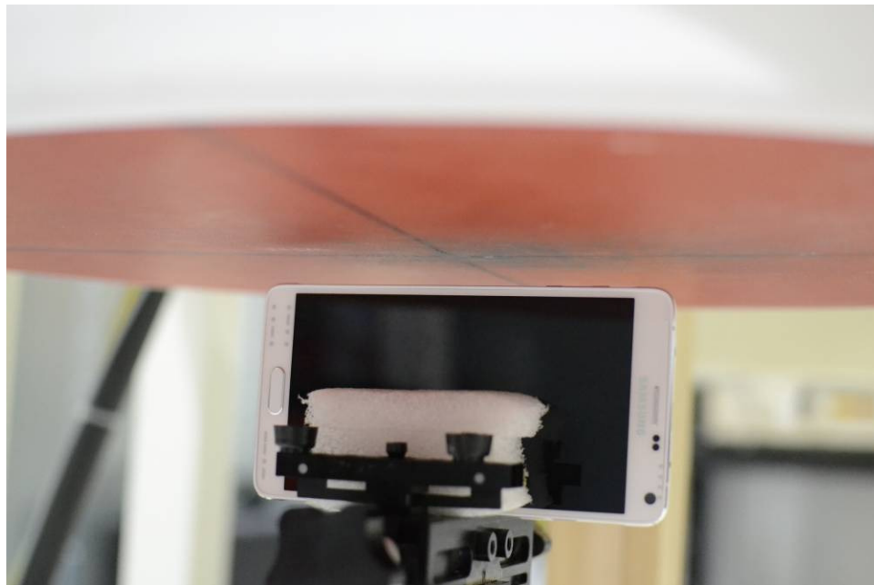
SAR Test Setup Photo 12: Left Edge at 10mm, Standard Back Cover
