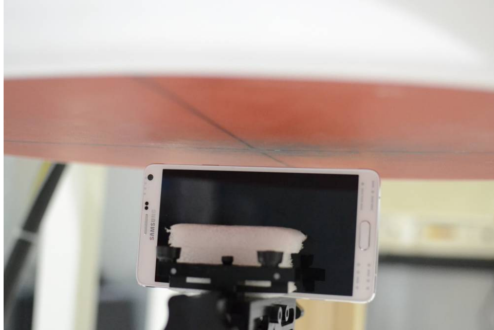
SAR Test Setup Photo 11: Right Edge at 10mm, Standard Back Cover
