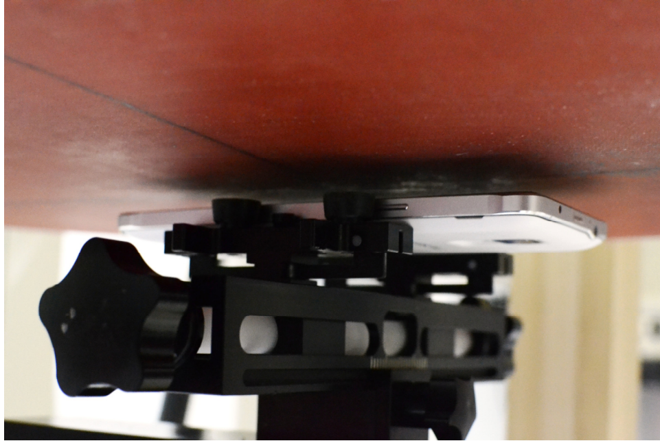
SAR Test Setup Photo 9: Front Side at 10mm, Wireless Charging Cover
