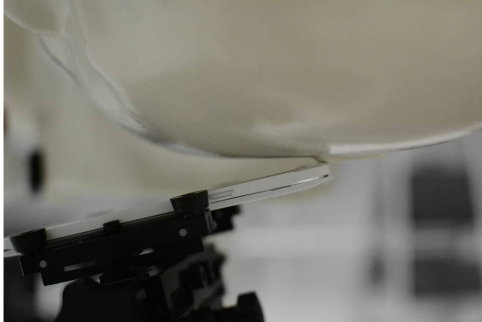
SAR Test Setup Photo 5: Left Tilt, Standard Back Cover
