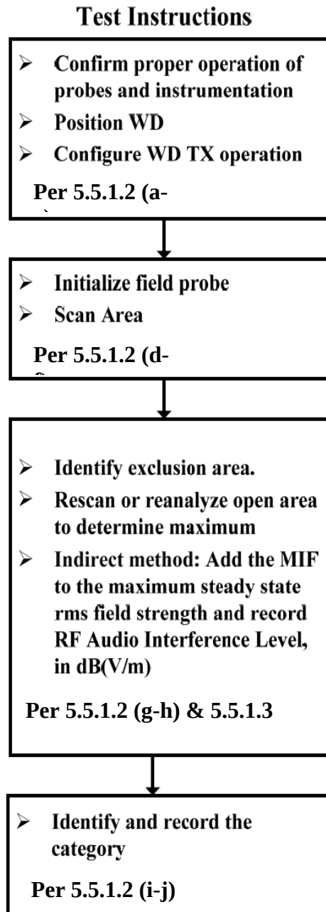
Figure 6-1 RF Emissions Flow Chart
