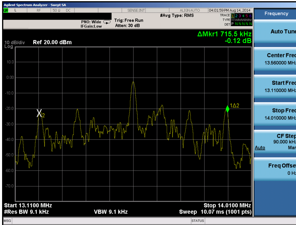
Figure 8-3. 20dB Bandwidth Plot with WCC
