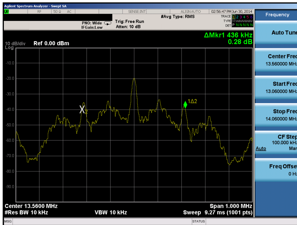
Figure 8-2. 20dB Bandwidth Plot
