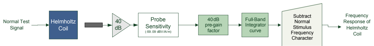
Figure 5-11 Frequency Response Block Diagram
