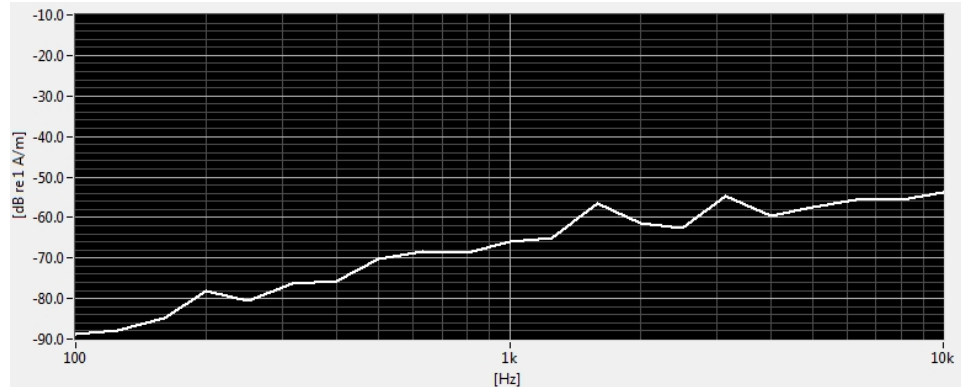
Figure 7-3 Worst-case ABM2 Plot for WD, UMTS
