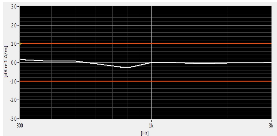
Figure 7-4 Helmholtz Coil Validation for Frequency Response
