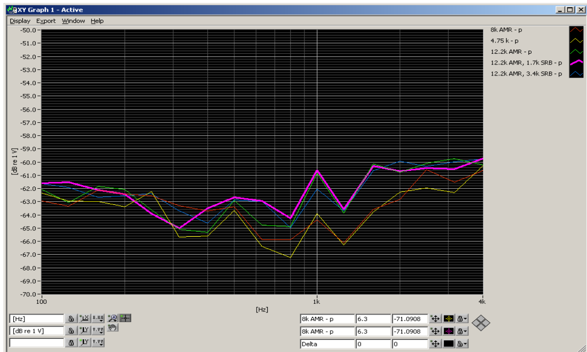
Figure 6-1 UMTS Audio Band Magnetic Noise
