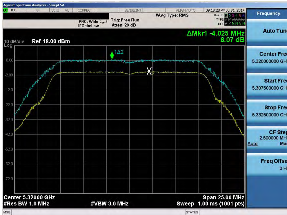
Plot 6-126. Peak Excursion Ratio Plot (20MHz BW 802.11n (UNII Band 2A) – Ch. 64)
