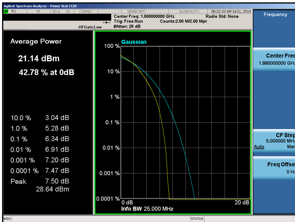
Plot 6-124. PAR Plot (Band 2 – 20.0MHz 16-QAM – RB Size 100)
