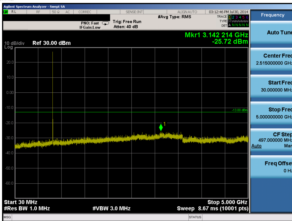
Plot 6-35. Conducted Spurious Plot (Band 5 – 1.4MHz QPSK – RB Size 1, RB Offset 0 – Mid Channel)
