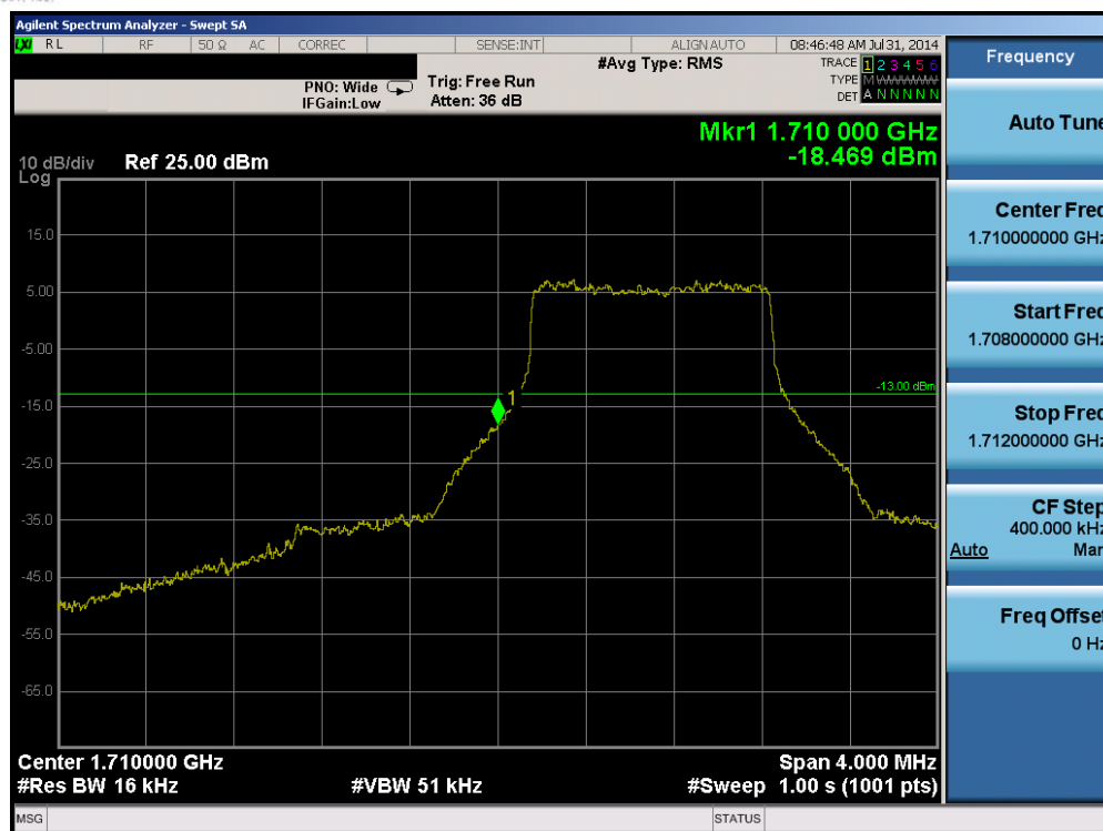
Plot 6-65. Lower Band Edge Plot (Band 4 – 1.4MHz QPSK – RB Size 6)
