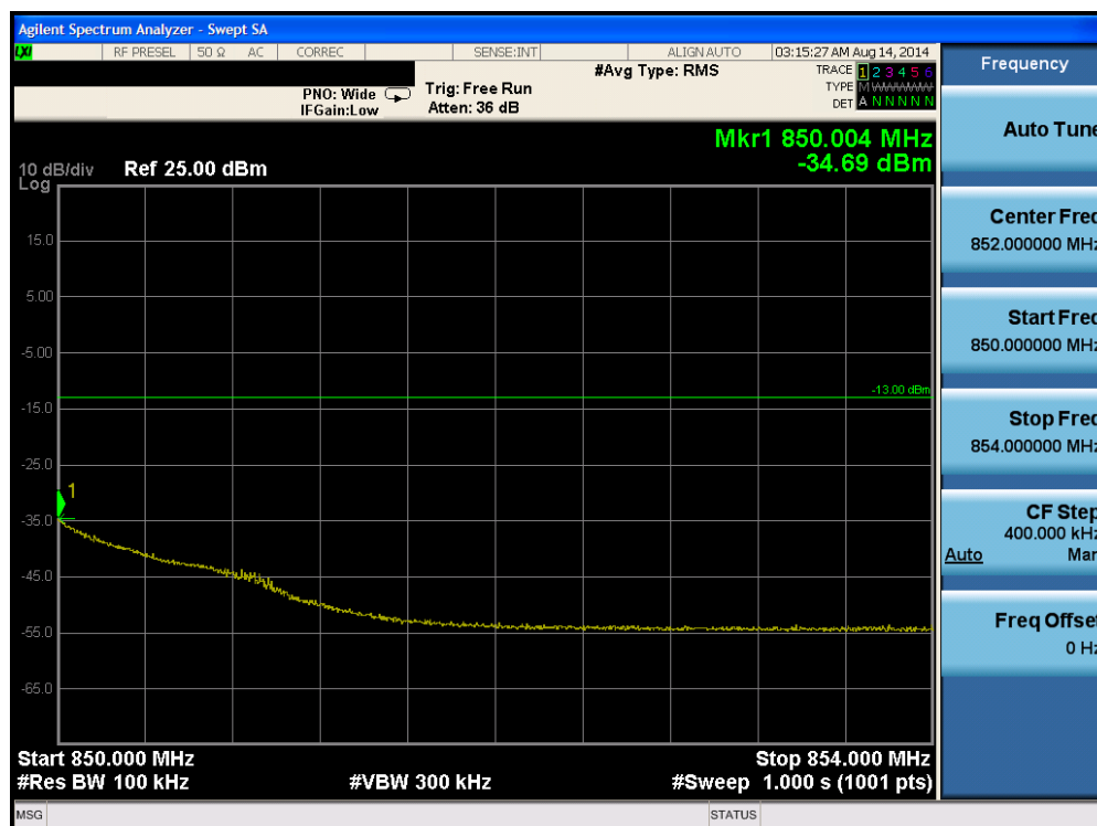
Plot 6-54. Upper Extended Band Edge Plot (Band 5 – 1.4MHz QPSK – RB Size 6)
