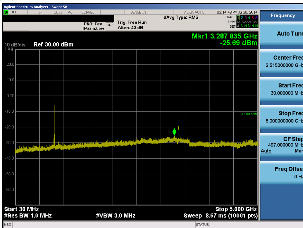
Plot 6-33. Conducted Spurious Plot (Band 5 – 1.4MHz QPSK – RB Size 1, RB Offset 0 – Low Channel)
