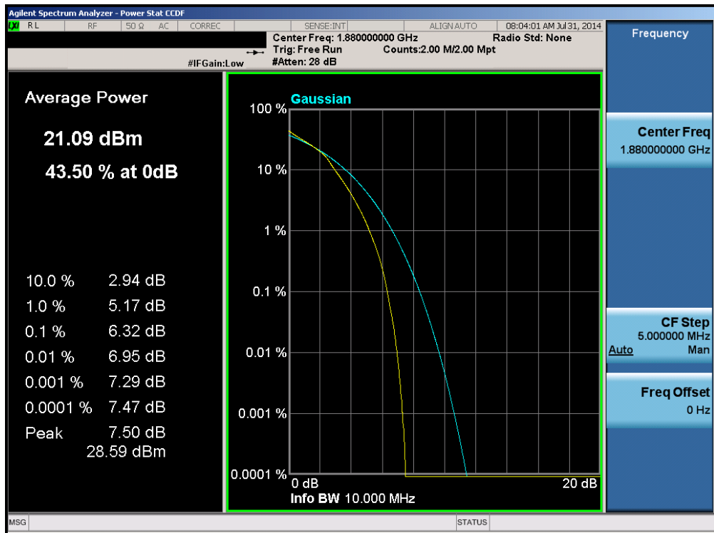
Plot 6-120. PAR Plot (Band 2 – 10.0MHz 16-QAM – RB Size 50)
