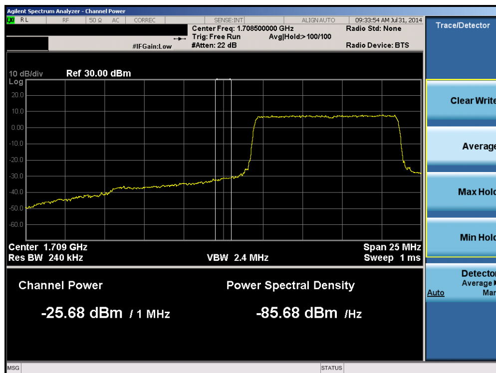
Plot 6-78. Lower Extended Band Edge Plot (Band 4 – 10.0MHz QPSK – RB Size 50)
