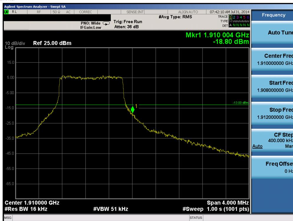
Plot 6-91. Upper Band Edge Plot (Band 2 – 1.4MHz QPSK – RB Size 6)
