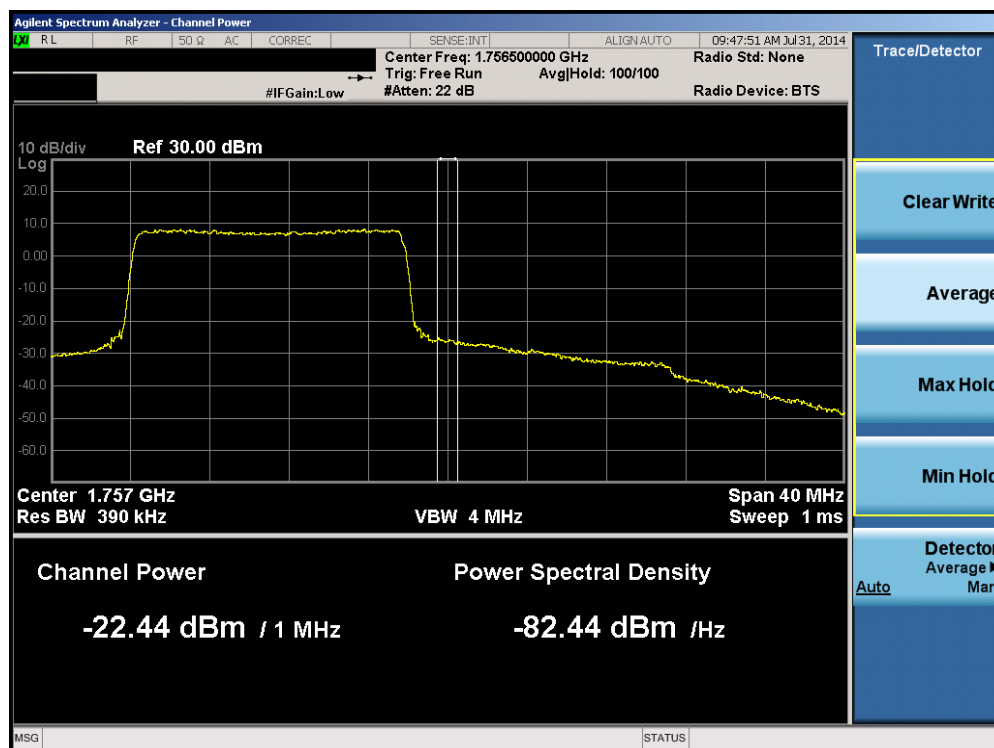
Plot 6-84. Upper Extended Band Edge Plot (Band 4 – 15.0MHz QPSK – RB Size 75)
