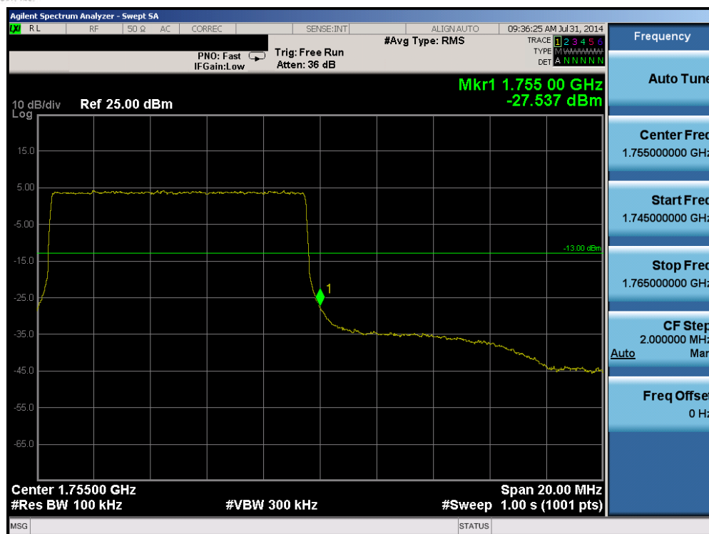
Plot 6-79. Upper Band Edge Plot (Band 4 – 10.0MHz QPSK – RB Size 50)
