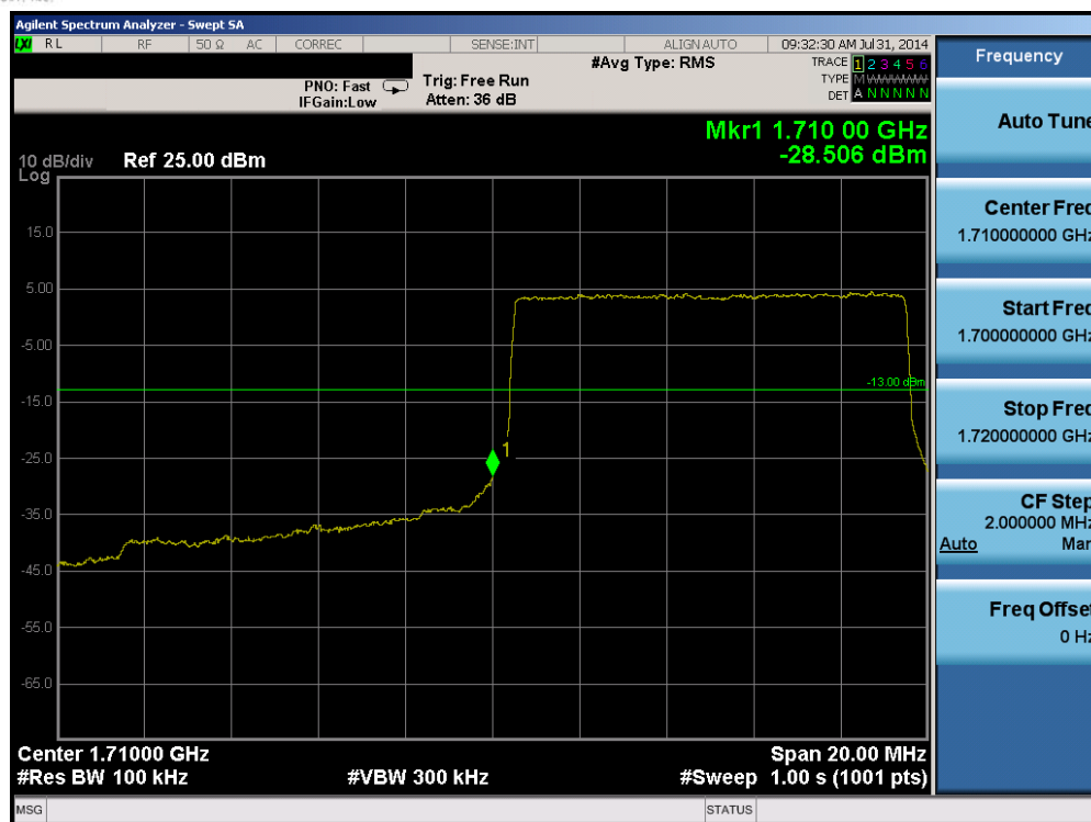
Plot 6-77. Lower Band Edge Plot (Band 4 – 10.0MHz QPSK – RB Size 50)
