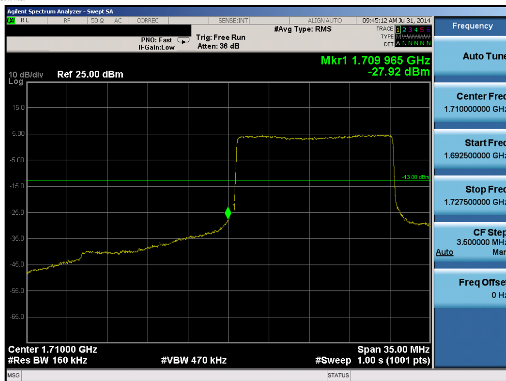
Plot 6-81. Lower Band Edge Plot (Band 4 – 15.0MHz QPSK – RB Size 75)
