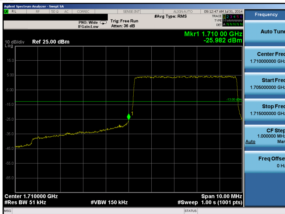
Plot 6-73. Lower Band Edge Plot (Band 4 – 5.0MHz QPSK – RB Size 25)
