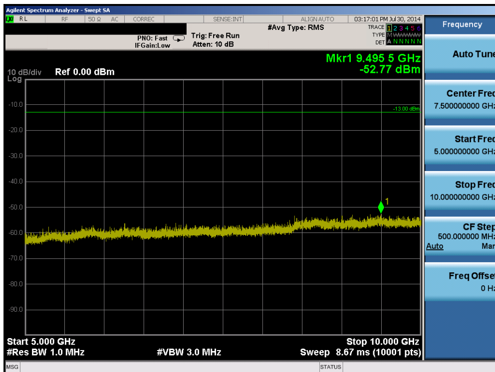
Plot 6-38. Conducted Spurious Plot (Band 5 – 1.4MHz QPSK – RB Size 1, RB Offset 0 – High Channel)
