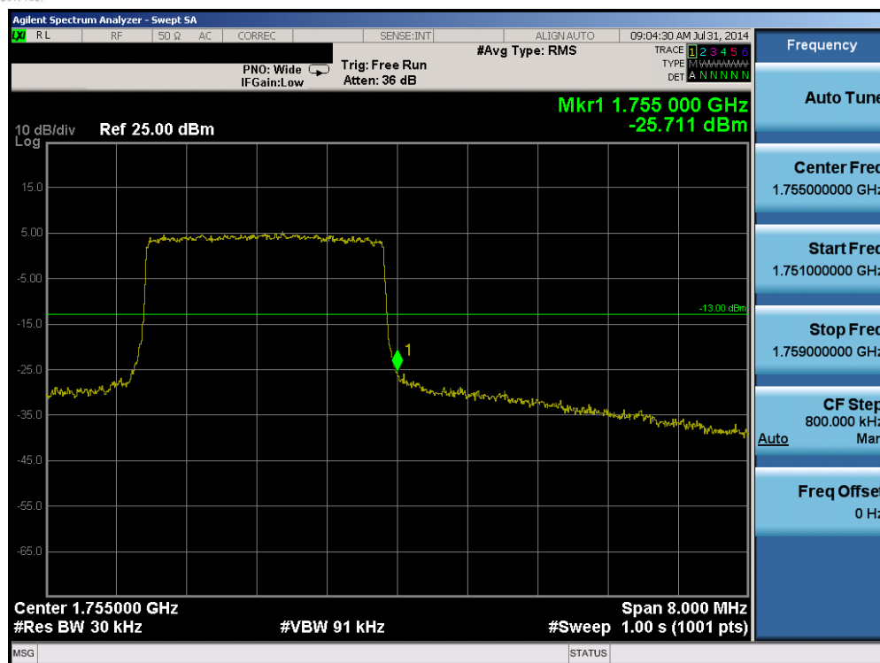
Plot 6-71. Upper Band Edge Plot (Band 4 – 3.0MHz QPSK – RB Size 15)
