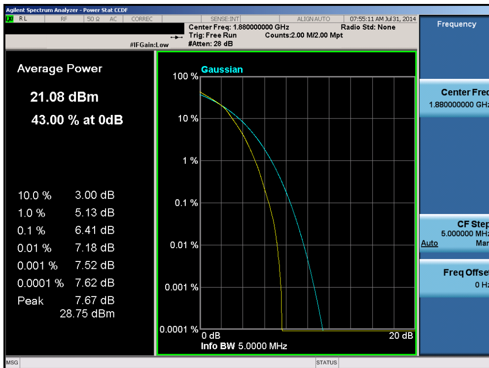
Plot 6-118. PAR Plot (Band 2 – 5.0MHz 16-QAM – RB Size 25)
