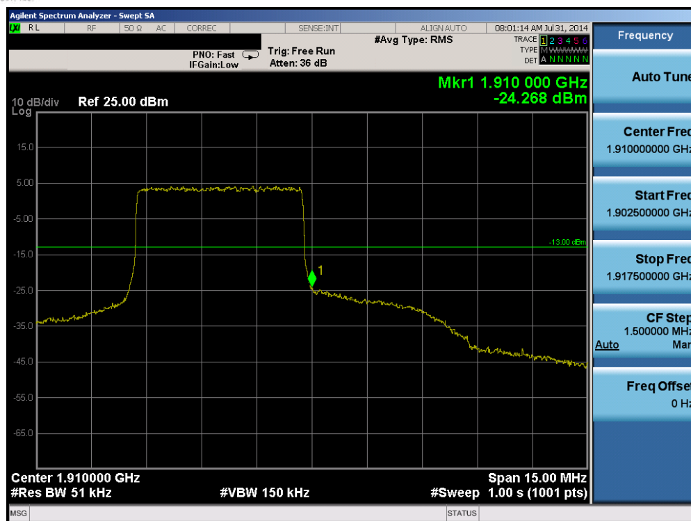
Plot 6-99. Upper Band Edge Plot (Band 2 – 5.0MHz QPSK – RB Size 25)
