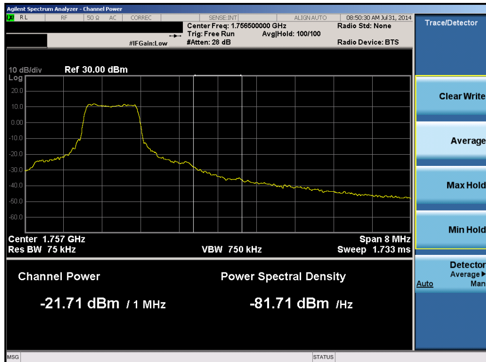
Plot 6-68. Upper Extended Band Edge Plot (Band 4 – 1.4MHz QPSK – RB Size 6)
