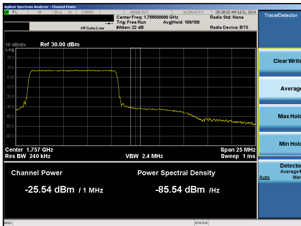
Plot 6-80. Upper Extended Band Edge Plot (Band 4 – 10.0MHz QPSK – RB Size 50)
