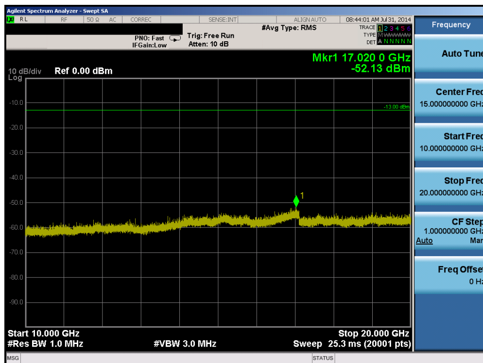
Plot 6-42. Conducted Spurious Plot (Band 4 – 1.4MHz QPSK – RB Size 1, RB Offset 0 – Mid Channel)
