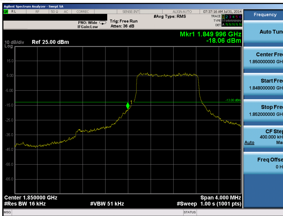
Plot 6-89. Lower Band Edge Plot (Band 2 – 1.4MHz QPSK – RB Size 6)
