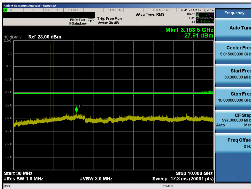
Plot 6-49. Conducted Spurious Plot (Band 2 – 1.4MHz QPSK – RB Size 1, RB Offset 0 – High Channel)
