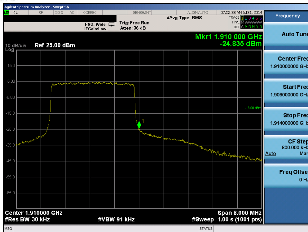
Plot 6-95. Upper Band Edge Plot (Band 2 – 3.0MHz QPSK – RB Size 15)
