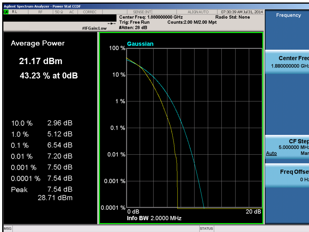
Plot 6-114. PAR Plot (Band 2 – 1.4MHz 16-QAM – RB Size 6)
