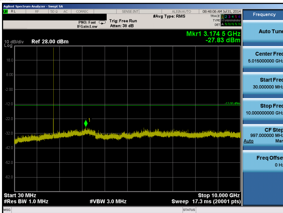
Plot 6-43. Conducted Spurious Plot (Band 4 – 1.4MHz QPSK – RB Size 1, RB Offset 0 – High Channel)
