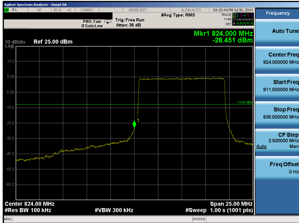
Plot 6-63. Lower Band Edge Plot (Band 5 – 10.0MHz QPSK – RB Size 50)
