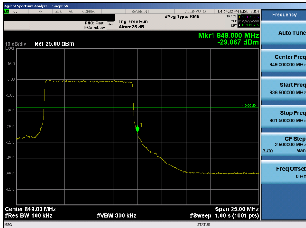
Plot 6-64. Upper Band Edge Plot (Band 5 – 10.0MHz QPSK – RB Size 50)
