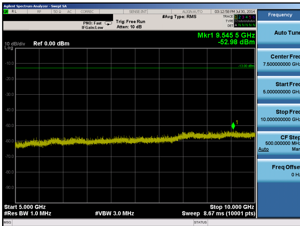
Plot 6-36. Conducted Spurious Plot (Band 5 – 1.4MHz QPSK – RB Size 1, RB Offset 0 – Mid Channel)
