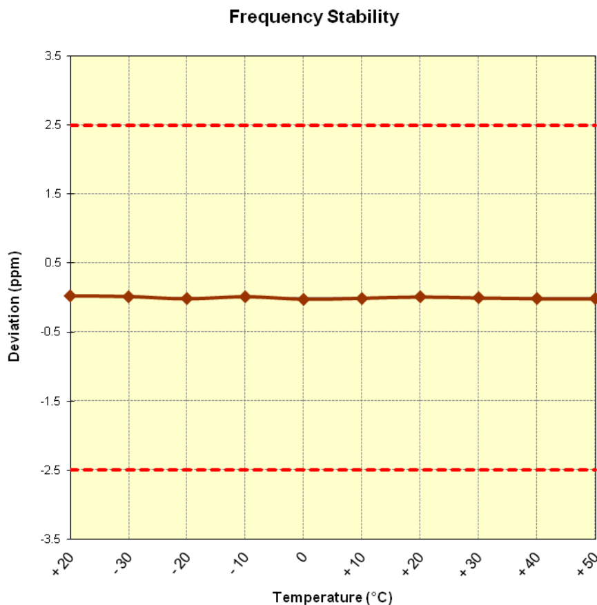
Figure 6-7. Frequency Stability Graph (Band 5)
