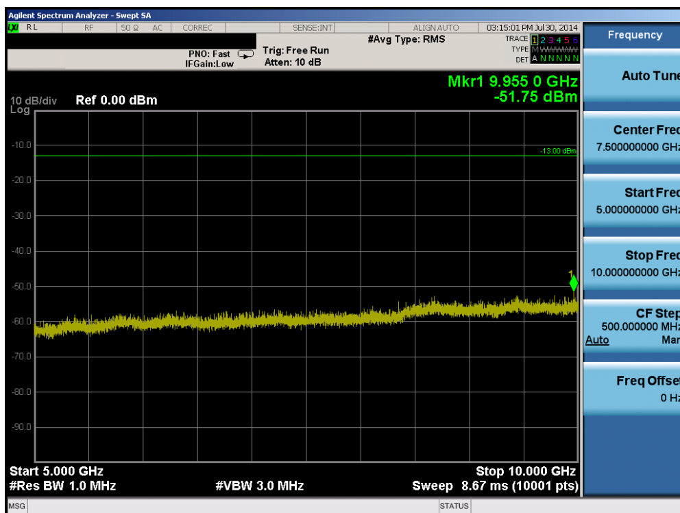
Plot 6-34. Conducted Spurious Plot (Band 5 – 1.4MHz QPSK – RB Size 1, RB Offset 0 – Low Channel)
