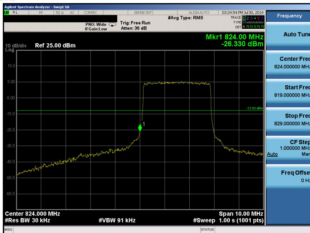
Plot 6-55. Lower Band Edge Plot (Band 5 – 3.0MHz QPSK – RB Size 15)
