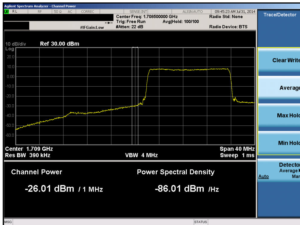
Plot 6-82. Lower Extended Band Edge Plot (Band 4 – 15.0MHz QPSK – RB Size 75)
