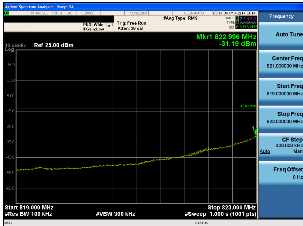
Plot 6-52. Lower Extended Band Edge Plot (Band 5 - 1.4MHz QPSK - RB Size 6)
