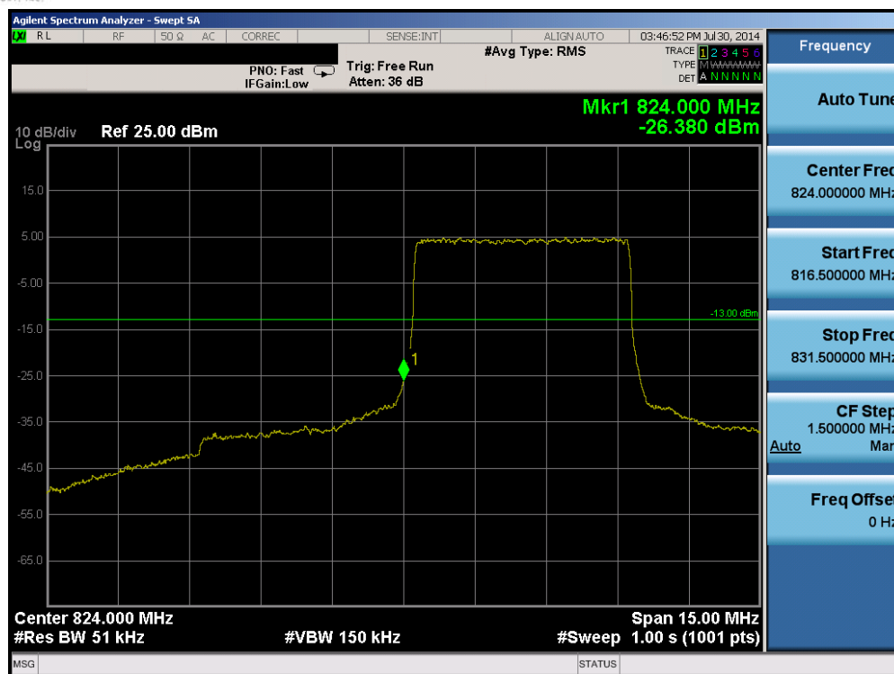
Plot 6-59. Lower Band Edge Plot (Band 5 - 5.0MHz QPSK - RB Size 25)
