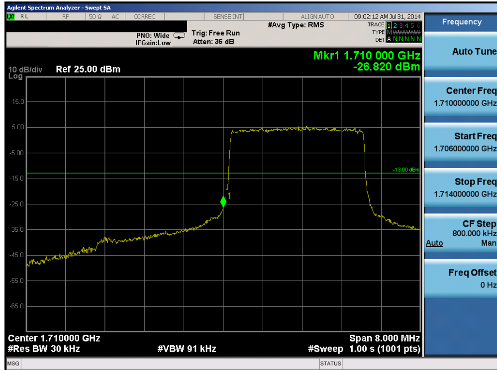
Plot 6-69. Lower Band Edge Plot (Band 4 – 3.0MHz QPSK – RB Size 15)
