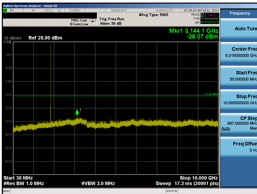
Plot 6-45. Conducted Spurious Plot (Band 2 – 1.4MHz QPSK – RB Size 1, RB Offset 0 – Low Channel)
