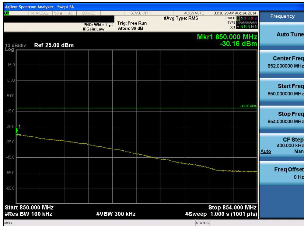
Plot 6-62. Upper Extended Band Edge Plot (Band 5 – 5.0MHz QPSK – RB Size 25)
