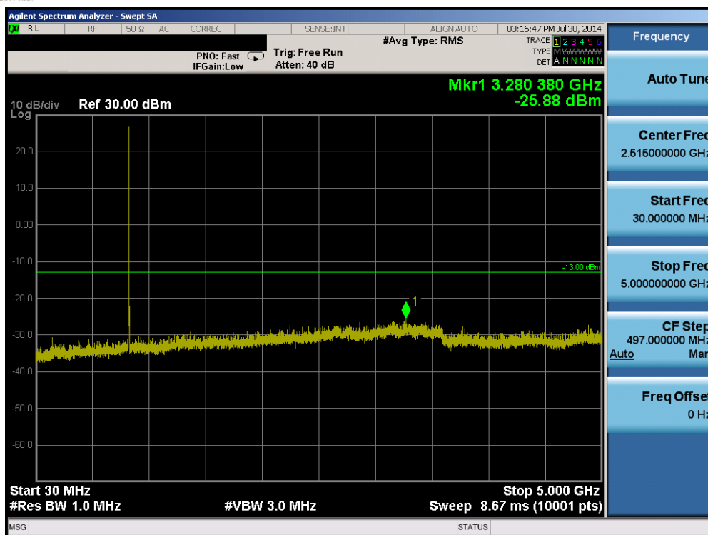
Plot 6-37. Conducted Spurious Plot (Band 5 – 1.4MHz QPSK – RB Size 1, RB Offset 0 – High Channel)
