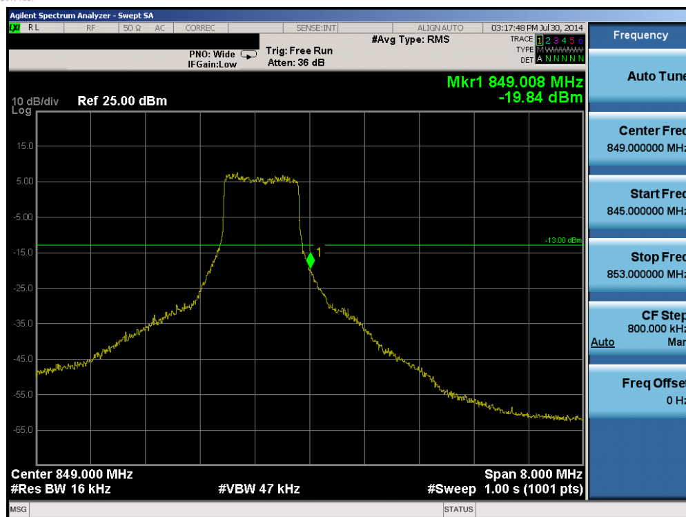
Plot 6-53. Upper Band Edge Plot (Band 5 – 1.4MHz QPSK – RB Size 6)
