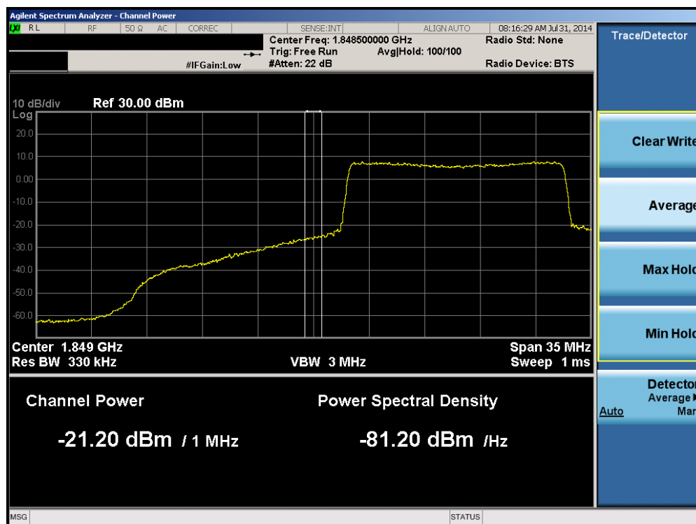
Plot 6-106. Lower Extended Band Edge Plot (Band 2 – 15.0MHz QPSK – RB Size 75)
