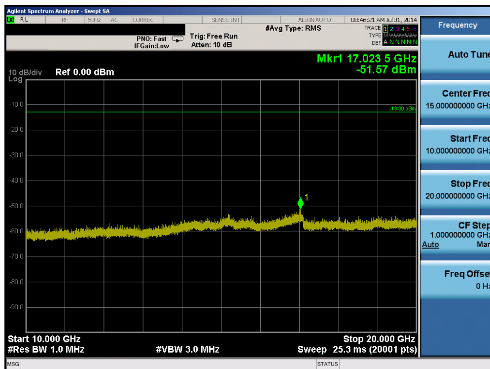
Plot 6-40. Conducted Spurious Plot (Band 4 – 1.4MHz QPSK – RB Size 1, RB Offset 0 – Low Channel)
