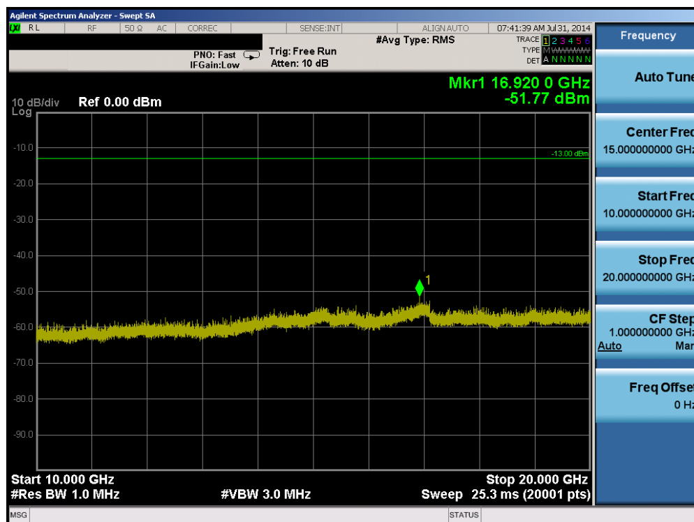
Plot 6-50. Conducted Spurious Plot (Band 2 – 1.4MHz QPSK – RB Size 1, RB Offset 0 – High Channel)
