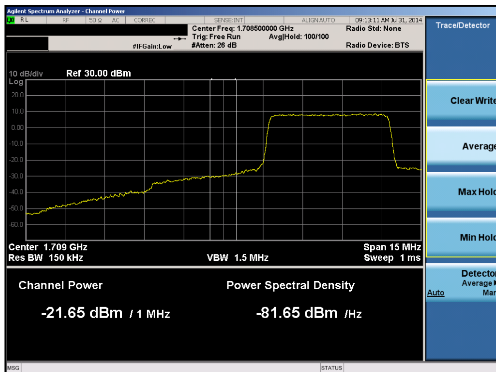
Plot 6-74. Lower Extended Band Edge Plot (Band 4 – 5.0MHz QPSK – RB Size 25)
