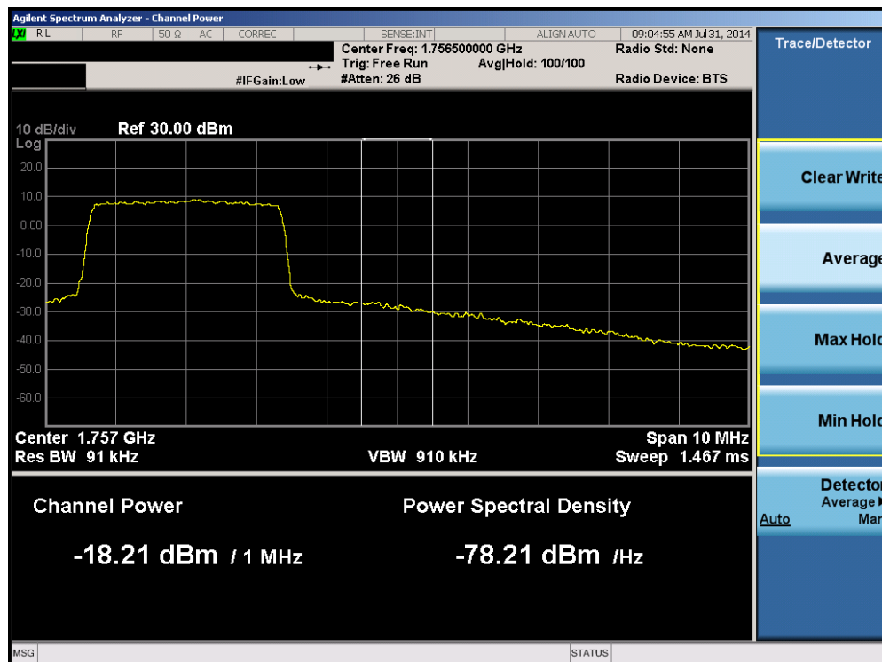
Plot 6-72. Upper Extended Band Edge Plot (Band 4 – 3.0MHz QPSK – RB Size 15)
