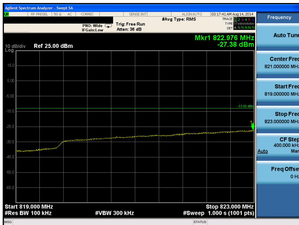
Plot 6-60. Lower Extended Band Edge Plot (Band 5 - 5.0MHz QPSK - RB Size 25)
