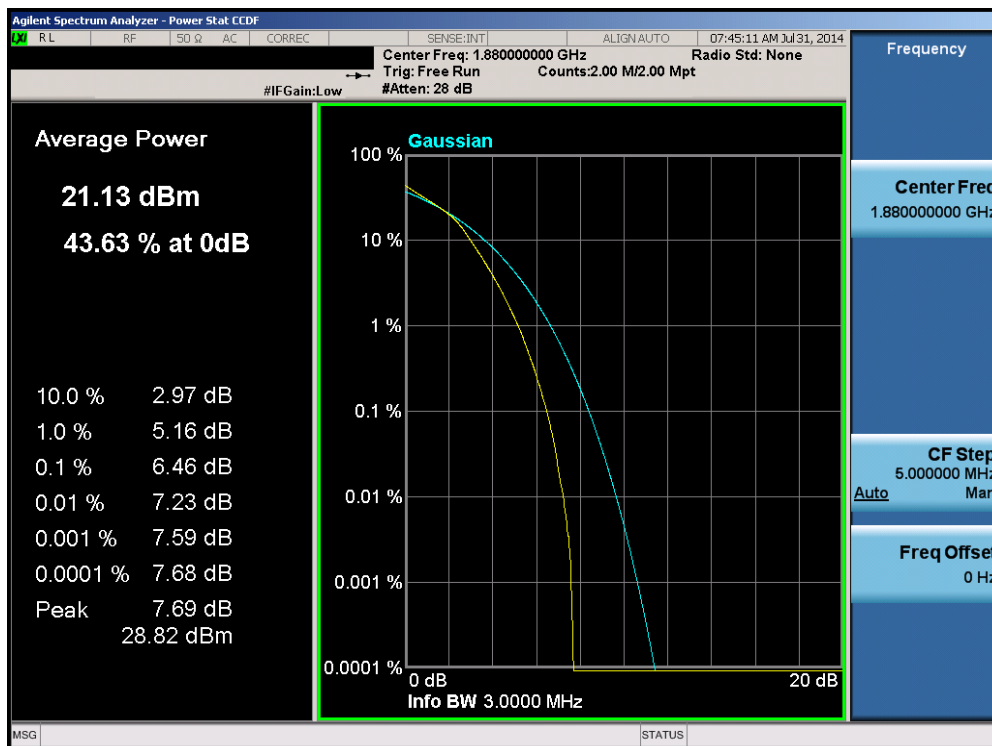
Plot 6-116. PAR Plot (Band 2 – 3.0MHz 16-QAM – RB Size 15)
