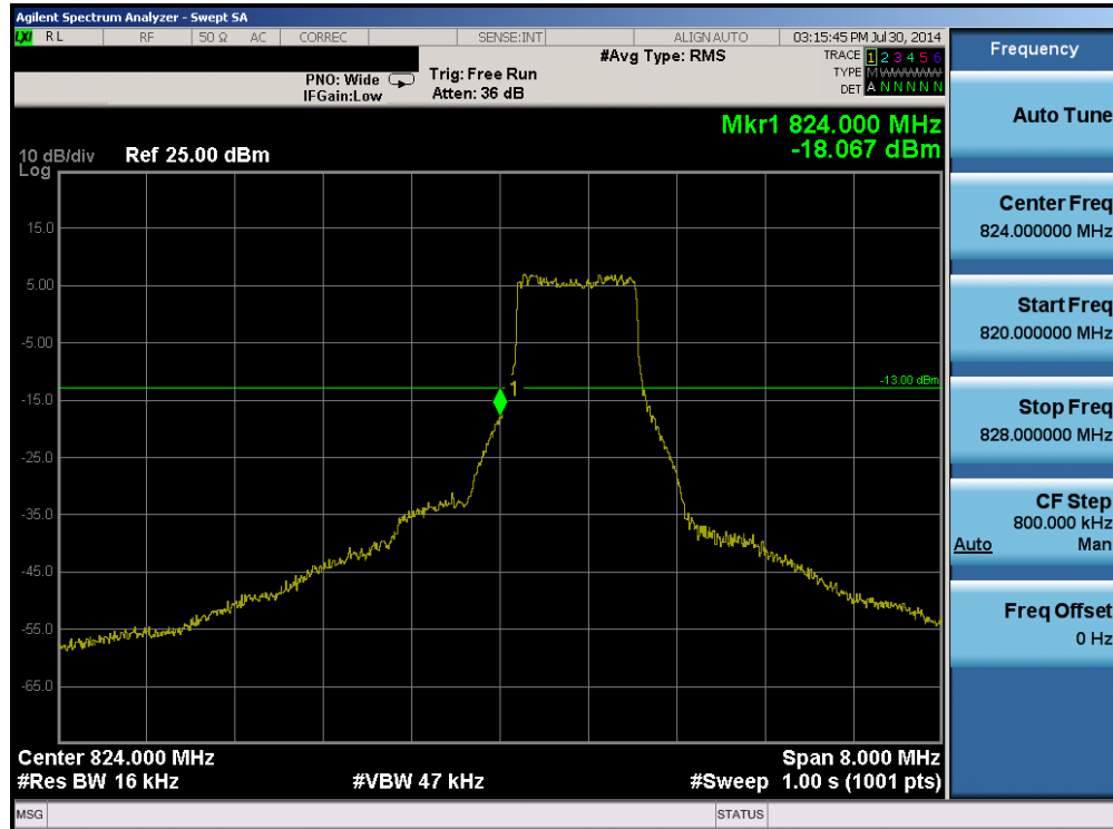
Plot 6-51. Lower Band Edge Plot (Band 5 - 1.4MHz QPSK - RB Size 6)
