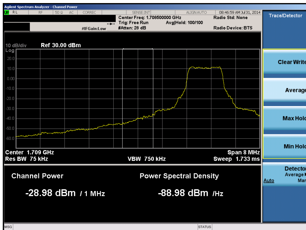
Plot 6-66. Lower Extended Band Edge Plot (Band 4 – 1.4MHz QPSK – RB Size 6)
