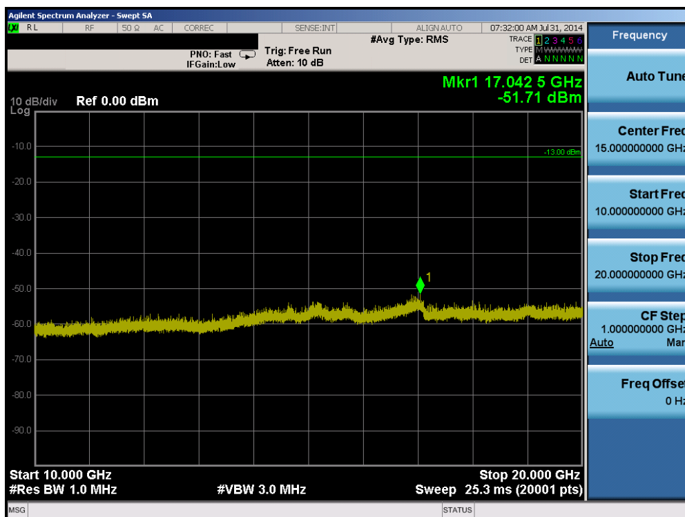
Plot 6-48. Conducted Spurious Plot (Band 2 – 1.4MHz QPSK – RB Size 1, RB Offset 0 – Mid Channel)
