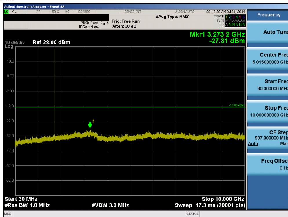
Plot 6-41. Conducted Spurious Plot (Band 4 – 1.4MHz QPSK – RB Size 1, RB Offset 0 – Mid Channel)
