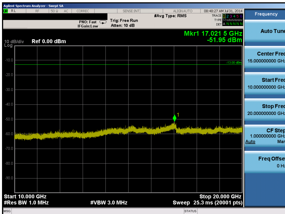
Plot 6-44. Conducted Spurious Plot (Band 4 – 1.4MHz QPSK – RB Size 1, RB Offset 0 – High Channel)
