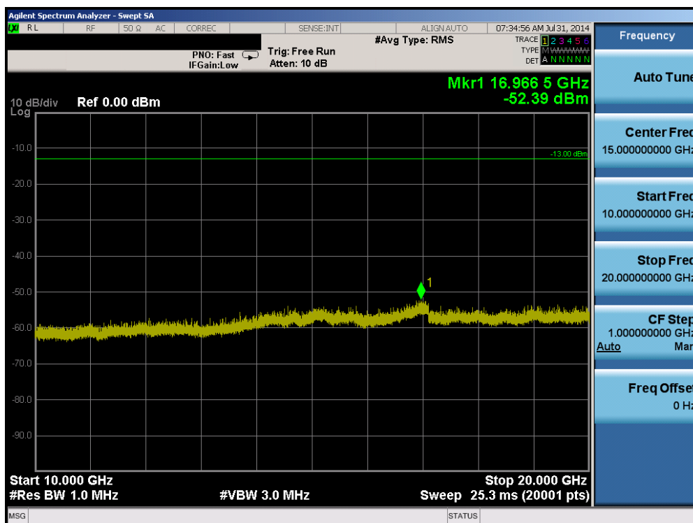
Plot 6-46. Conducted Spurious Plot (Band 2 – 1.4MHz QPSK – RB Size 1, RB Offset 0 – Low Channel)
