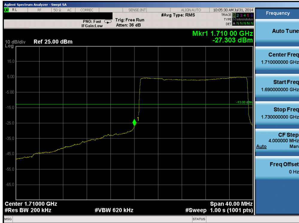
Plot 6-85. Lower Band Edge Plot (Band 4 – 20.0MHz QPSK – RB Size 100)
