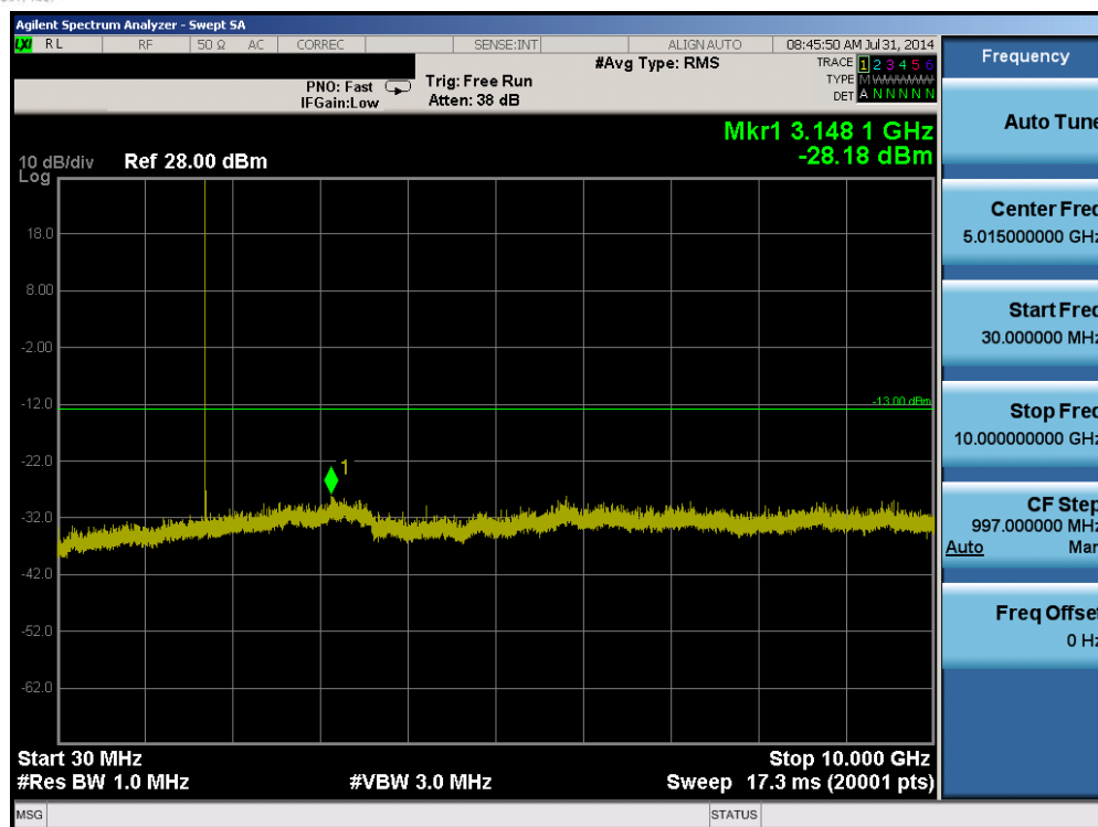
Plot 6-39. Conducted Spurious Plot (Band 4 – 1.4MHz QPSK – RB Size 1, RB Offset 0 – Low Channel)
