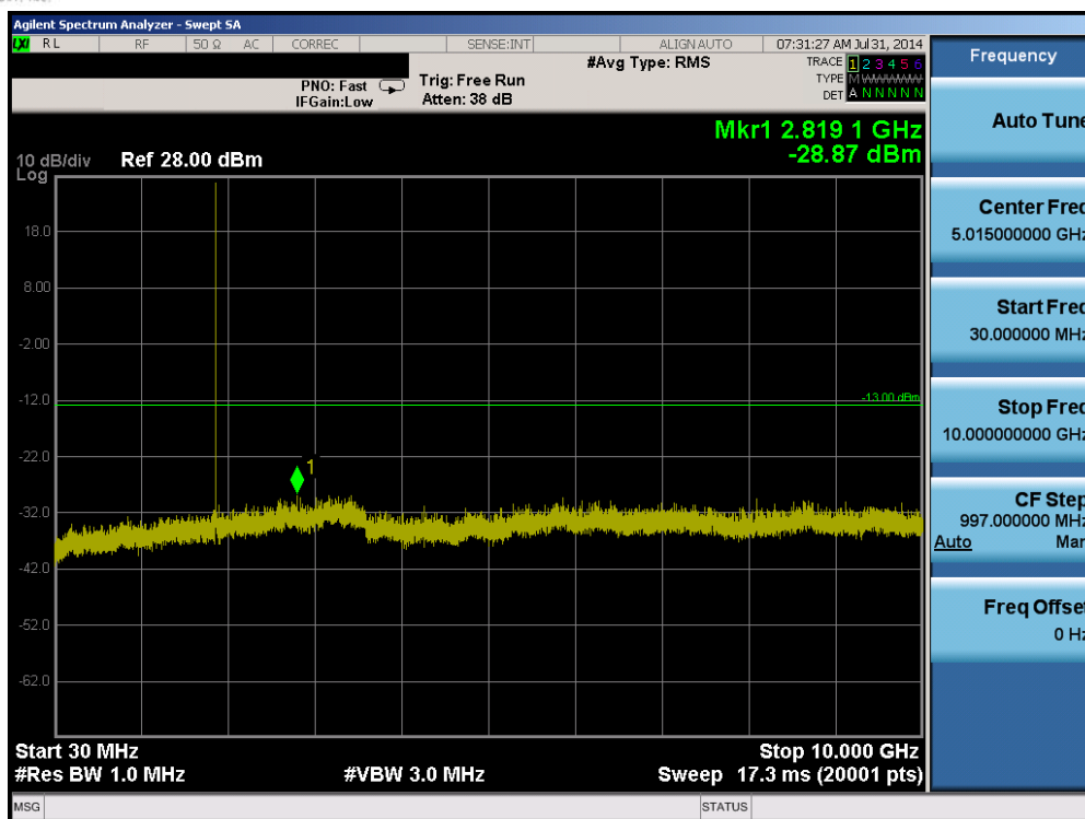
Plot 6-47. Conducted Spurious Plot (Band 2 – 1.4MHz QPSK – RB Size 1, RB Offset 0 – Mid Channel)
