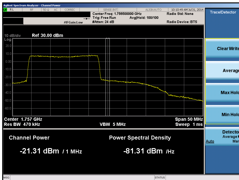
Plot 6-88. Upper Extended Band Edge Plot (Band 4 – 20.0MHz QPSK – RB Size 100)
