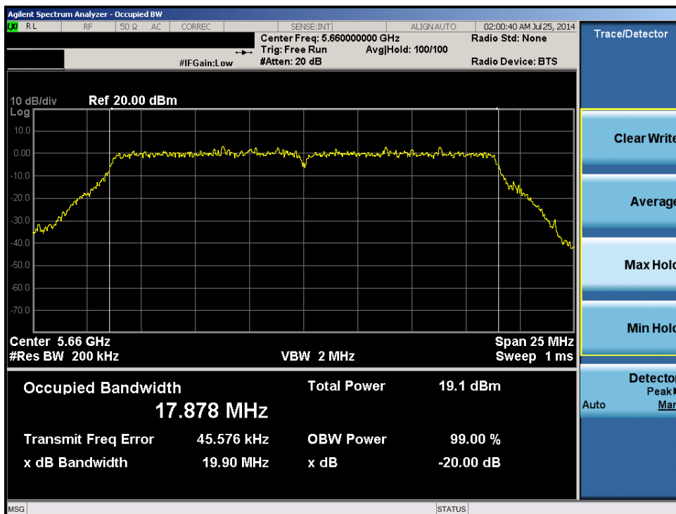
Plot 6-65. 20dB Bandwidth Plot (20MHz BW 802.11n (UNII Band 2C) – Ch. 132)
