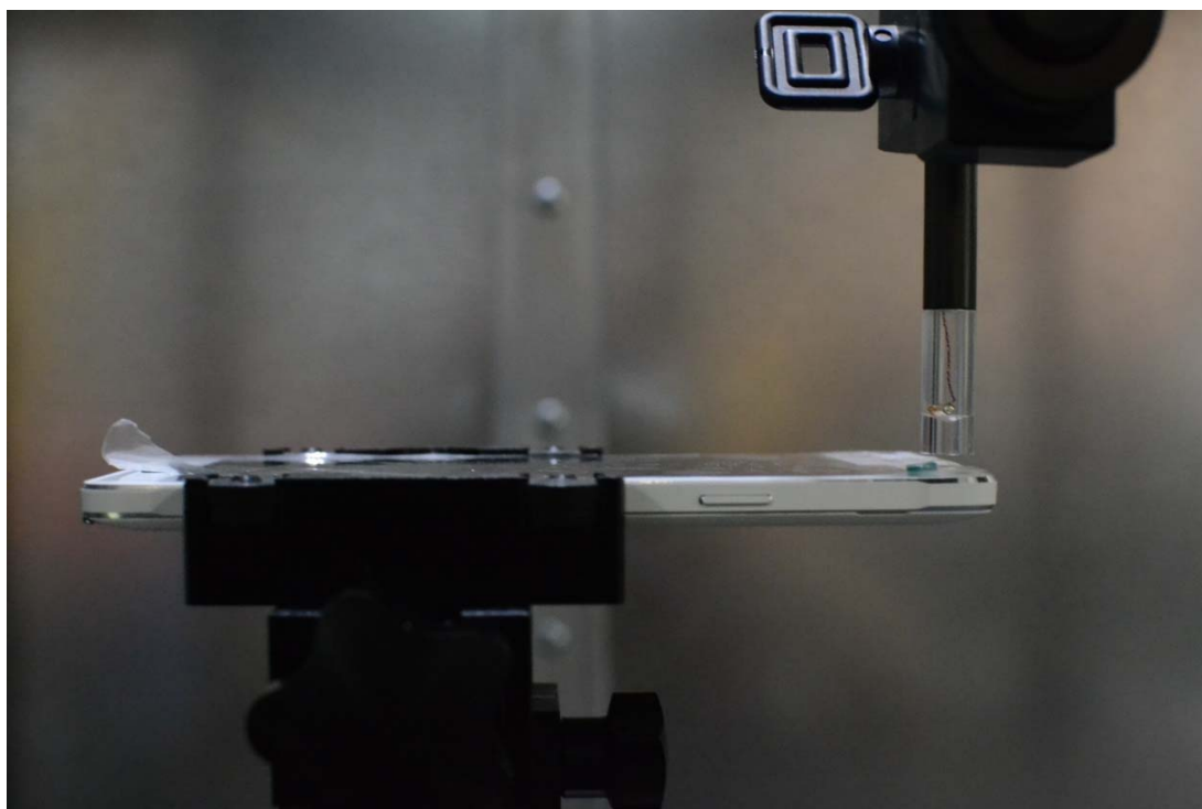
Figure 14-2 Test Setup for Wireless Device (Pictured with the Standard Battery Cover)
