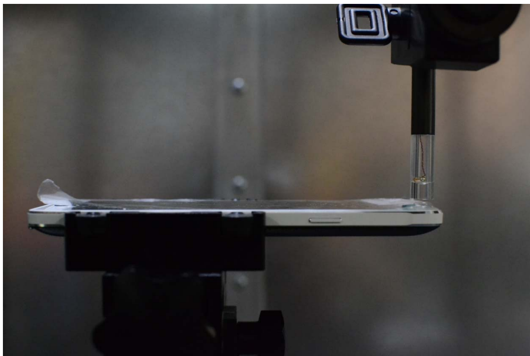
Figure 14-3 Test Setup for Wireless Device (Pictured with the Wireless Charging Cover Accessory)
