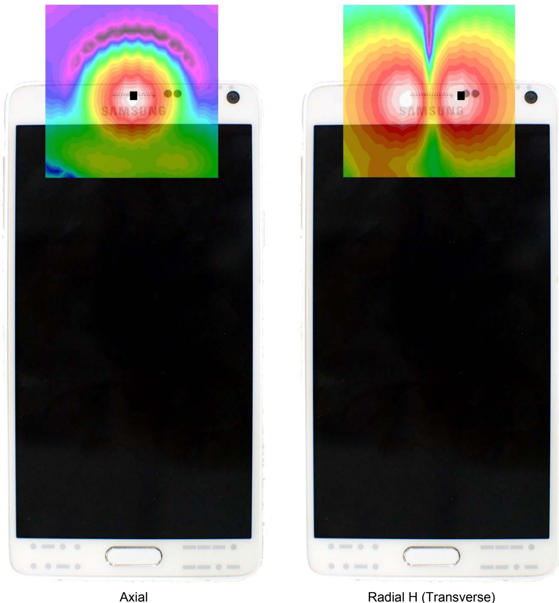
Figure 14-4 T-Coil Scan Overlay Magnetic Field Distributions
