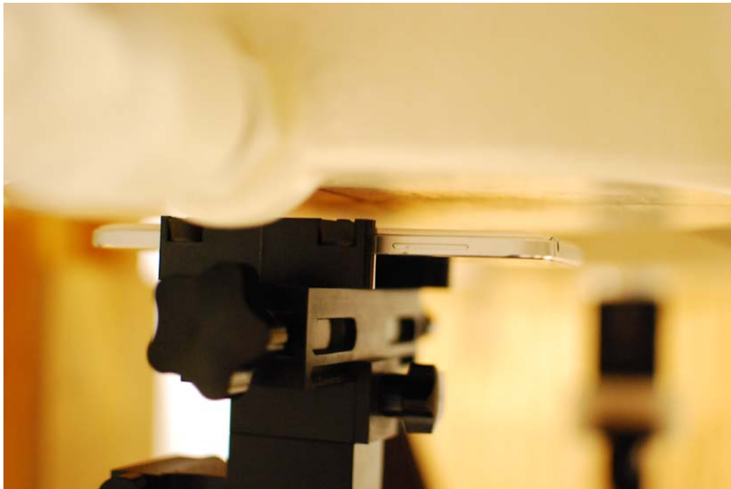
SAR Test Setup Photo 6: Back Side at 1.0 cm (Body-worn)
