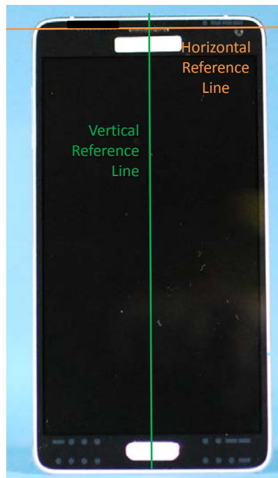
SAR Test Setup Photo 10: DUT Reference Lines
