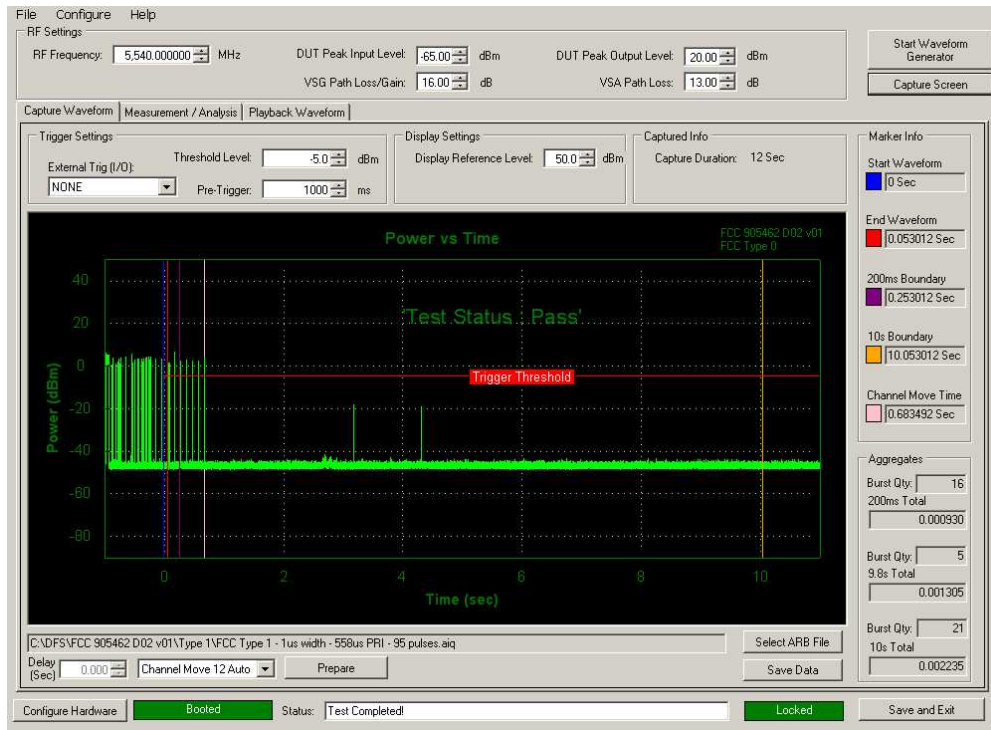
Figure 5-2. Band 2C Move Time and Aggregate Time
