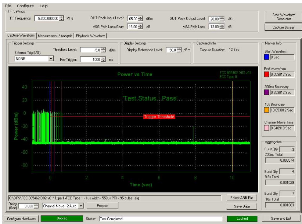
Figure 5-1. Band 2A Move Time and Aggregate Time
