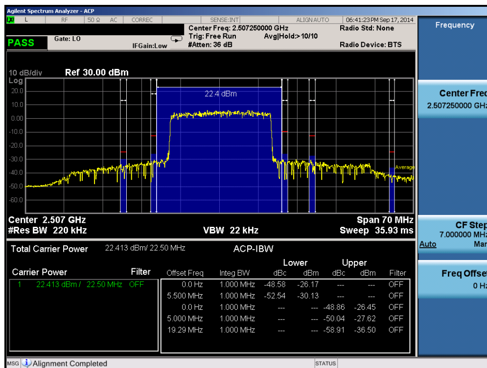
Plot 6-27. Lower ACP Plot (Band 41 – 20.0MHz QPSK – RB Size 100)
