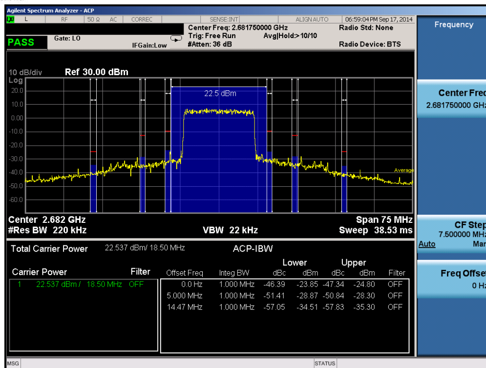
Plot 6-26. Upper ACP Plot (Band 41 – 15.0MHz QPSK – RB Size 75)
