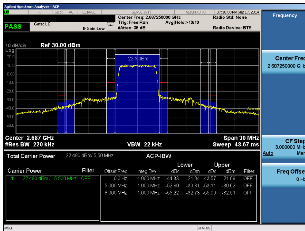
Plot 6-20. Upper ACP Plot (Band 41 – 5.0MHz QPSK – RB Size 25)
