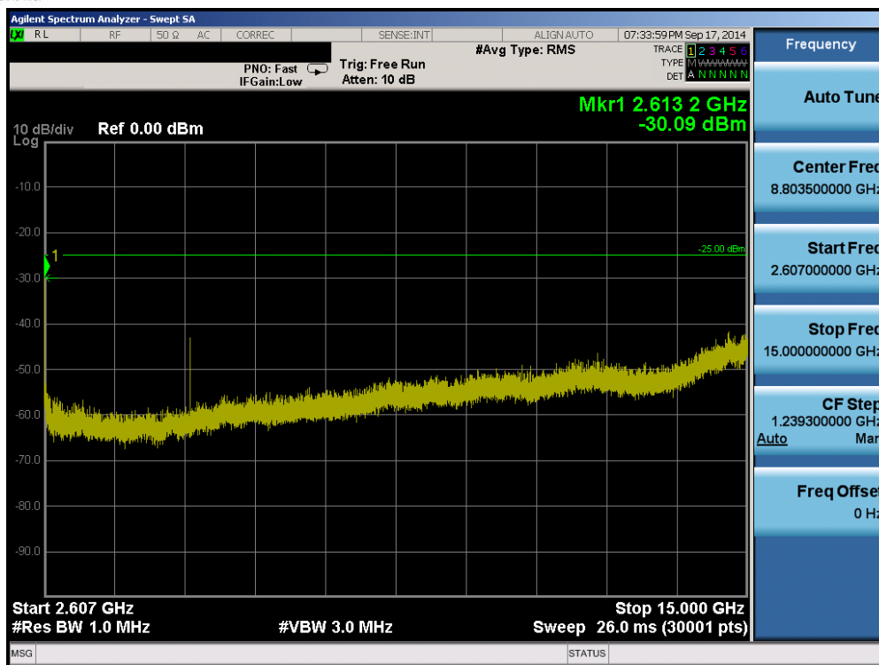
Plot 6-13. Conducted Spurious Plot (Band 41 – 15.0MHz QPSK – RB Size 1, RB Offset 0 – Mid Channel)
