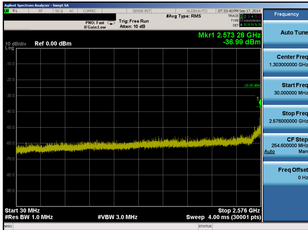
Plot 6-12. Conducted Spurious Plot (Band 41 – 15.0MHz QPSK – RB Size 1, RB Offset 0 – Mid Channel)
