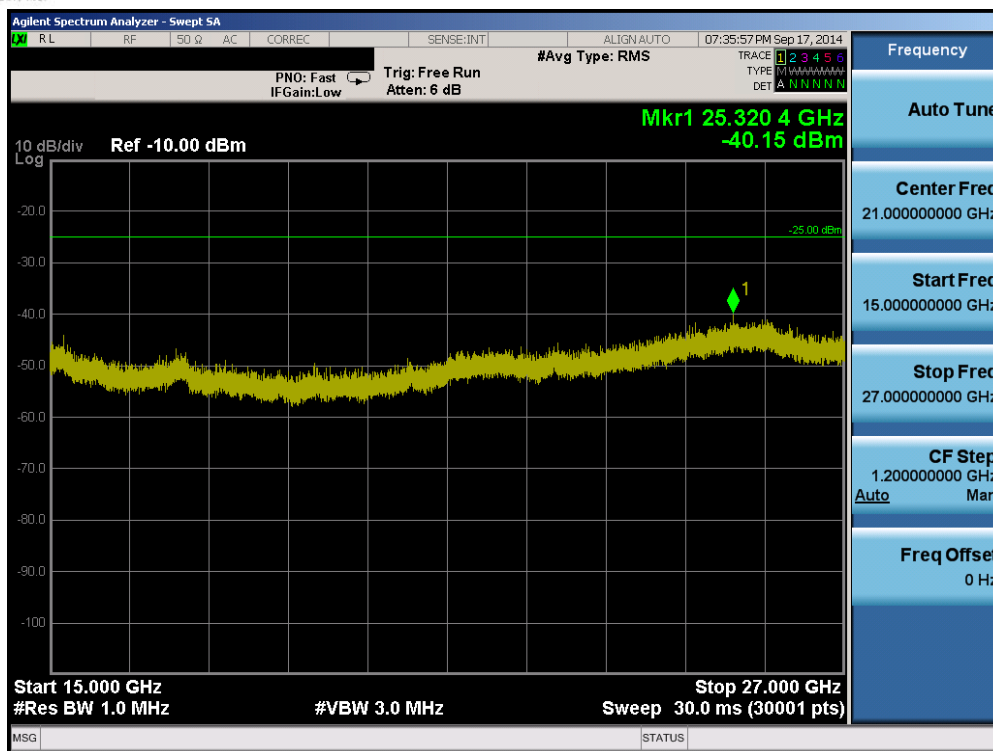
Plot 6-17. Conducted Spurious Plot (Band 41 – 15.0MHz QPSK – RB Size 1, RB Offset 0 – High Channel)
