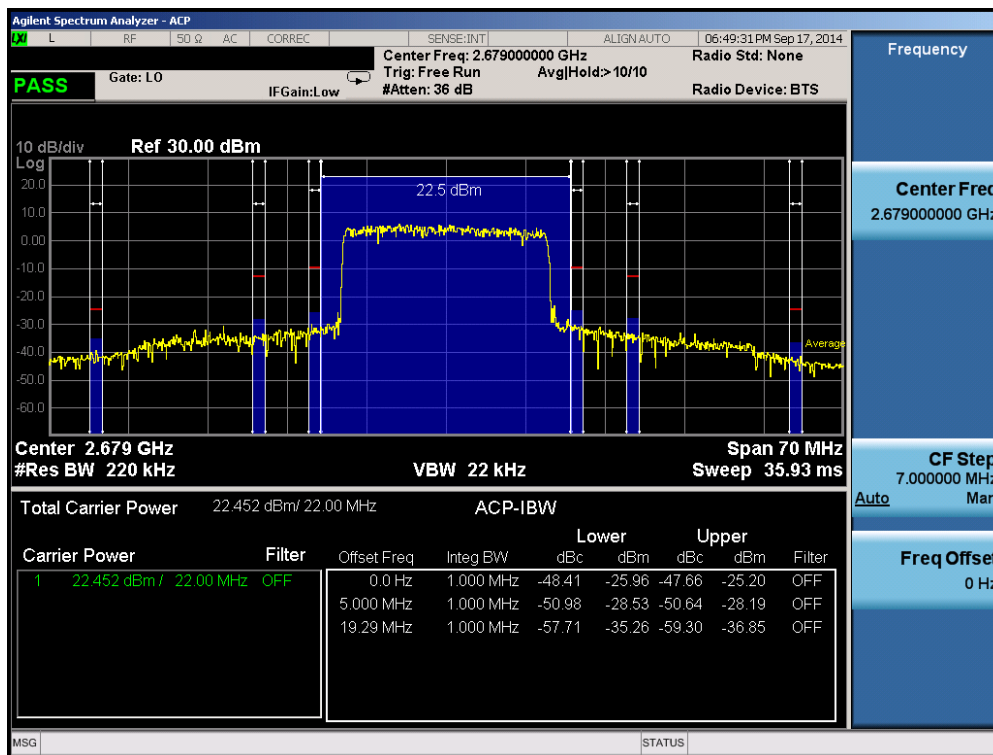
Plot 6-29. Upper ACP Plot (Band 41 – 20.0MHz QPSK – RB Size 100)
