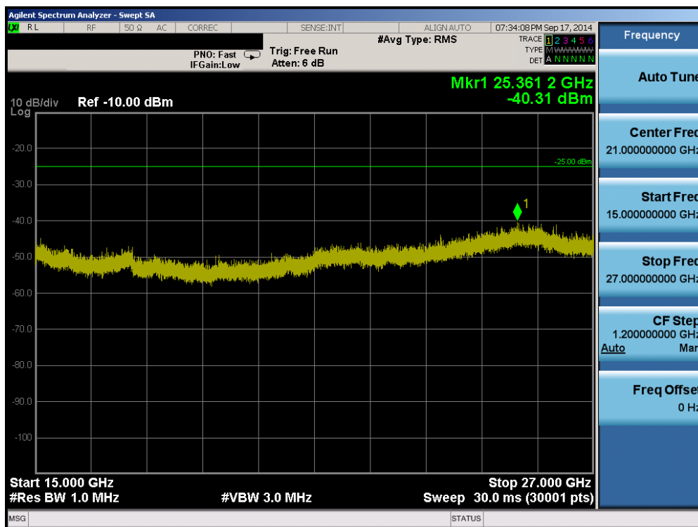
Plot 6-14. Conducted Spurious Plot (Band 41 – 15.0MHz QPSK – RB Size 1, RB Offset 0 – Mid Channel)
