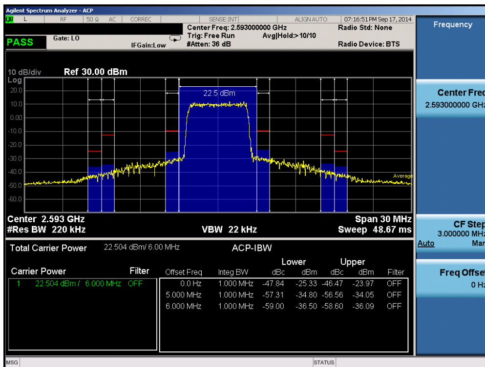
Plot 6-19. Mid ACP Plot (Band 41 – 5.0MHz QPSK – RB Size 25)
