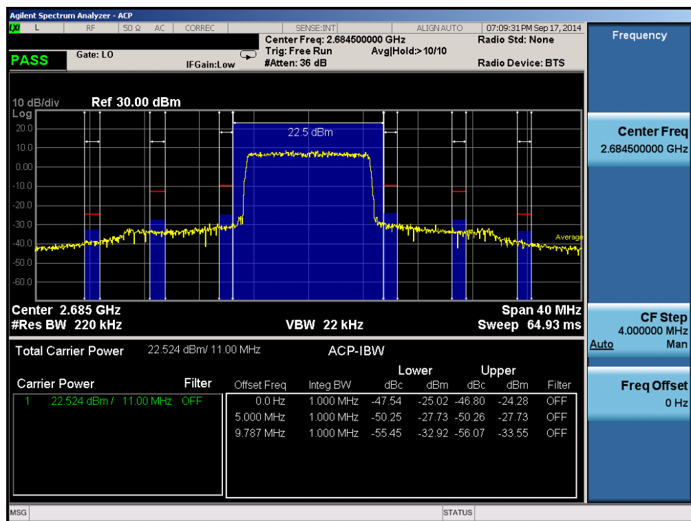
Plot 6-23. Upper ACP Plot (Band 41 – 10.0MHz QPSK – RB Size 50)
