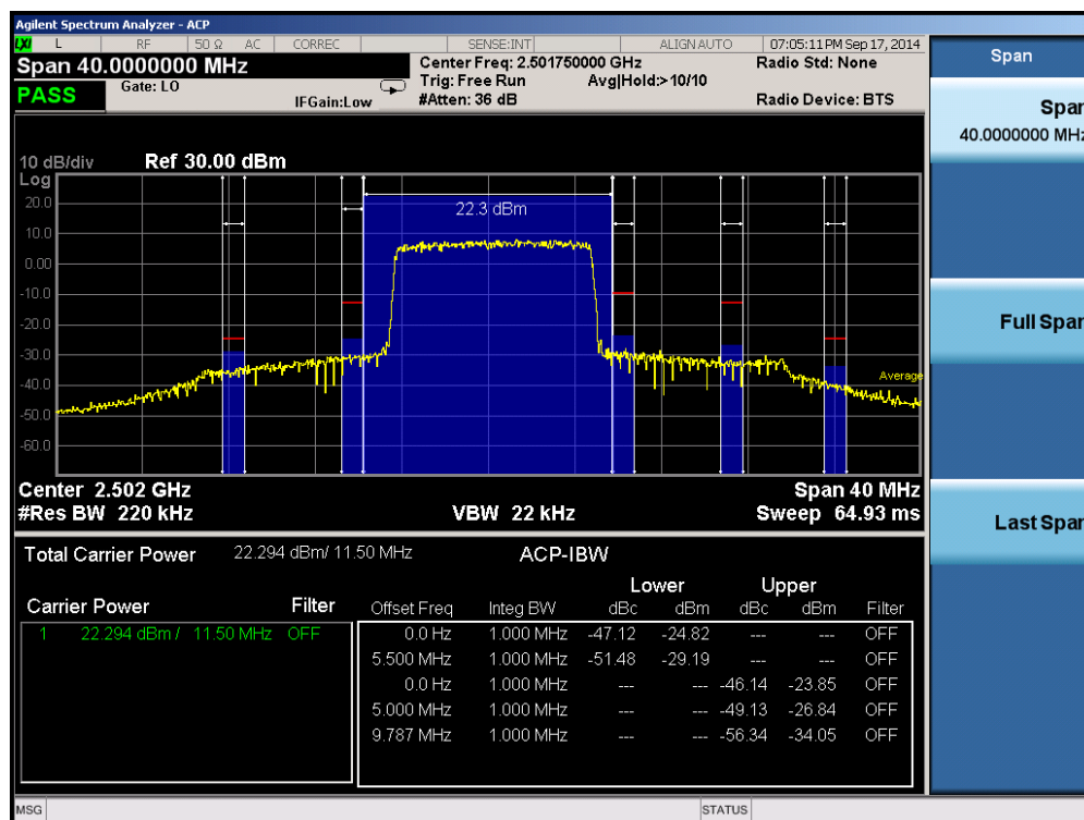
Plot 6-21. Lower ACP Plot (Band 41 – 10.0MHz QPSK – RB Size 50)
