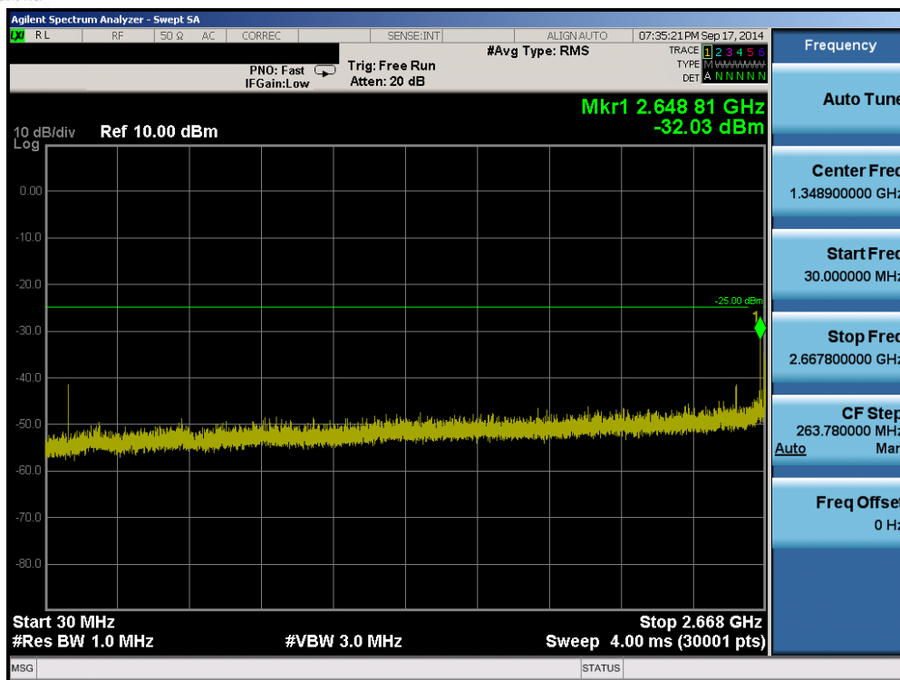
Plot 6-15. Conducted Spurious Plot (Band 41 – 15.0MHz QPSK – RB Size 1, RB Offset 0 – High Channel)
