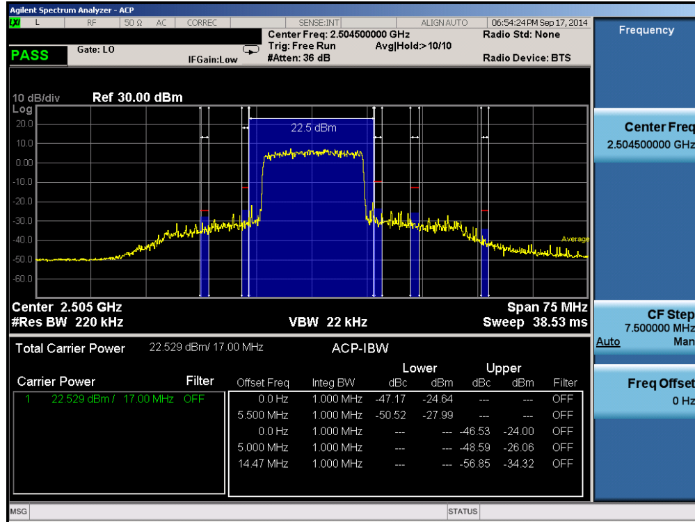
Plot 6-24. Lower ACP Plot (Band 41 – 15.0MHz QPSK – RB Size 75)
