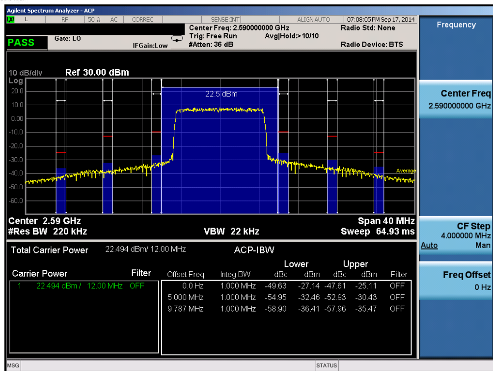
Plot 6-22. Mid ACP Plot (Band 41 – 10.0MHz QPSK – RB Size 50)
