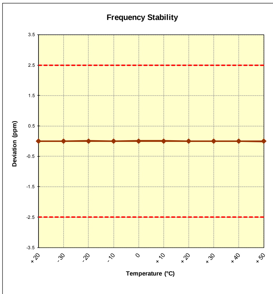
Figure 6-6. Frequency Stability Graph (Band 41)
