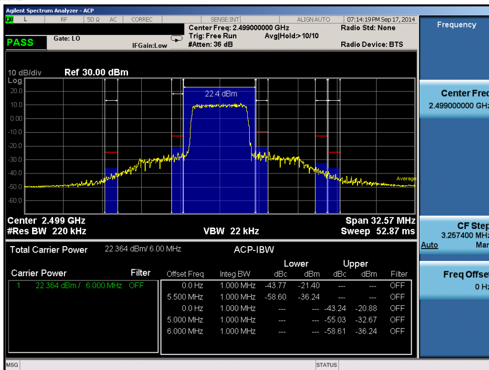
Plot 6-18. Lower ACP Plot (Band 41 – 5.0MHz QPSK – RB Size 25)
