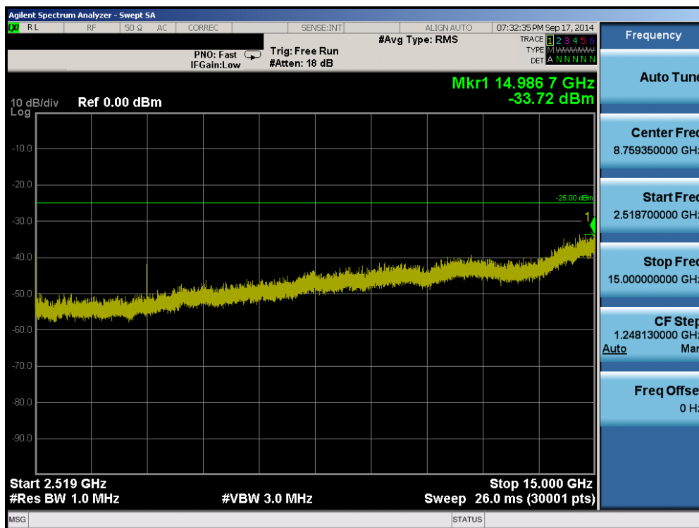
Plot 6-10. Conducted Spurious Plot (Band 41 – 15.0MHz QPSK – RB Size 1, RB Offset 0 – Low Channel)
