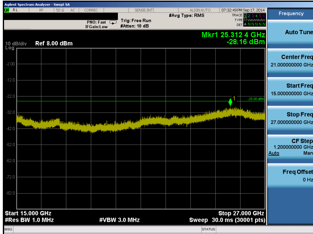
Plot 6-11. Conducted Spurious Plot (Band 41 – 15.0MHz QPSK – RB Size 1, RB Offset 0 – Low Channel)
