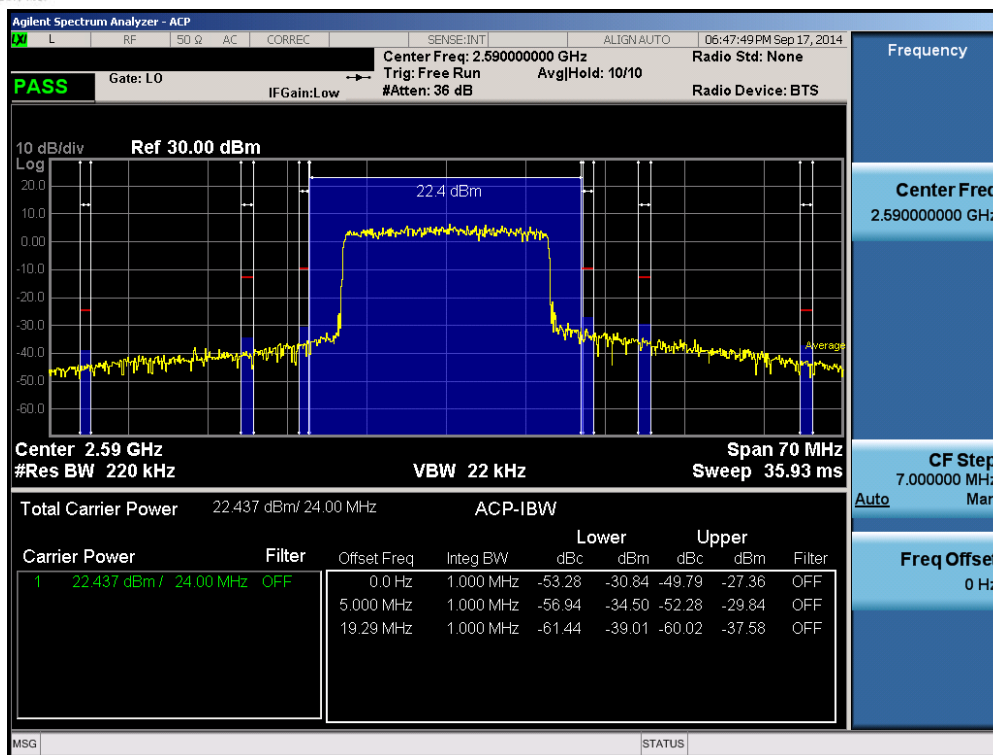
Plot 6-28. Mid ACP Plot (Band 41 – 20.0MHz QPSK – RB Size 100)
