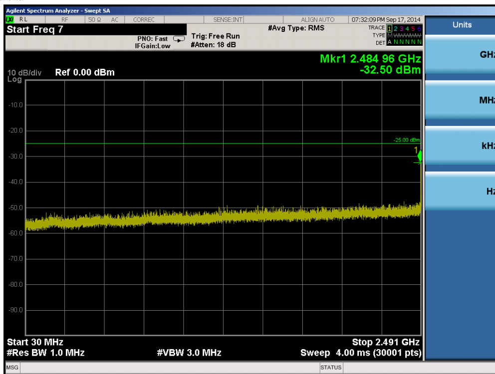
Plot 6-9. Conducted Spurious Plot (Band 41 – 15.0MHz QPSK – RB Size 1, RB Offset 0 – Low Channel)
