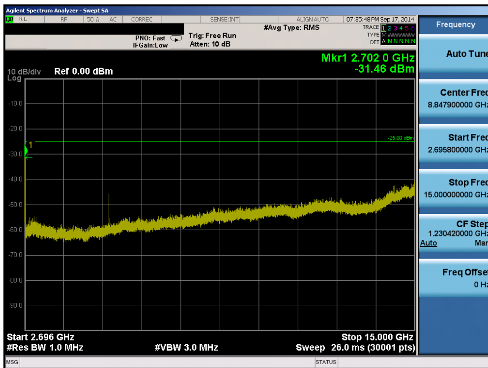
Plot 6-16. Conducted Spurious Plot (Band 41 – 15.0MHz QPSK – RB Size 1, RB Offset 0 – High Channel)
