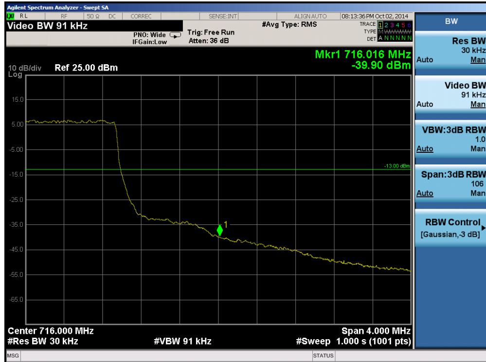
Plot 6-79. Upper Band Edge Plot (Band 12 – 1.4MHz QPSK – RB Size 1)
